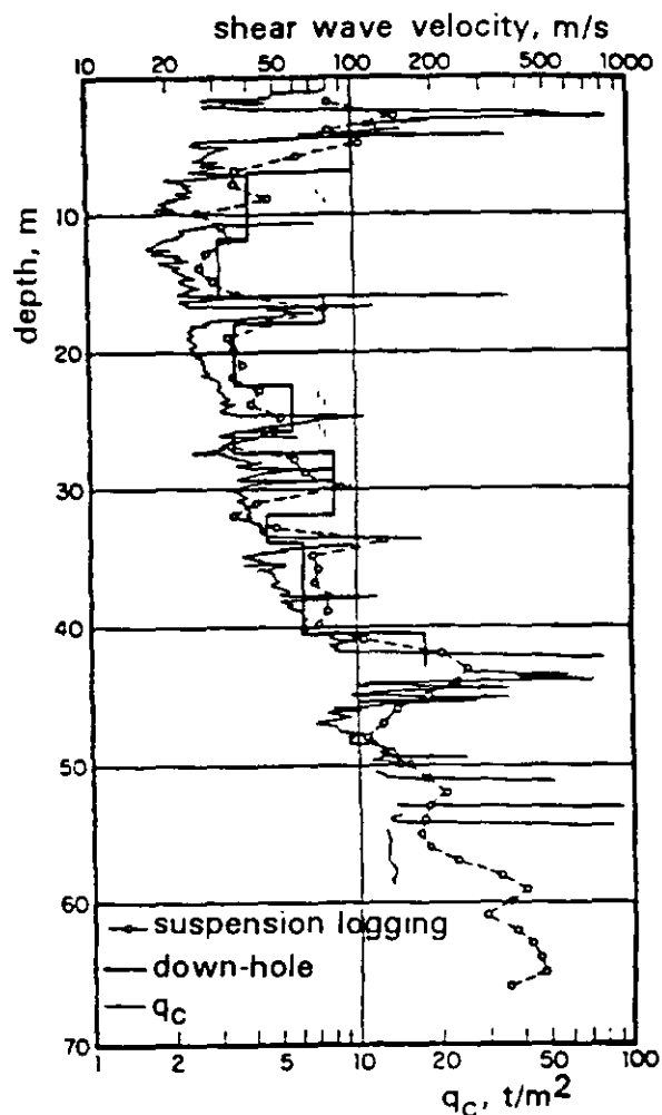
Fig 2 CPT sounding and shear wave velocity profiles for a site in the former Xochimilco-Chalco lake
