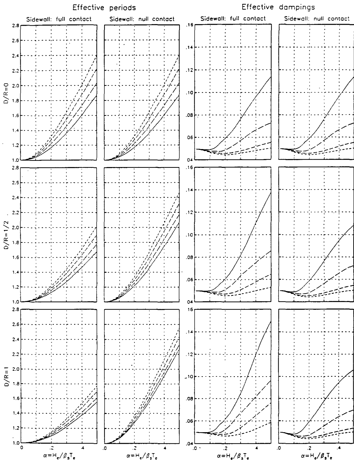
Fig. 3d Effective periods \bar{T}_e/T_e and dampings \bar{\zeta}_e of soil-structure systems for \nu_s = 0.45 and H_s/R = 10 ; curves correspond to H_e/R = 2 (solid line), 3, 4 and 5 (smallest dashed line)
