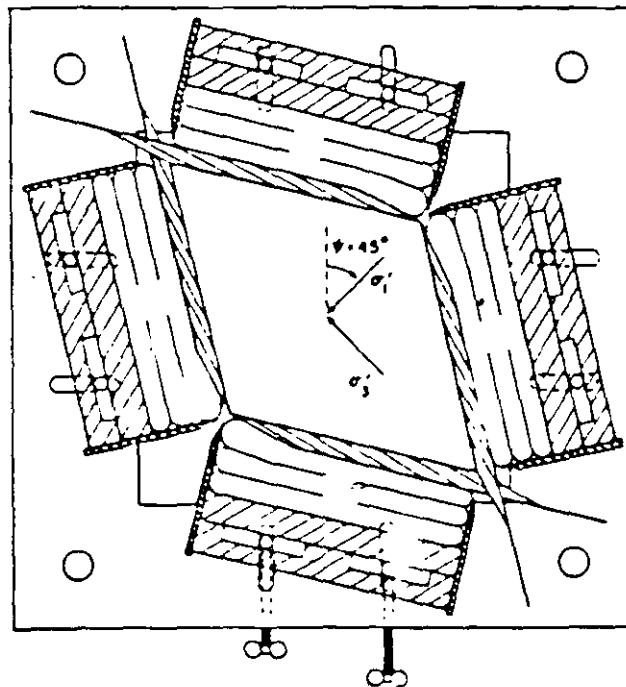
FIGURE 6 Stress condition and principal directions rotations in the DSC cell. After Arthur (1932).
