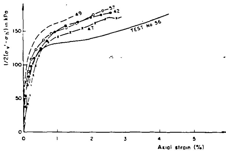
FIG. 20.B HRS tested at different strain rates Stress-strain curves (OVANDOCY HIGHT)
