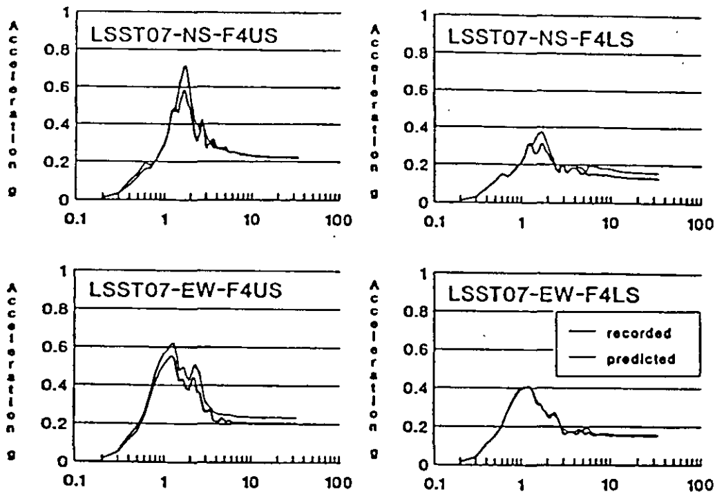
Figure 3. Predicted and recorded 5% damped response spectra, event LSST07- Soil-Spring method
