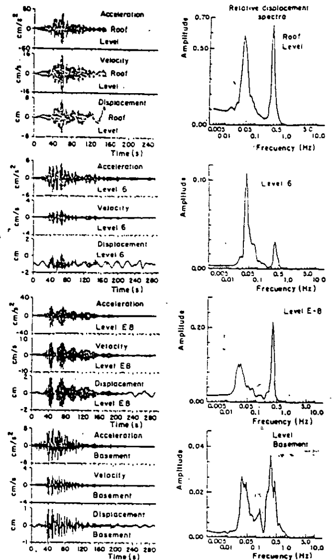
Figure 5. Torsional relative time series and relative displacement spectra obtained on May 30 th, 1990 earthquake
