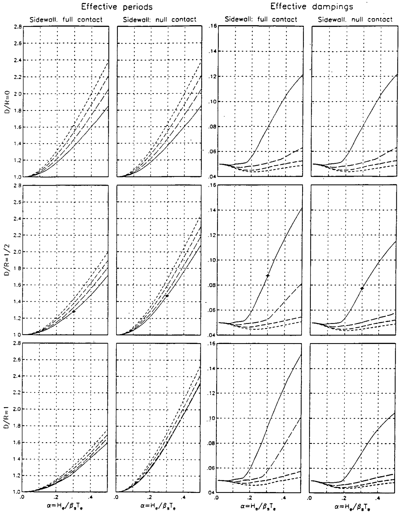
Fig. 3c Effective periods \bar{T}_e/T_e and dampings \bar{\zeta}_e of soil-structure systems for \nu_s = 0.45 and H_e/R = 6 ; curves correspond to H_e/R = 2 (solid line), 3, 4 and 5 (smallest dashed line)
