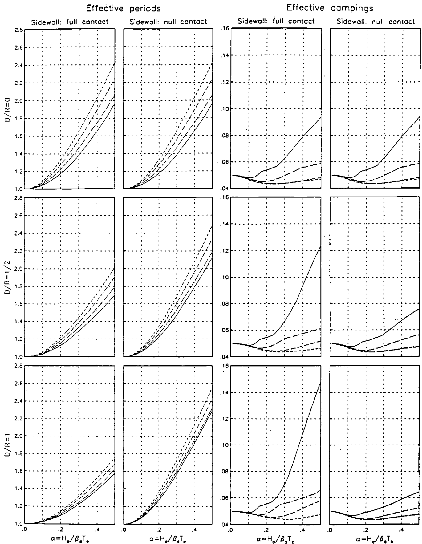
Fig. 3b Effective periods \bar{T}/T_e and dampings \bar{\zeta} of soil-structure systems for \nu_s = 0.45 and H_e/R = 4 ; curves correspond to H_e/R = 2 (solid line), 3, 4 and 5 (smallest dashed line)
