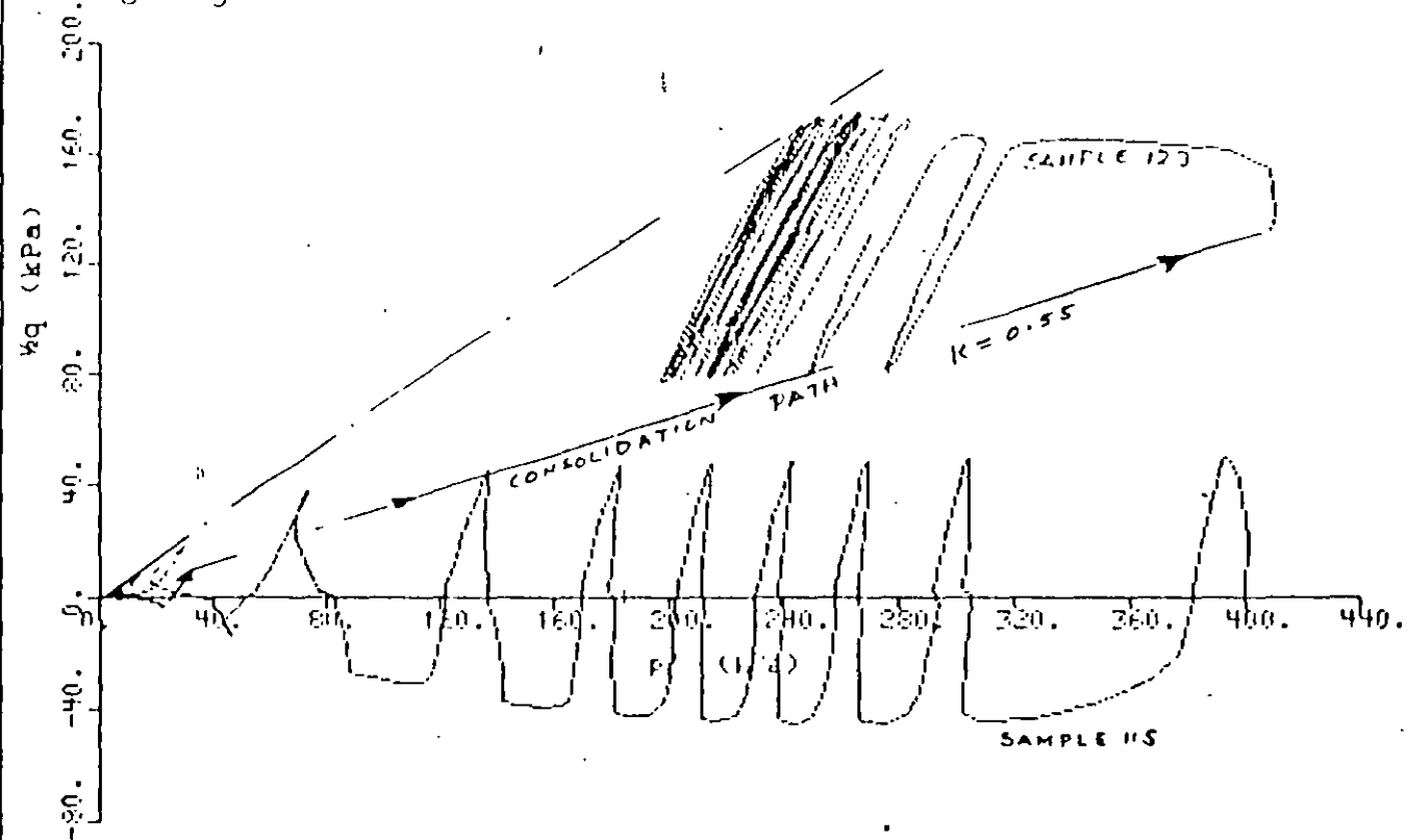
Fig. 9 NORMALLY CONSOLIDATED SAMPLES WITH DIFFERENT STRESS HISTORIES
