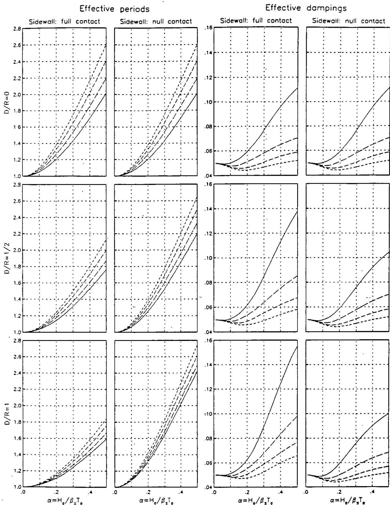
Fig. 2d Effective periods \bar{T}_e/T_e and dampings \bar{\zeta}_e of soil-structure systems for \nu_r = 1/3 and H_s/R=10 ; curves correspond to H_e/R=2 (solid line), 3, 4 and 5 (smallest dashed line) 17
