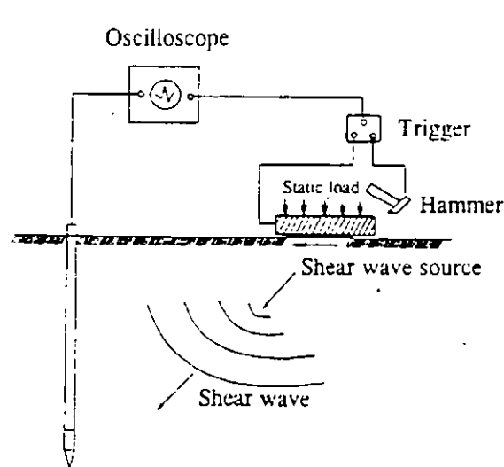
Fig 1 Seismic cone penetrometer (after Robertson et al, 1986)
