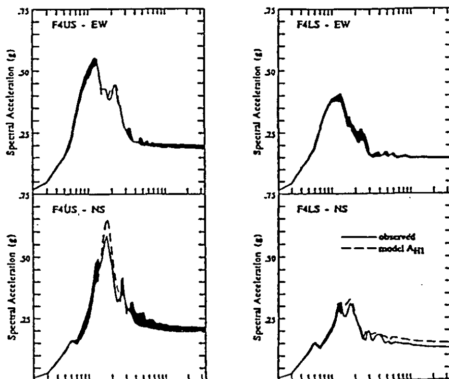
Figure 6. Predicted and recorded 5% damped response spectra for Model A_{HII} , event LSST07-CLASSI method, Luco/Wong
