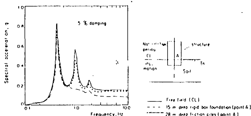
Fig. III-4.16: Effect of foundation type on floor response spectra
