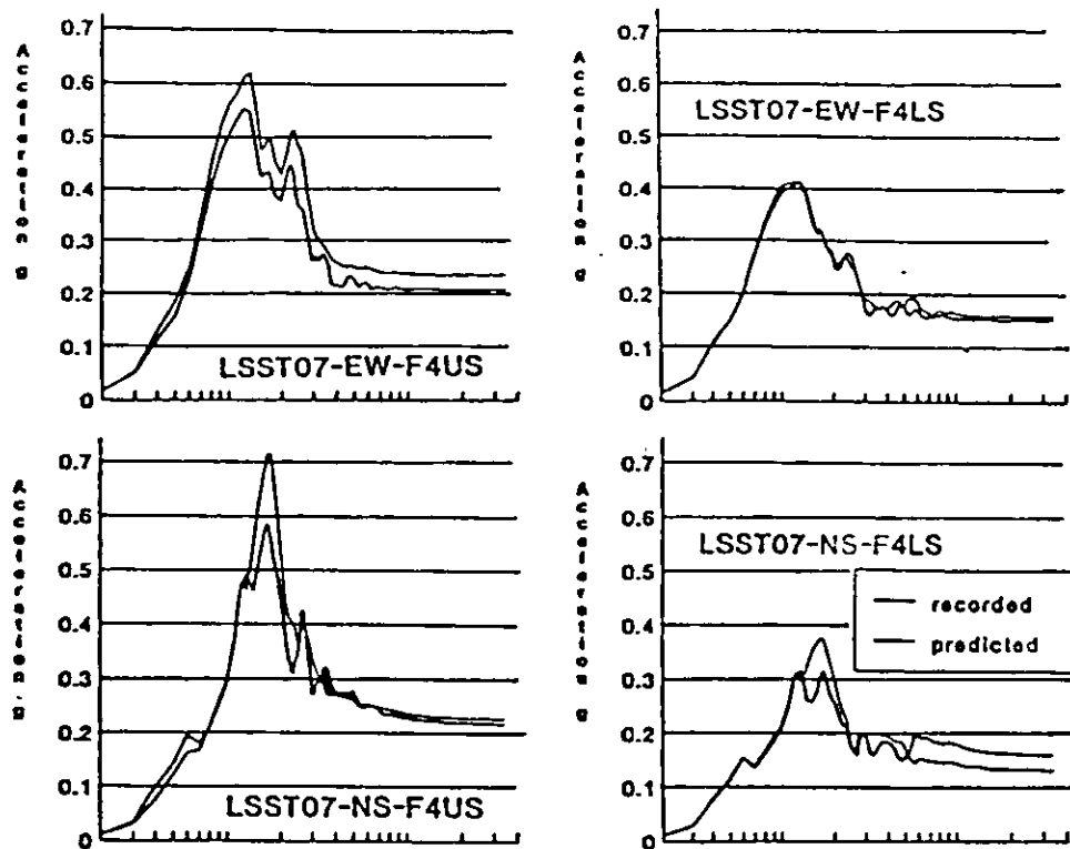
Figure 5. Predicted and recorded 5% damped response spectra, event LSST07-Soil-Spring method
