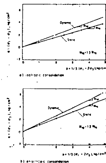
Fig. III-4.9: Failure envelopes for Mexico City clay
