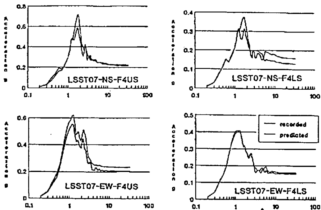
Figure 7. Predicted and recorded 5% damped response spectra, event LSST07-Soil-Spring method
