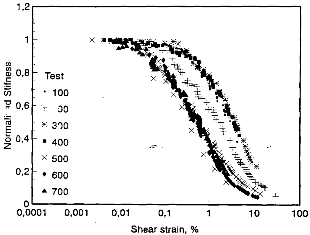
Fig 7 Normalized moduli ( G/G_{max} ) as a function of strain
