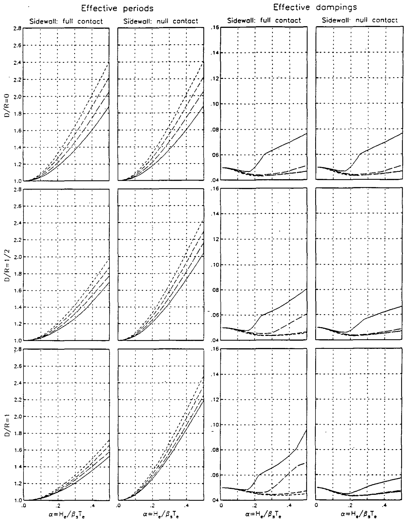
Fig. 3a Effective periods \bar{T}_e/T_e and dampings \zeta_e of soil-structure systems for \nu_s = 0.45 and H_s/R = 3 ; curves correspond to H_e/R = 2 (solid line), 3, 4 and 5 (smallest dashed line)
