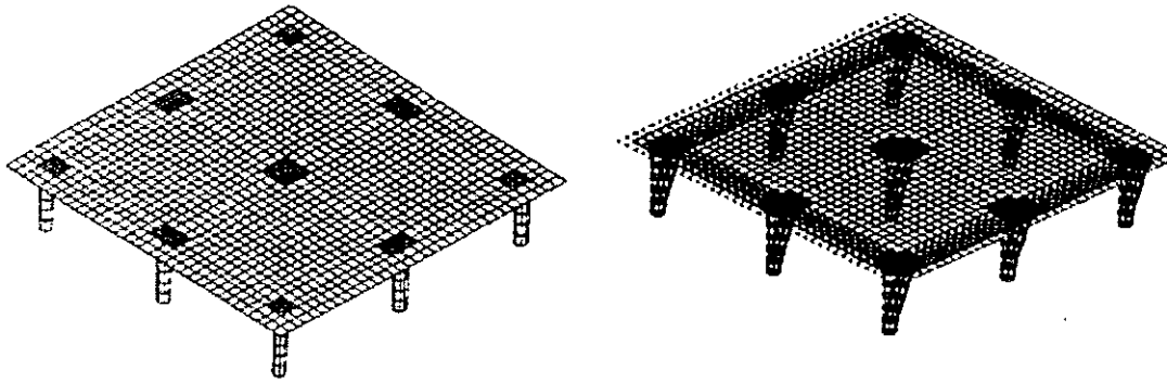
Figure 3 Finite element model of the flat slab system
