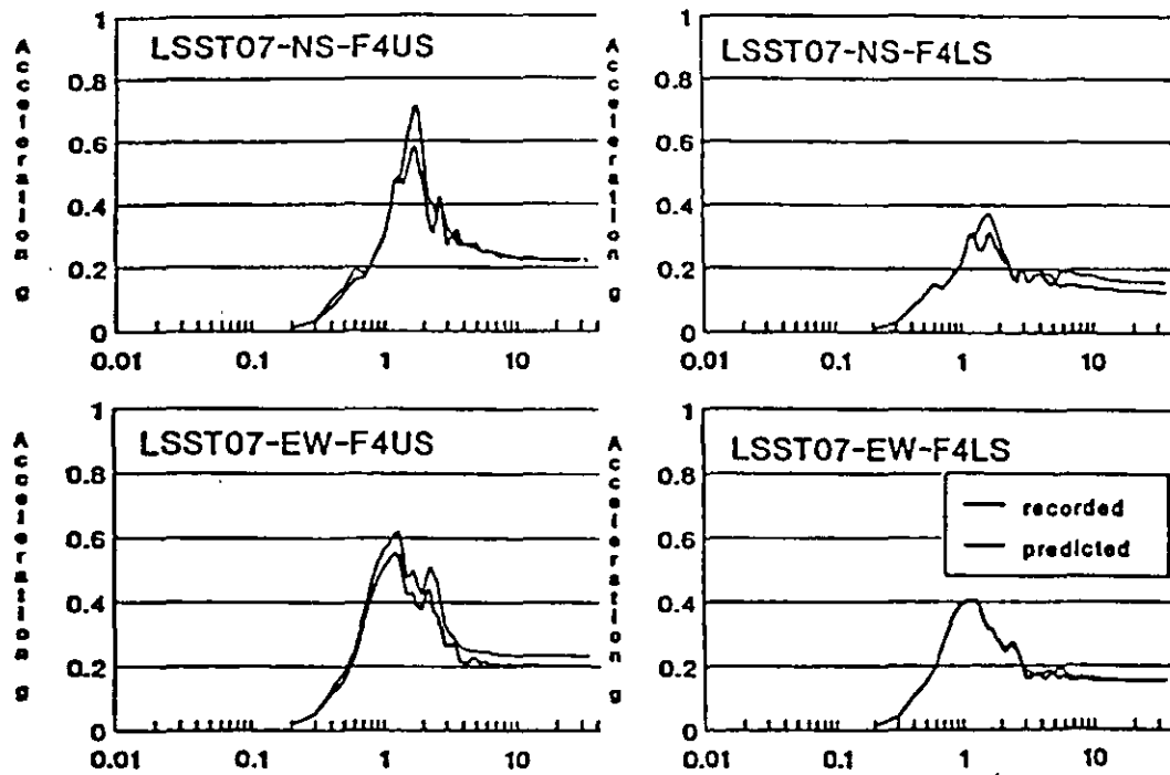
Figure 9. Predicted and recorded 5% damped response spectra, event LSST07-Soil-Spring method
