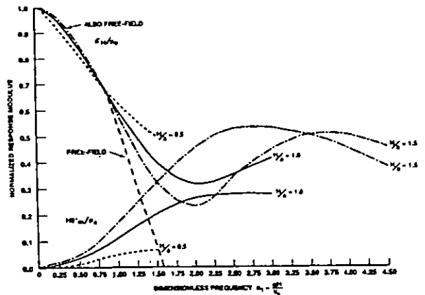
Figure 2. Normalized modulus of horizontal and rocking input motions for square foundations (adapted from Mita and Luco, 1989)
