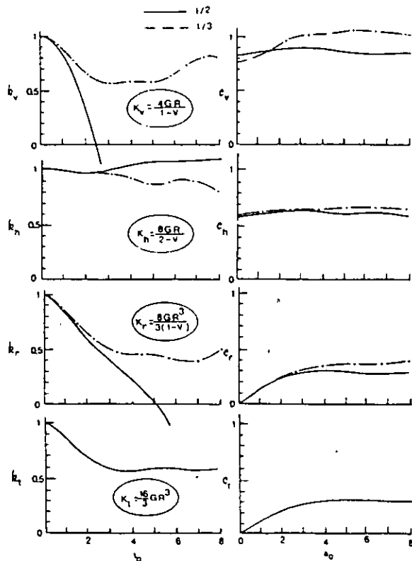
Figure 1. Impedance functions of rigid circular footings on homogeneous halfspace
