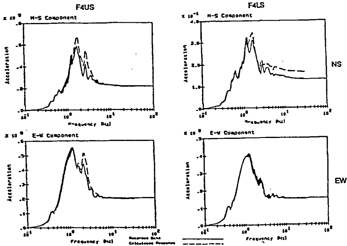
Figure 8. Predicted and recorded 5% damped response spectra for Model D, event LSST07- SUPERLUSH/CLASSI method, EQE/EET
