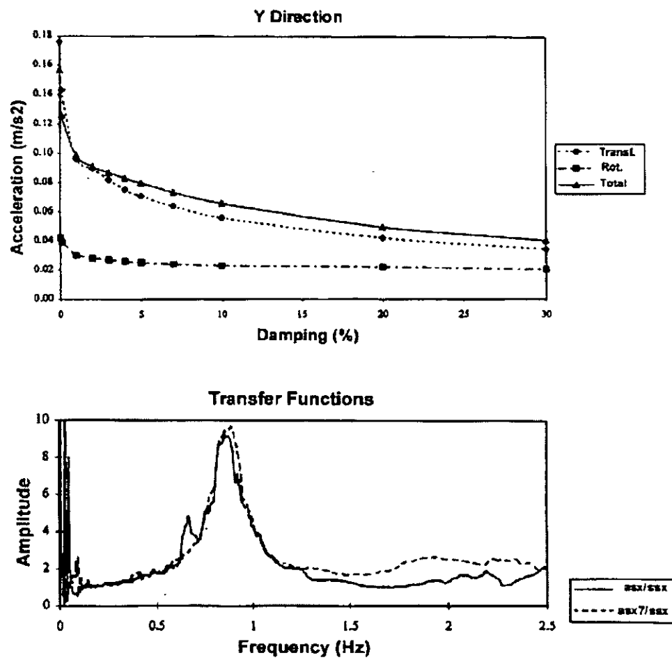
Figure 4 Effect of damping on roof acceleration
