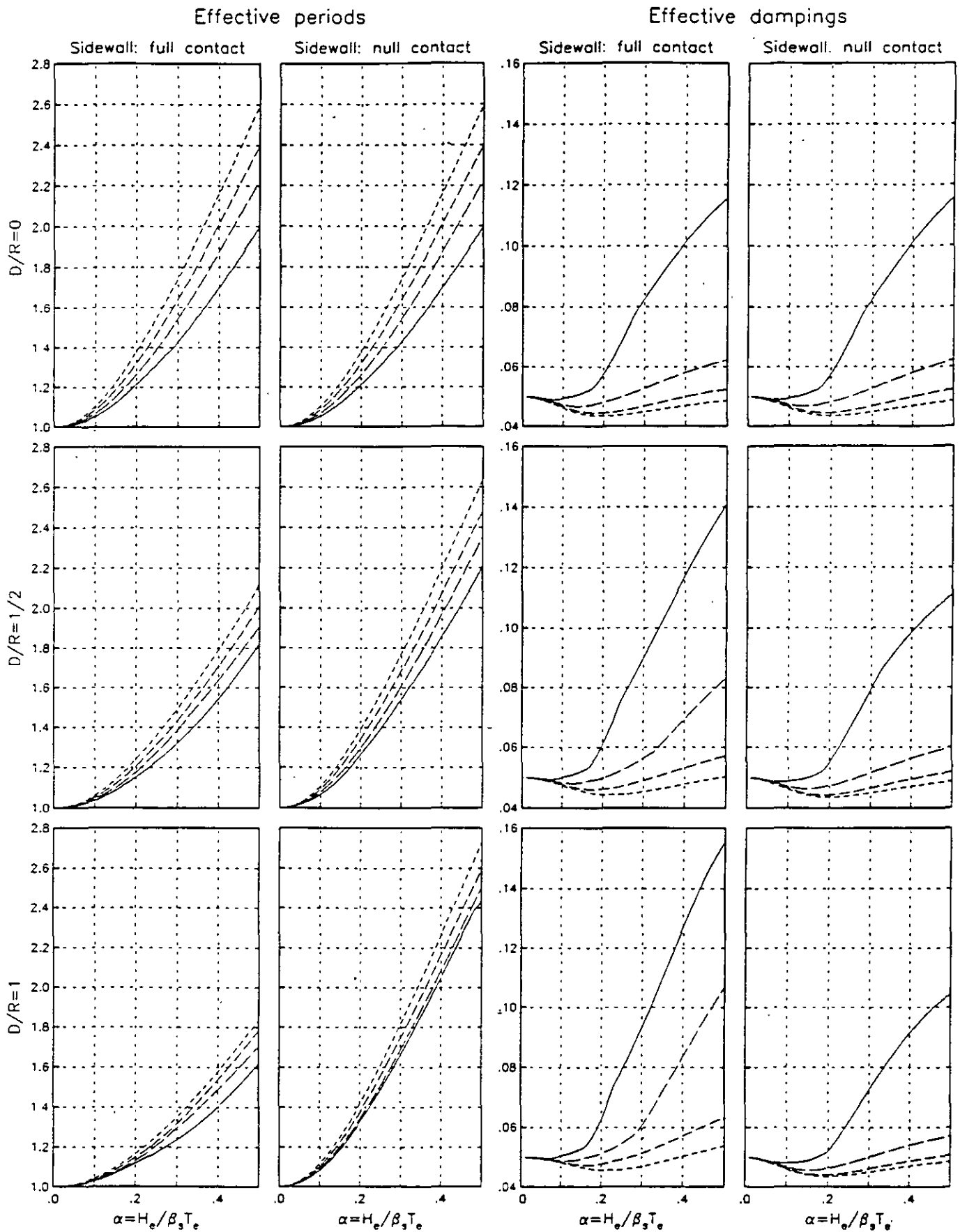
Fig. 2c Effective periods \bar{T}_e/T_e and dampings \bar{\zeta}_e of soil-structure systems for \nu_s = 1/3 and H_s/R = 6 ; curves correspond to H_e/R = 2 (solid line), 3, 4 and 5 (smallest dashed line)
