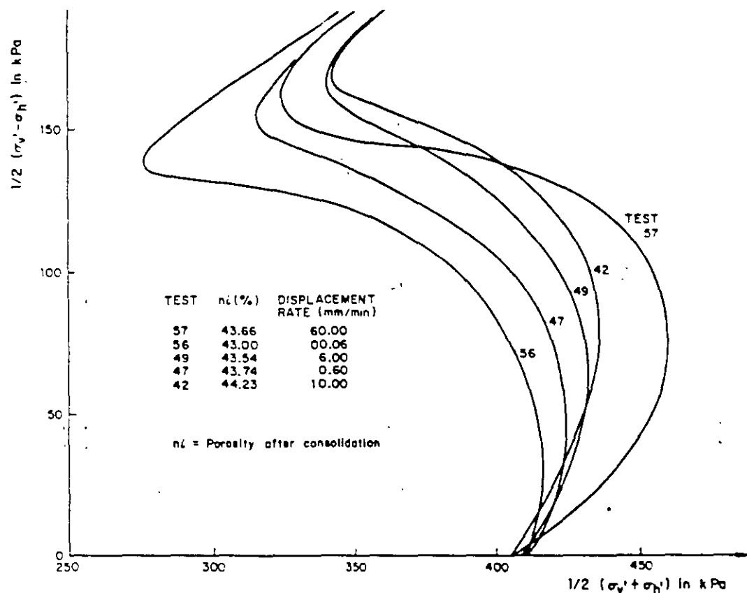
FIG 20.A Effect of axial displacement rate on the UESP s of isotropically, normally consolidated HRS (OVANDOCY HIGHT)
