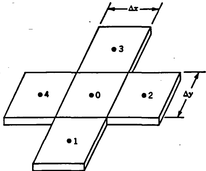
Block-centered grid.
