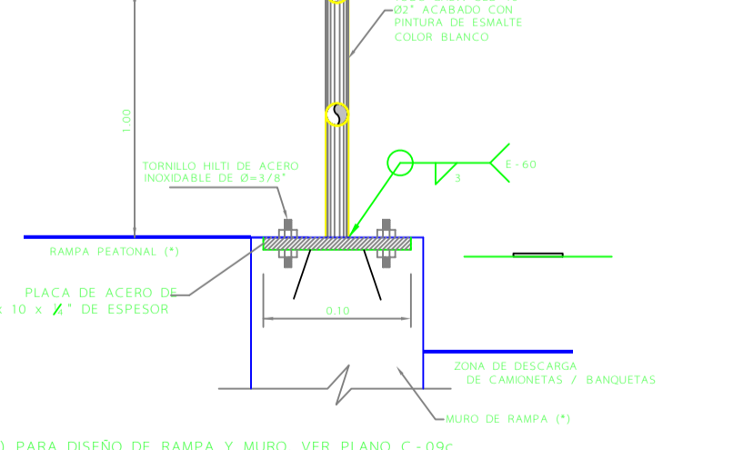
D-11 CORTE 4-4'
