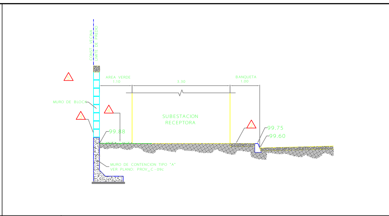
D-4 CORTE 4-4' ESC: SIN REF: D-1/C-03
