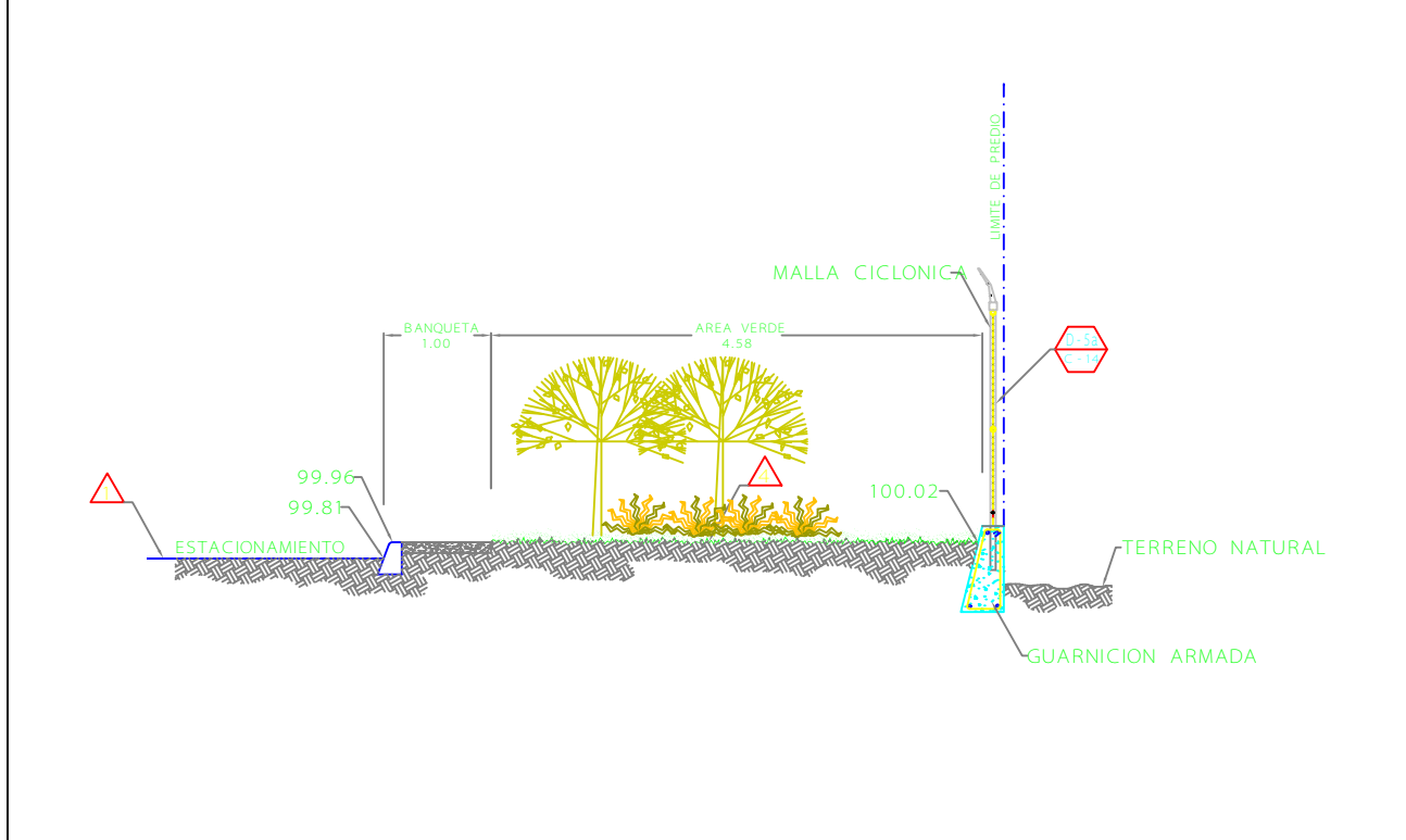
D-8 CORTE 8-8' ESC: SIN REF: D-1/C-03
