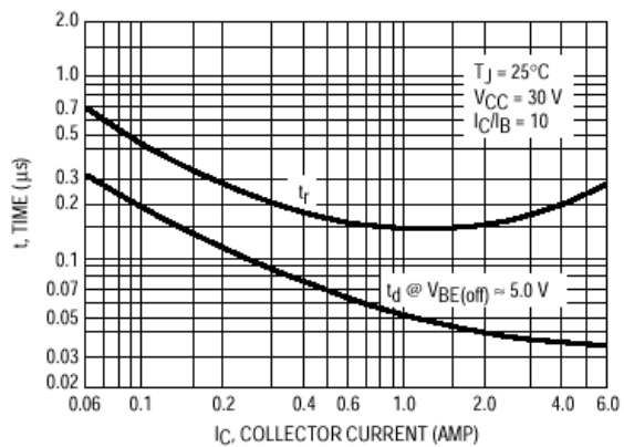
Figure 3. Turn-On Time
