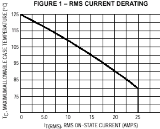
FIGURE 1 – RMS CURRENT DERATING
