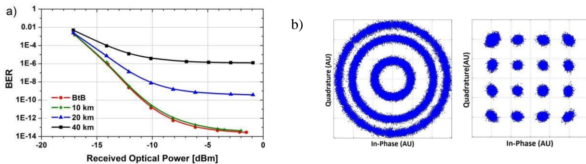
Fig. 3. a) BER of the DD-OFDM system as a function of received optical power (ROP) at the photodetector for different fiber lengths. b) Received constellation diagram prior and after equalization of the 16-QAM symbols for the 10 km setup.
