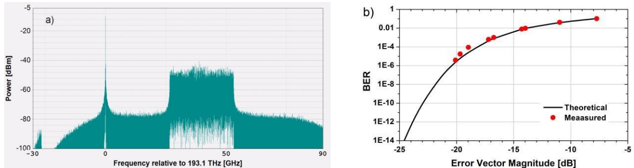
Fig. 2. a) Optical spectrum of the OFDM single sideband waveform plus optical carrier measured at the filter output (Res. 197.5 kHz). b) Calculated BER vs. EVM conversion graph for 16-QAM using a 10-km long SMF. The solid line stands for the theoretical (formula) values.
