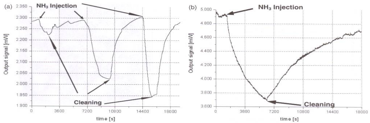
Figure 3. Output signal as a function of time for (a) 160, 2300 and 5000 ppm of NH 3 at \lambda = 980 nm and (b) 5000 ppm of NH 3 at \lambda = 1550 nm.
