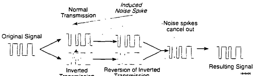
Figure 11-5. Twisted Pair Signal Equalization
