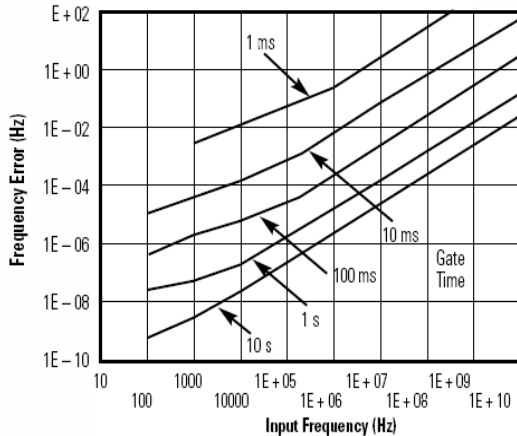
Graph 5: Agilent 53132A—Worst Case RMS Resolution 7 (Time or Digits Arming)
