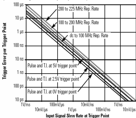
Graph 6: Trigger Level Timing Error (Level Setting Error and Input Hysteresis)
