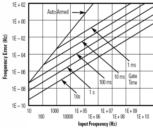
Graph 4: Agilent 53132A—Worst Case RMS Resolution 7 (Automatic or External Arming)
