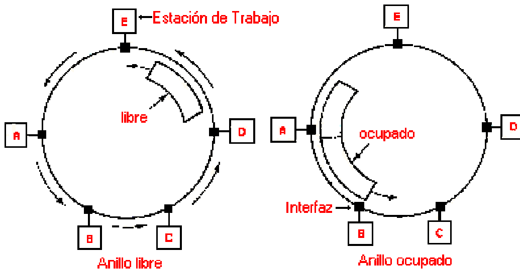
Figura 2.7.2.4.1 Red Token Ring.
