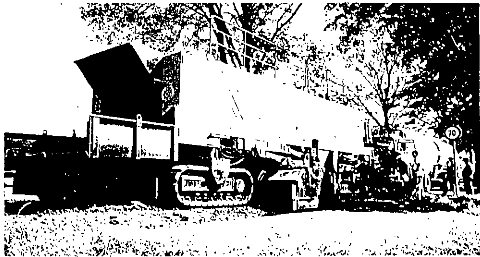
Wirtgen cold recycling: the existing road materials are reused to produce a strong foundation course
