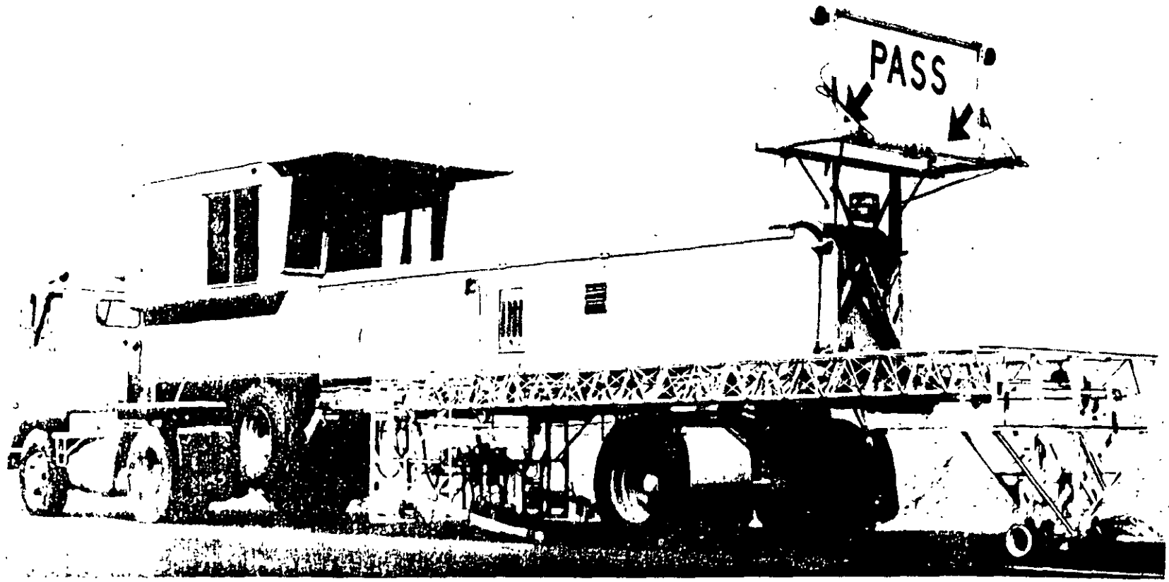
FIGURE 2 DEFLL METER
