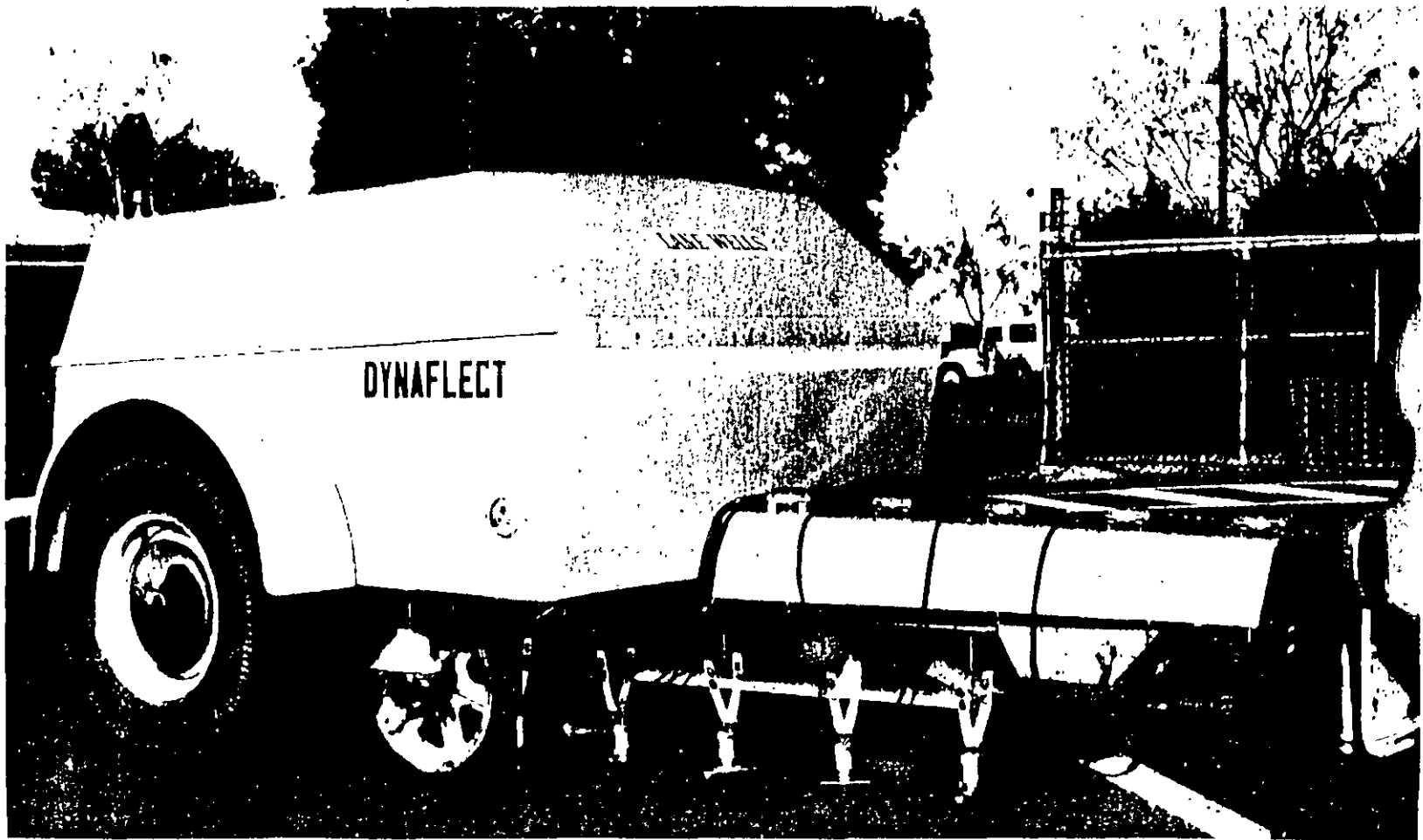
7 FIGURE 3 DYNAFLECT IN TEST POSITION WITH FORCE WHEELS AND GEOPHONES DOWN
