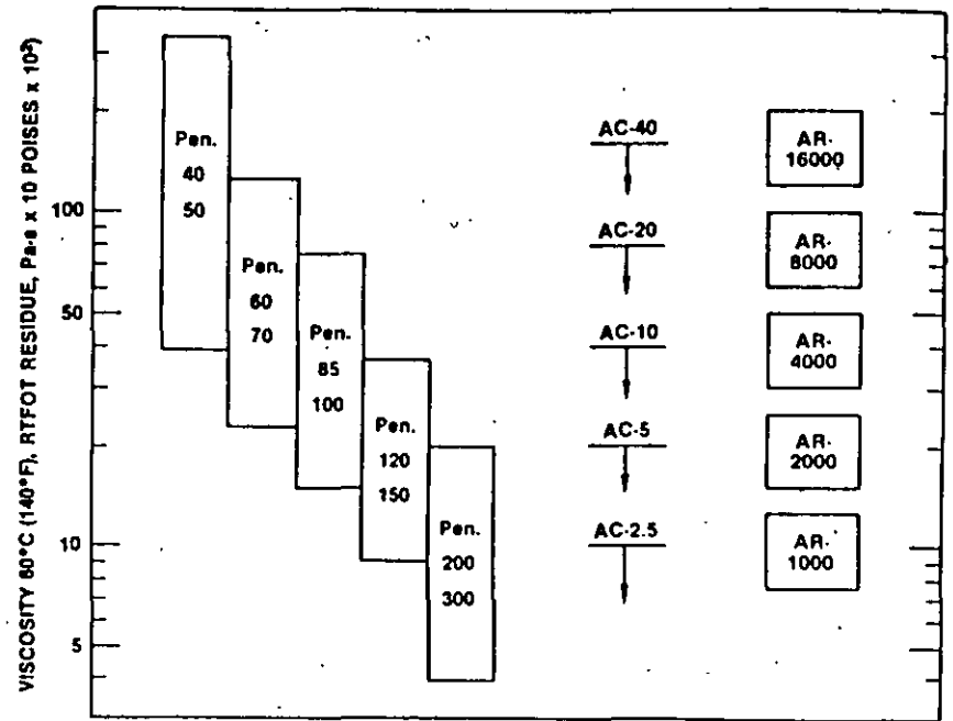
Figure III-4—Comparison of penetration grades and viscosity grades of asphalt cement (based on RTFOT residue for AR-grades and penetration grades; TFOT residue for AC-grades).
