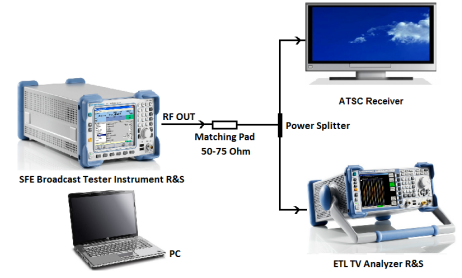
Fig. 1. Laboratory test setup.
