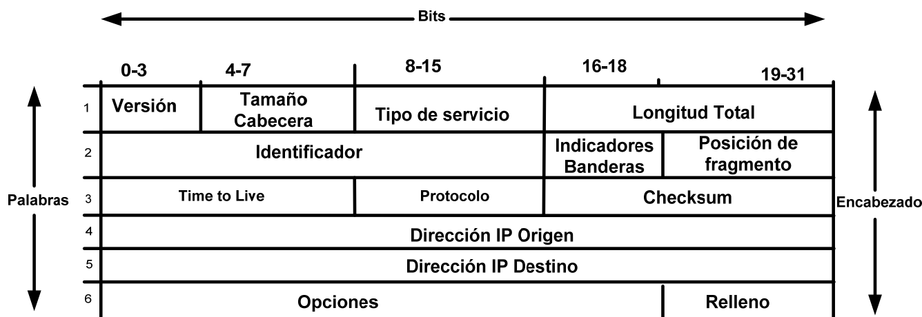
Figura 1. 10 Datagrama IP.
