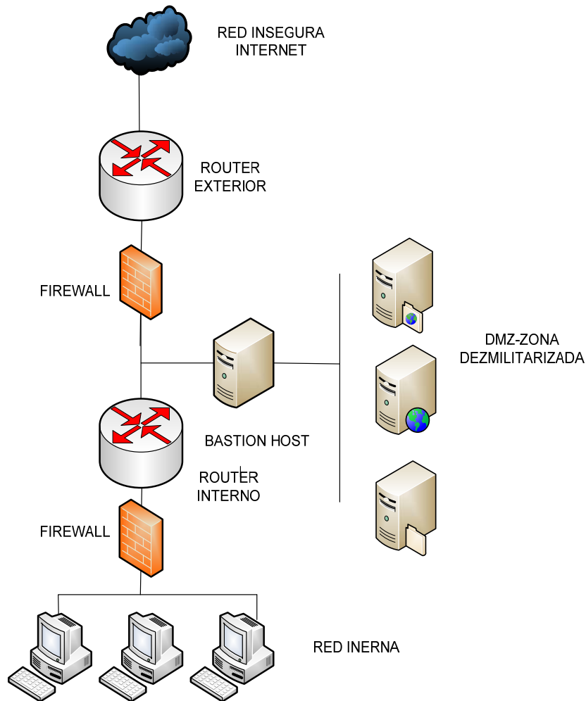
Figura C. 4 Screened subnet firewall.
