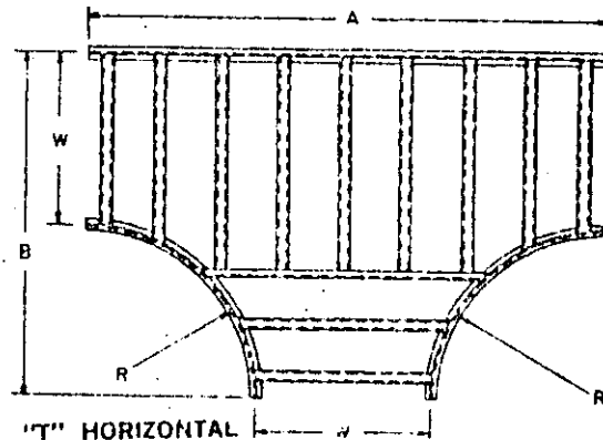
"T" HORIZONTAL
