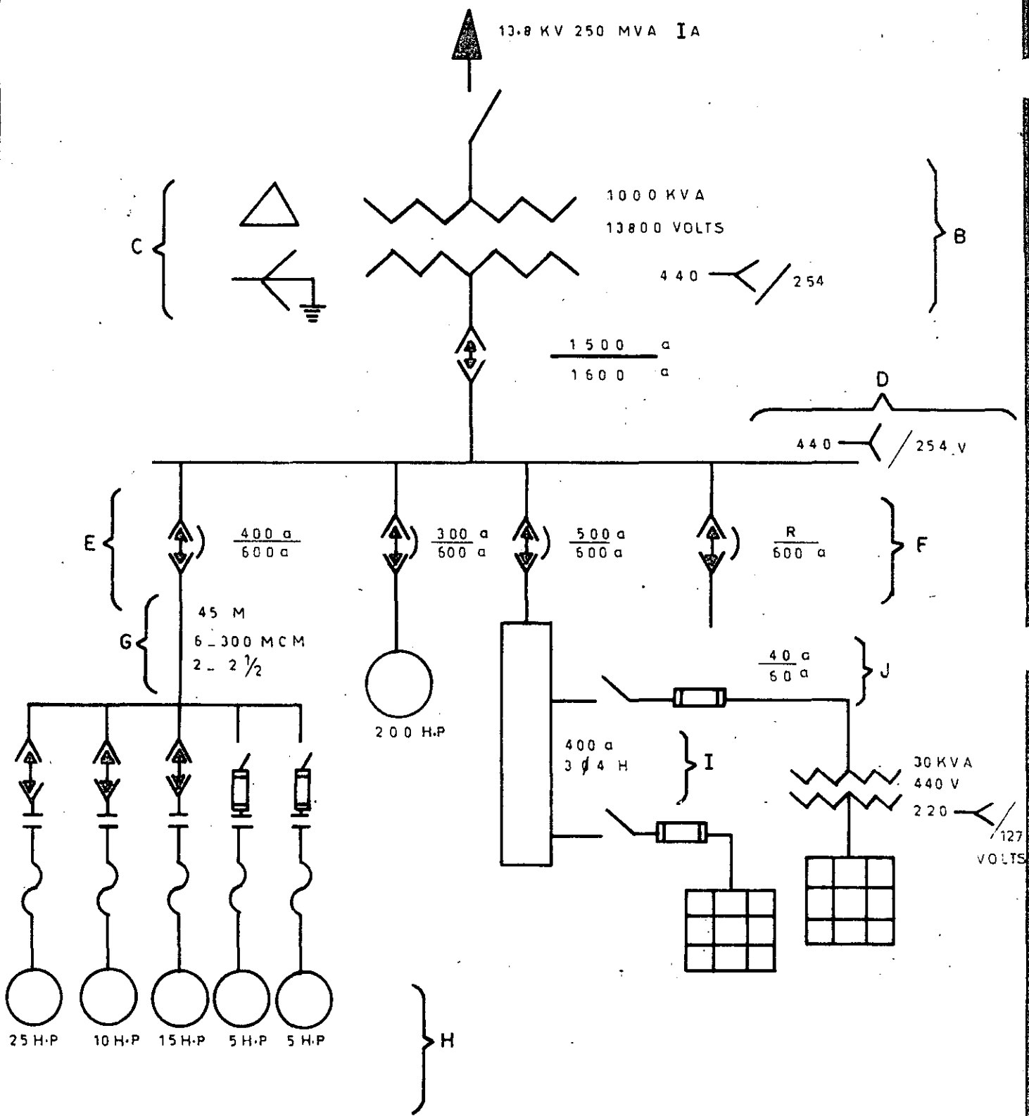
DIAGRAMA UNIFILAR
