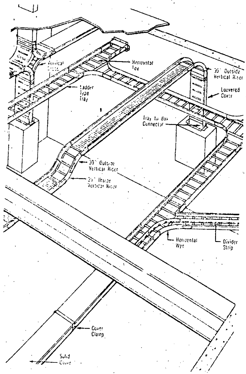
9-152 INTERIOR WIRING
