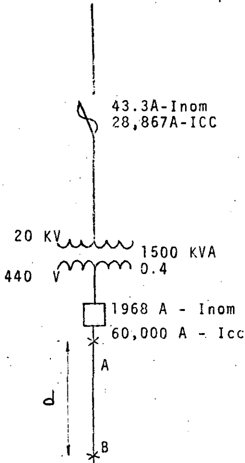
Diagrama unifilar
