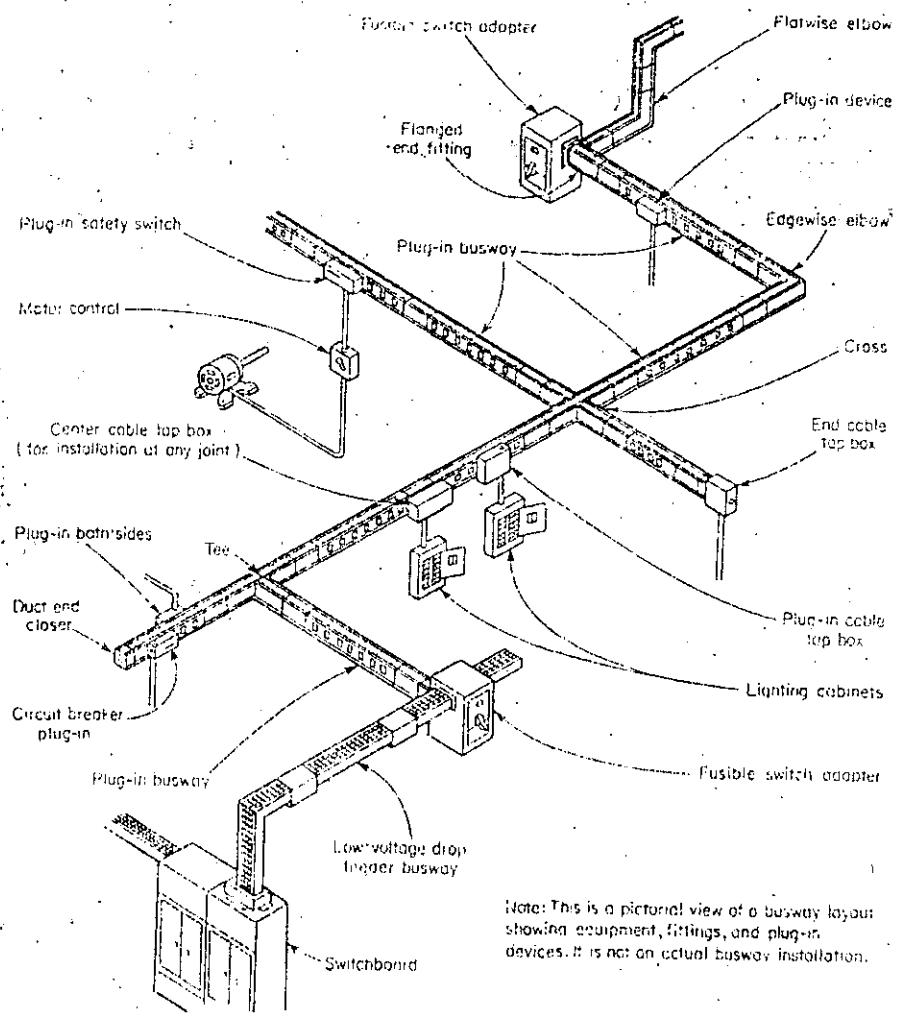
FIG. 16-1 Typical plug-in bus-way (power-type) system. (National Electric Dist., H. K. Potter Co., Inc.)
