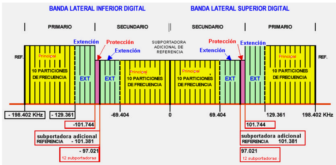
Fig. 2.9 IBOC Digital
