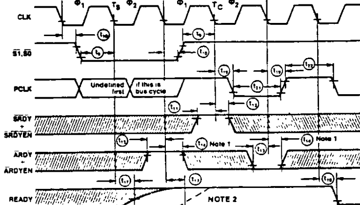
READY and PCLK Timing with RES HIGH
