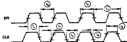
CLK as a Function of EFI (82284-6 only)
