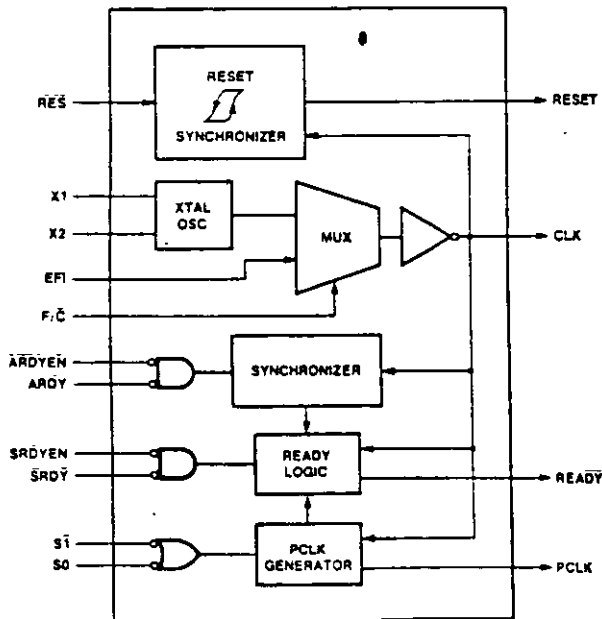
Figure 1. 82284 Block Diagram
