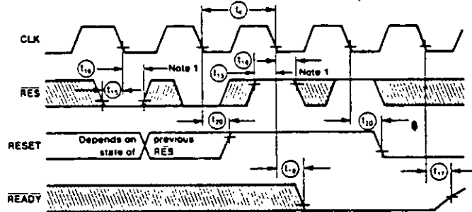
RESET and READY Timing as a Function of RES with S1, S0, ARDY to ARDYEN, and SRDY + SRDYEN HIGH
