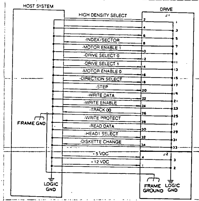
INTERFACE CONNECTIONS
