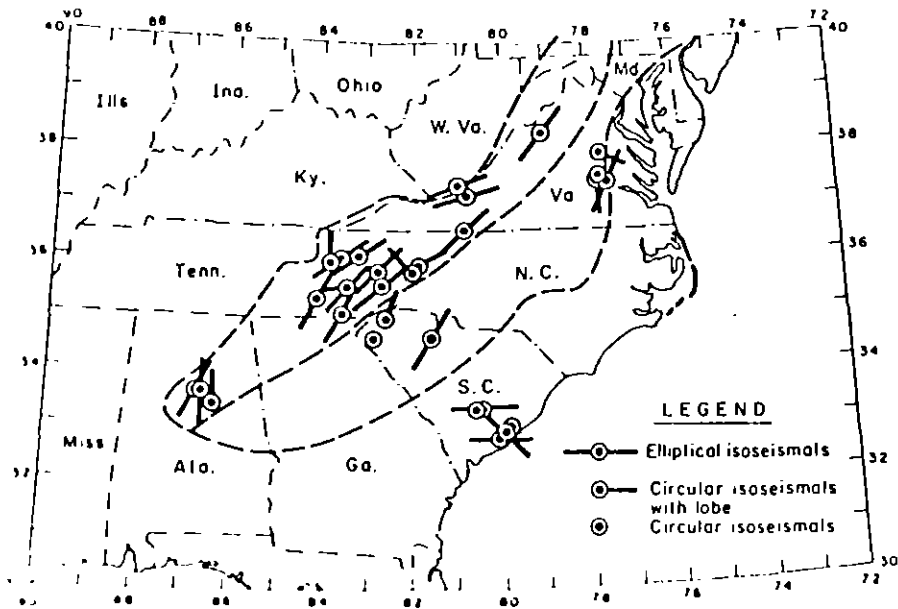
Fig. 6.2. Extension of isoseismals in the southeastern United States. (After Bollinger, 1953.)
