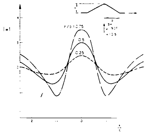
Fig. 10. Displacement amplitudes at the free-surface. Ridges with different aspect ratio h/b . Vertical incidence of SH waves with normalized frequency \eta=0.5
