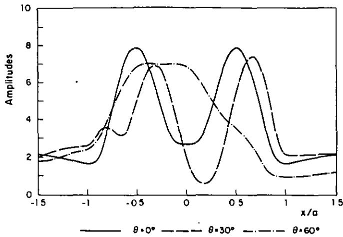
FIG. 5. Displacement amplitudes on the surface of the parabolic stratified deposit of Figure 4. Normalized frequency is \eta = 1.0 , and incidence angles are \theta = 0^\circ, 30^\circ , and 60^\circ .
