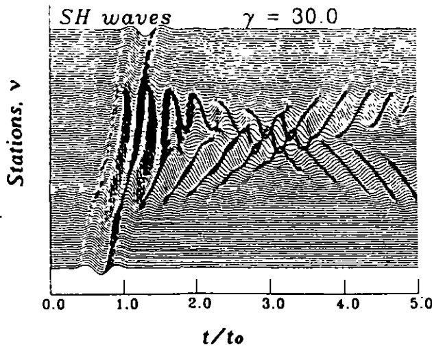
Fig. 14. Synthetic seismograms for incidence of SH waves in 51 stations (from -1.25a to 1.25a ) across the surface of the two-dimensional model.
