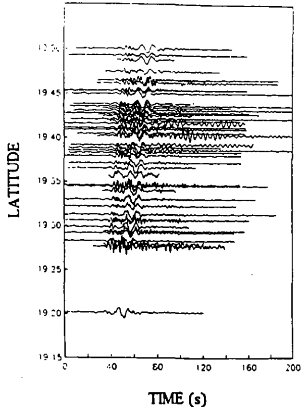
Fig. 4. Vertical displacements for 60 stations of the MCAA with a common time basis.
