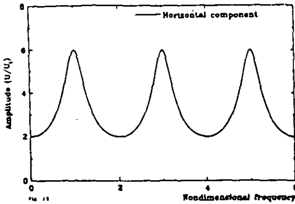
Fig. 23. The amplification factor due to a surface layer for normally incident S waves. The peak amplification is equal to twice the impedance contrast (\rho_2/\beta_2)/\rho_1\beta_1 , which is 6 in this case.
