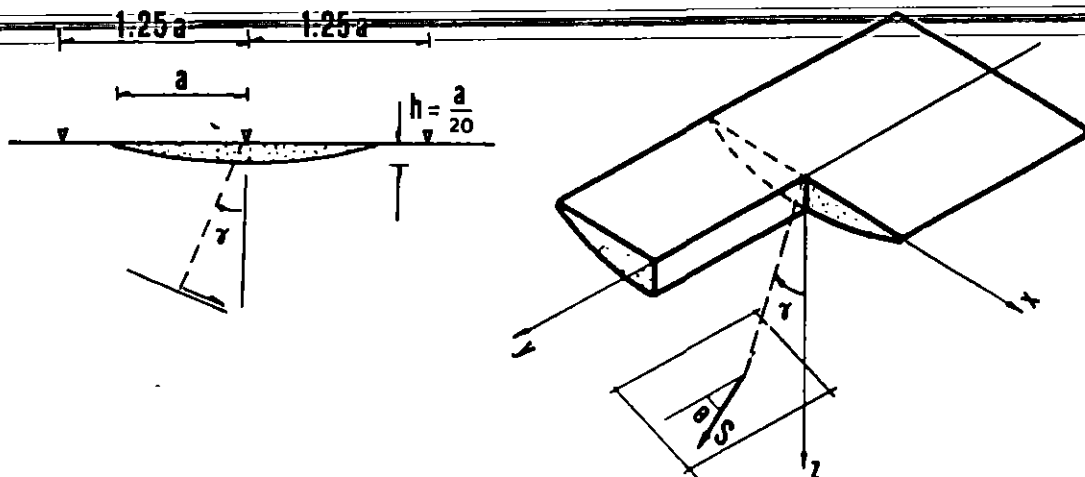
Fig. 13. Soft alluvial valley with parabolic interface under incidence of plane S waves. Incidence and polarization angles are represented by \gamma and \theta , respectively.
