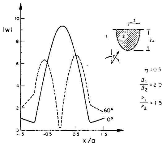
Fig. 9. Displacement amplitudes at the free-surface. Semi-elliptical alluvial valley. Incidence of SH waves with angles 0° and 60 degrees. Normalized frequency \eta=0.5
