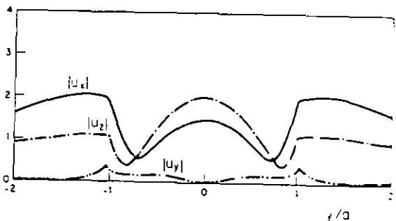
Fig. 12. Surface displacement amplitudes. Semi-spherical canyon under incidence of P waves with incidence angle of 60^\circ and normalized frequency \eta_k = 1.0 (Poisson ratio 0.25)
