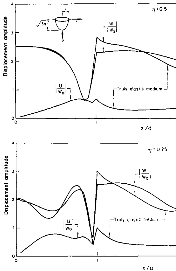
Fig. 5. Displacement amplitudes in a semi-ellipsoidal surface cavity under vertical incidence of P waves. Vertical displacements are computed for a simplified elastic medium in which horizontal motion is restricted. Comparison is provided with computations for a truly elastic medium
