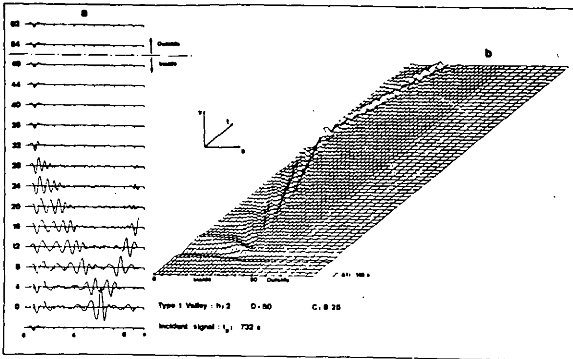
Fig. 26. Response of a type 1 valley with maximum depth h=200 m, half-width D=5 km, to a vertically incident SH Ricker wavelet of characteristic period 0.732 sec. (a) The traces represent the displacement at surface receivers, spaced from 0 to 6.2 km from the Valley Center. The bottom trace would be the surface displacement without the valley. (b) Diagram showing the spatial ( x ) and temporal evolution of the surface displacement in the valley and in its vicinity. The dots indicate the location of sites where the seismograms in (a) are computed. (Reproduced from Bard and Bouchon (1980a).)
