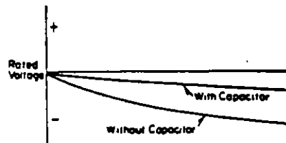
Figure 16. Voltage profile on feeder with distribution load.
