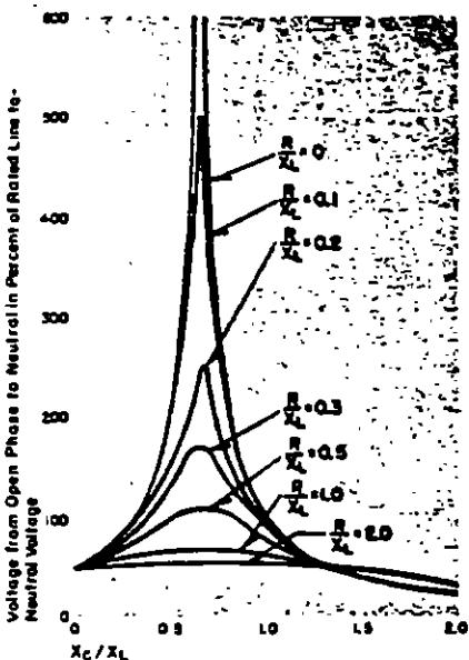
Figure 28. Overvoltages possible due to resonant conditions with one phase open.
