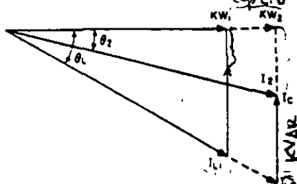
Figure 12. Vector diagram for voltage limited circuits.
