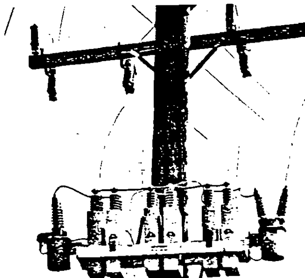
Figure 2. Pole-mounted Capacitors
