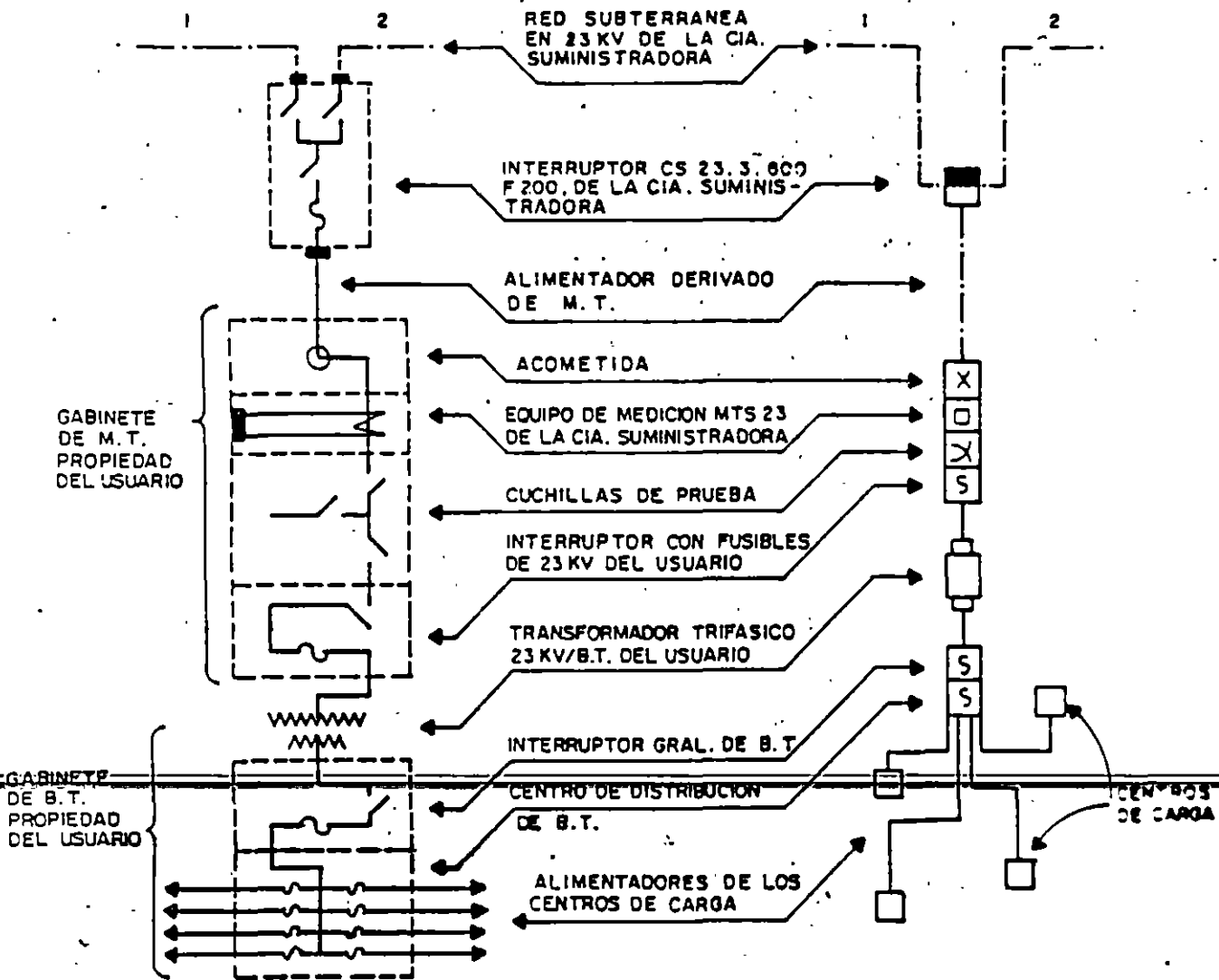
DIAGRAMA UNIFILAR
