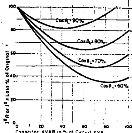
Figure 9. Reduction in circuit losses from adding capacitors.
