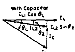
Figure 1. Fundamental vector diagrams showing effect of shunt capacitors.
