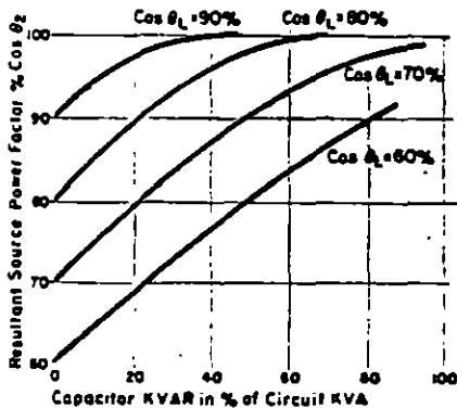
Figure 10. Increase in source power factor as a function of effect of shunt capacitors.
