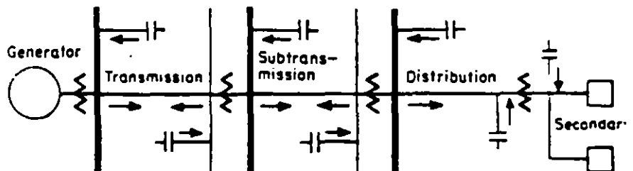
Figure 17. Typical system capacitor bank locations (arrows indicate direction of VAR flow for maximum system losses).
