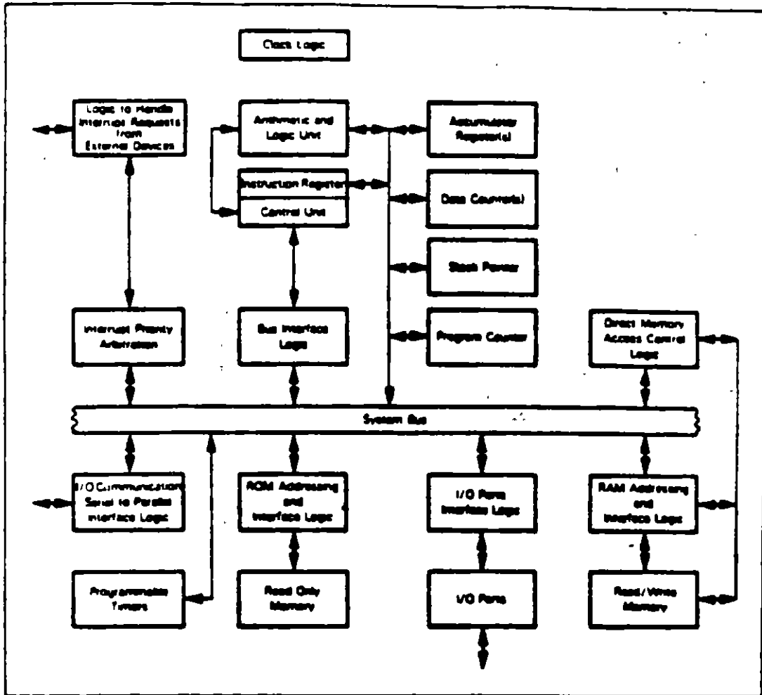
Figure 20-1. Logic of the Intel 8085 CPU
