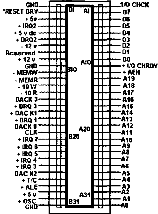
I/O CHANNEL SLOT
