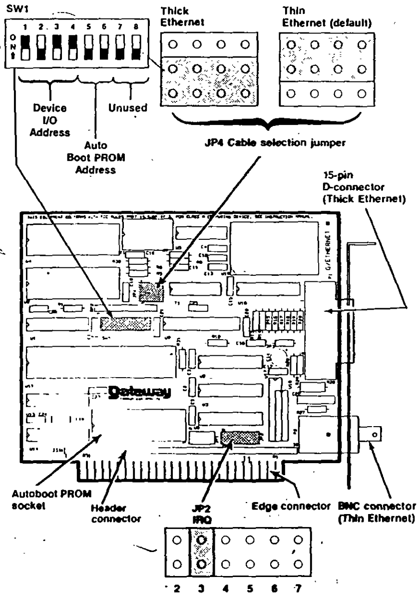
Figure 2-1. G/Ethernet 8 Component Locations.
