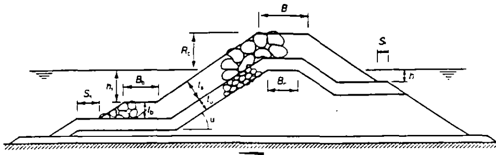
Figure 239 Definition sketch for a rubble-mound breakwater
