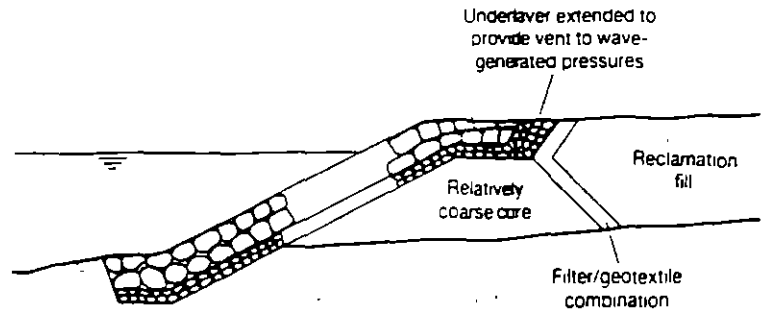
Figure 294 Land-reclamation revetment
