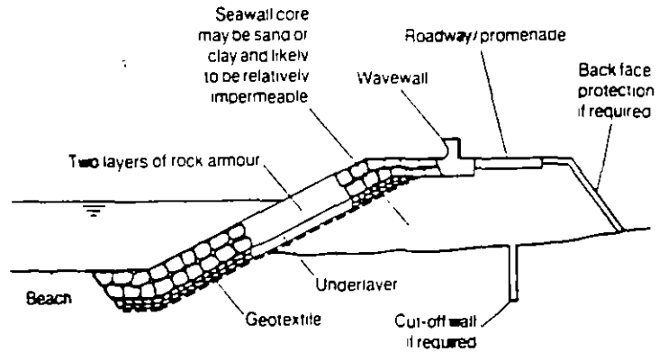
Figure 293 Sea-defence revetment
