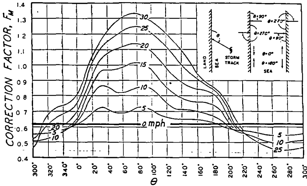
Figure 3.--Nomogram of correction factors against the vector storm motion. The factor corrects for motion other than standard; standard motion is a vector track, 090^{\circ}/15 mph, relative to the coastline. The inset gives orientation of the argument \theta and also gives some extreme tracks relative to the coast.
