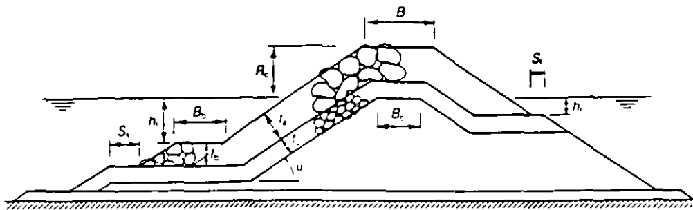
Figure 239 Definition sketch for a rubble-mound breakwater
