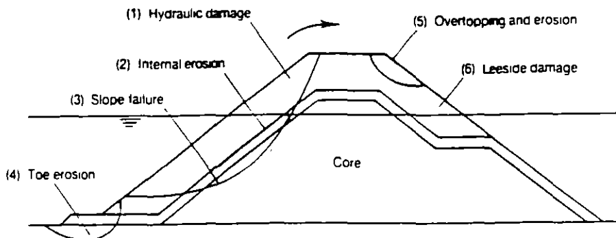
Figure 240 Failure mechanisms of a rubble-mound breakwater
