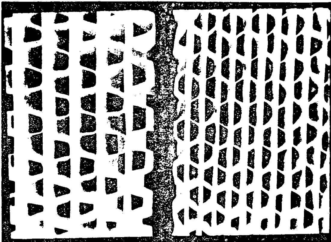
Cross-section of RBC media showing alternating flat and corrugated sheets. Left-side, regular media; Right-side, high density media. (Courtesy of Autotrol Corp.).
