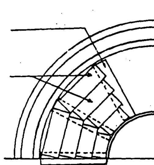
PLAN VIEW OF MODIFIED CLARIFIER
