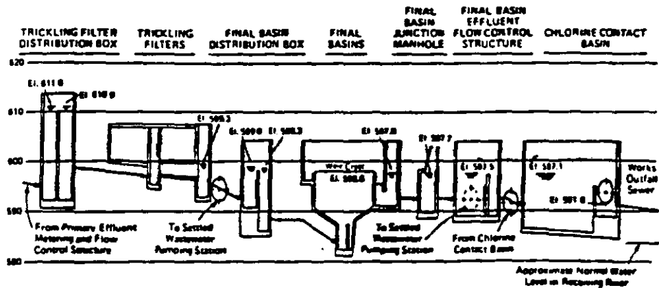
Figure 5.3 Typical hydraulic profile for a trickling filter plant. Water surface elevations represent flow of 85 000 m 3 /d (22 mgd).
