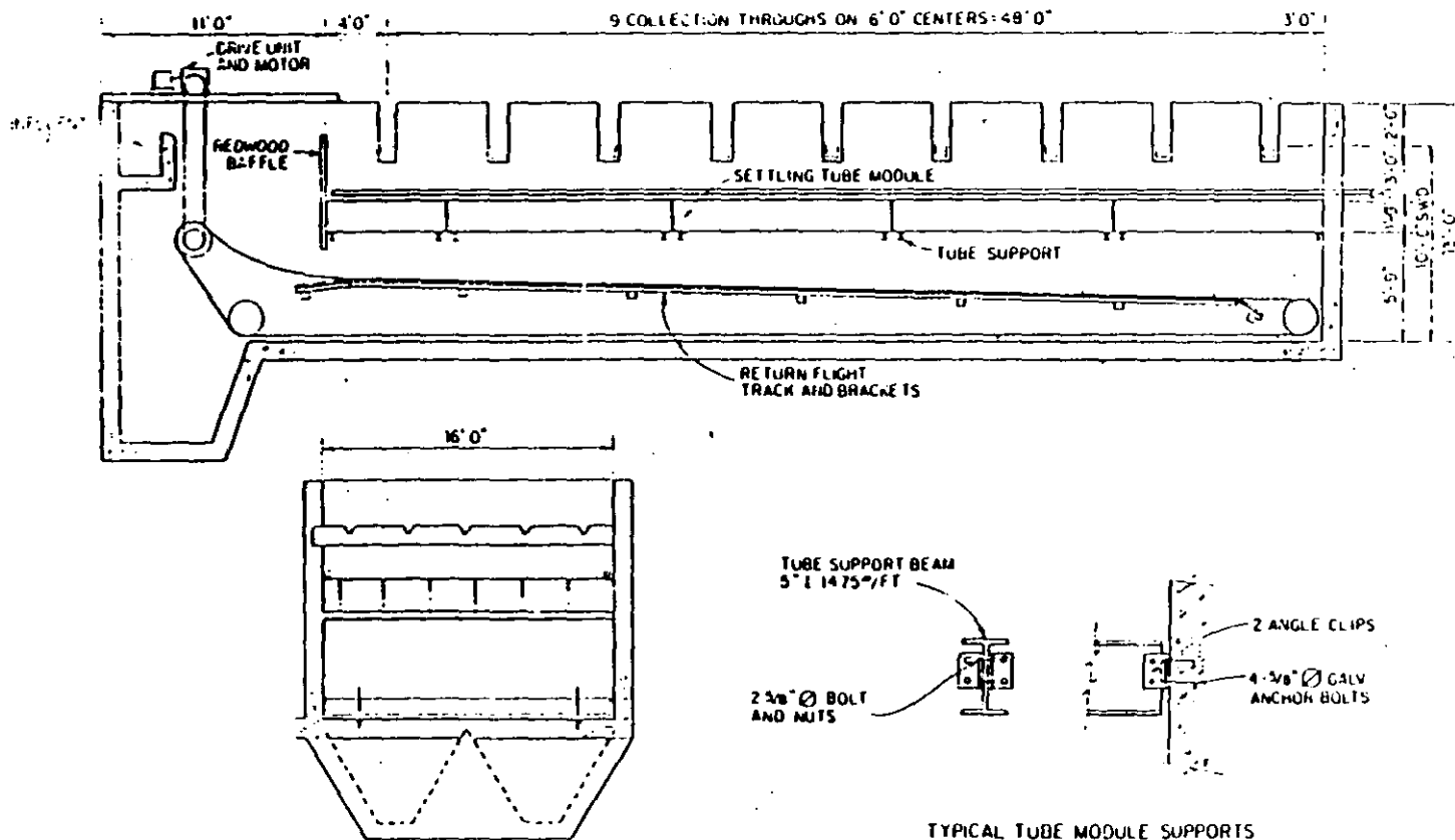
Figure Cross section of typical tube clarifier for clarification of chemically coagulated secondary effluent. (Courtesy Neptune Microfilm, Inc.)
