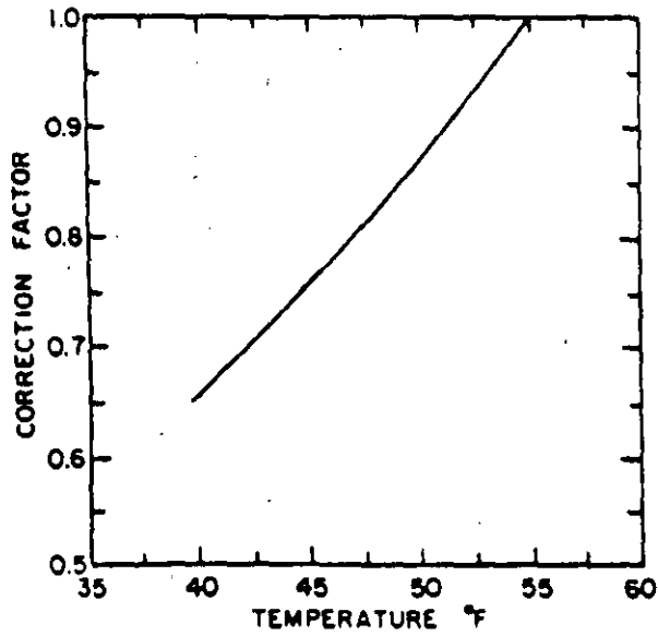
Empirical temperature correction factor which the hydraulic loading rate can be multiplied to maintain the same BOD 5 removal. (Courtesy of Autotrol Corp.).
