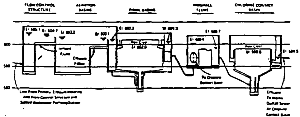
Figure 5.2 Typical hydraulic profile for an activated sludge plant. Water surface elevations in feet above msl represent flow of 160 000 m 3 /d (42 mgd).
