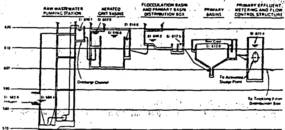
Figure 5.1 Typical hydraulic profile for influent pumping and primary treatment. Water surface elevations in feet above msl represent flow of 160 000 m 3 /d (42 mgd).
