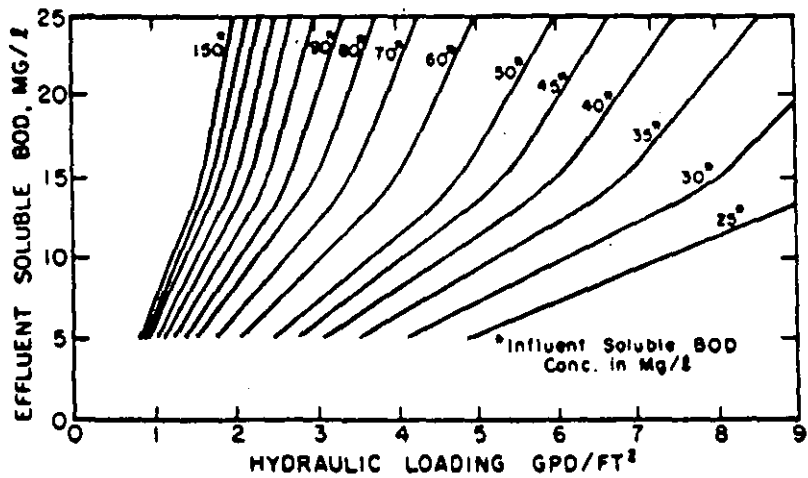
Design correlation for soluble BOD 5 removal in municipal wastewater treatment. (Courtesy of Autotrol Corp.).
