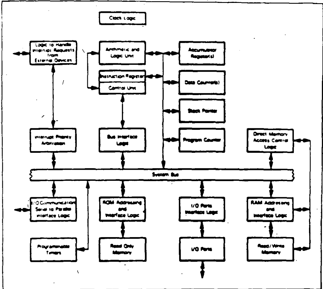
Figure 20-1. Logic of the Intel 8086 CPU
