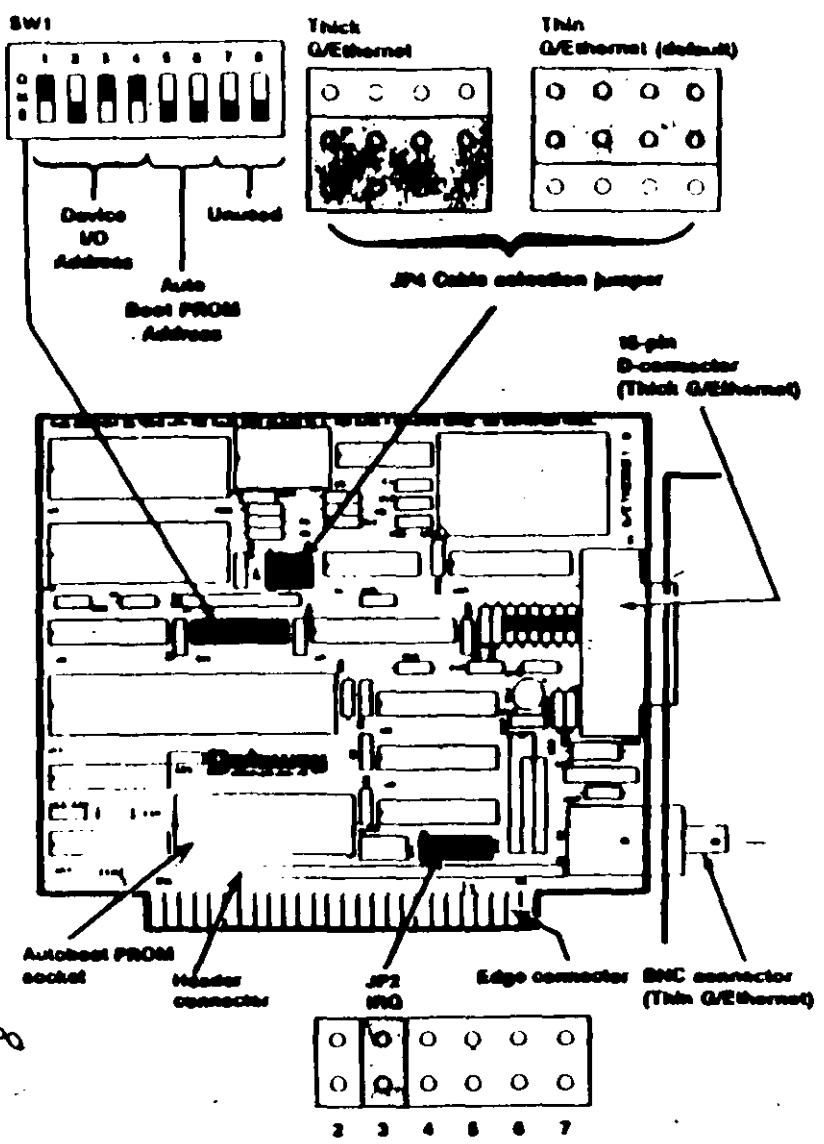
Figure 2-1. Ethernet 16-bit Component Locations.
