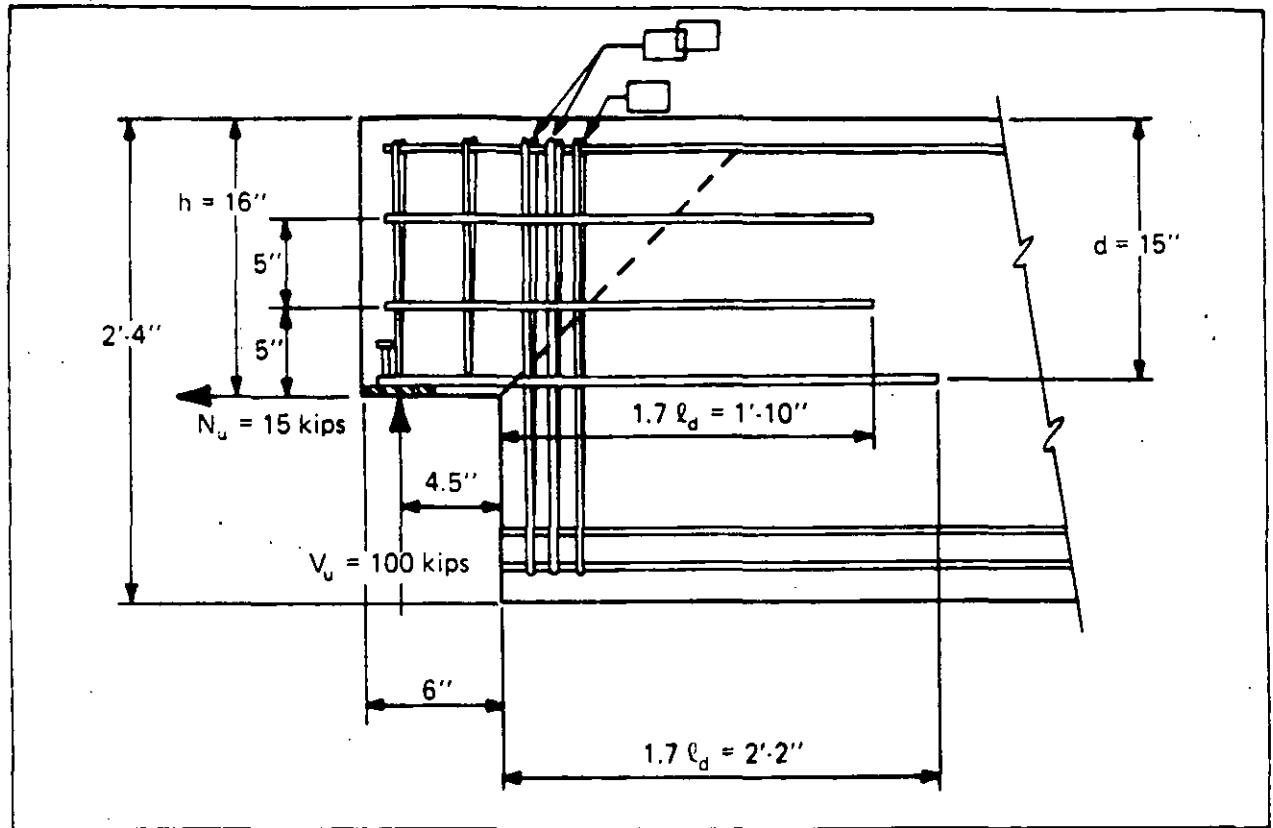
Fig. 5.9.2 Dapped-end beam of Example 5.9.1
