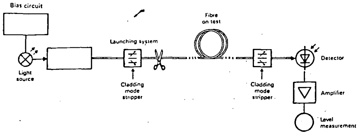
FIGURE B-10/G.651
