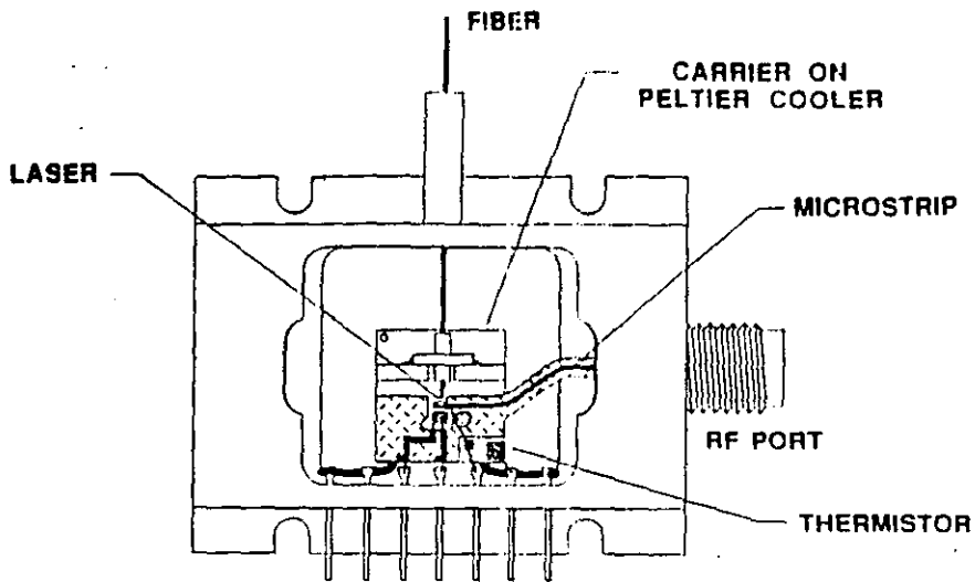
Figure 1. Unmatched wide-bandwidth diode laser package with bias insertion network.
