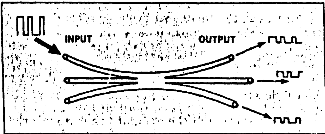
Fig. 3 Passive star operation.
