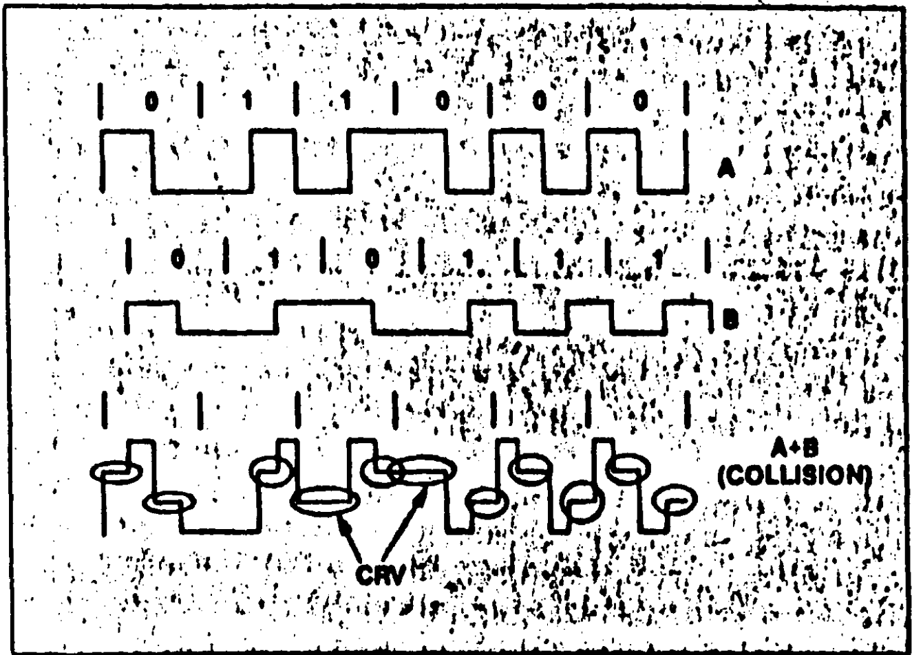
Fig. 1 Manchester CRV technique for collision detection.
