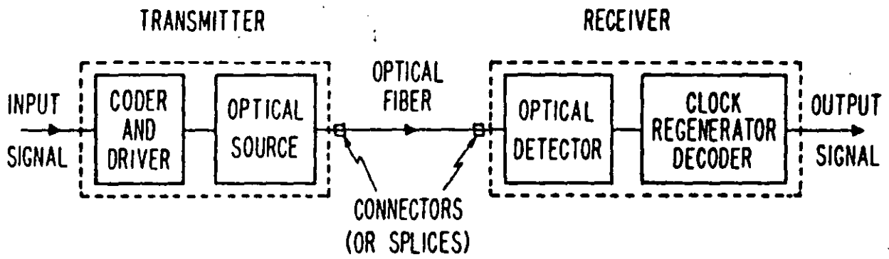
Fig. 1. A simple optical-fiber communications link.
