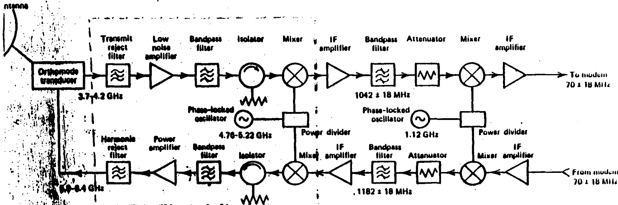
Fig. 1. Block diagram of a C-band earth terminal.
