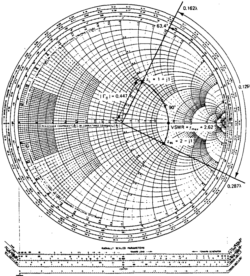
IMPEDANCE OR ADMITTANCE COORDINATES
