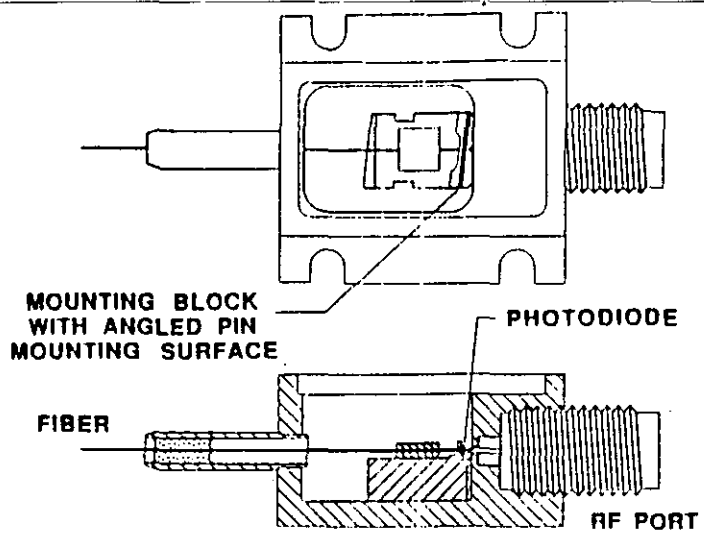
Figure 6. Top and side views of a wide-bandwidth unmatched photodetector package.
