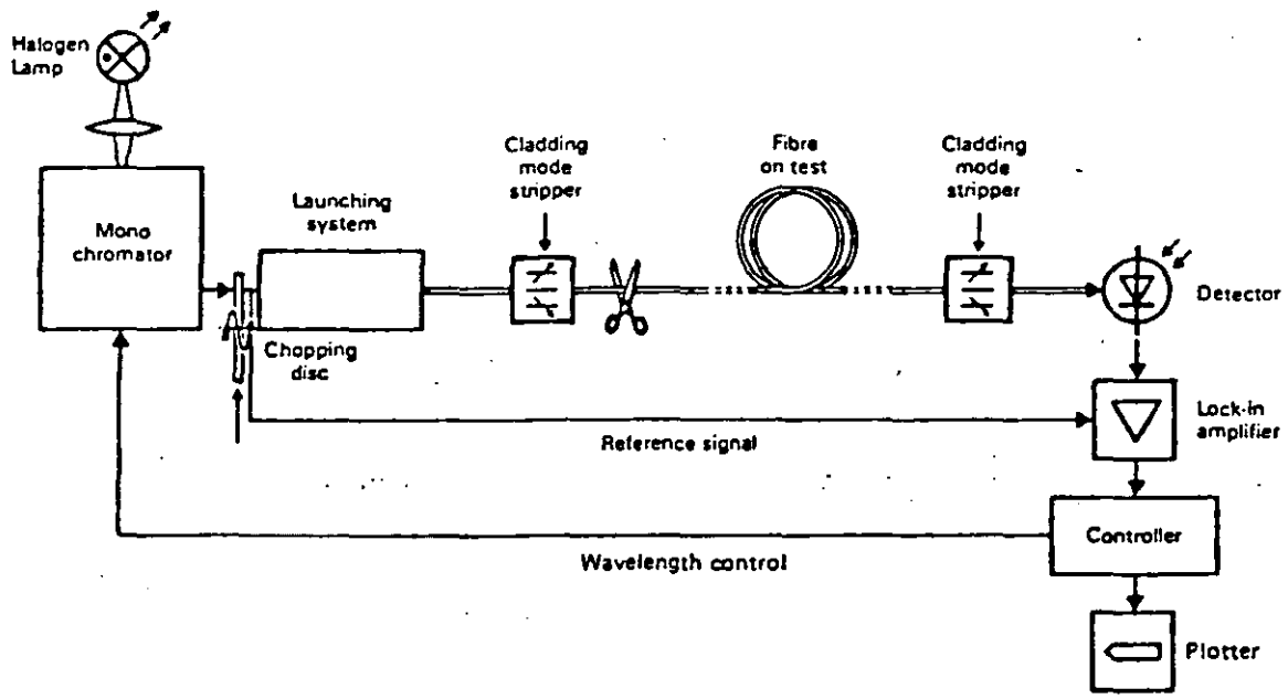
Arrangement of test equipment used to obtain the loss spectrum
