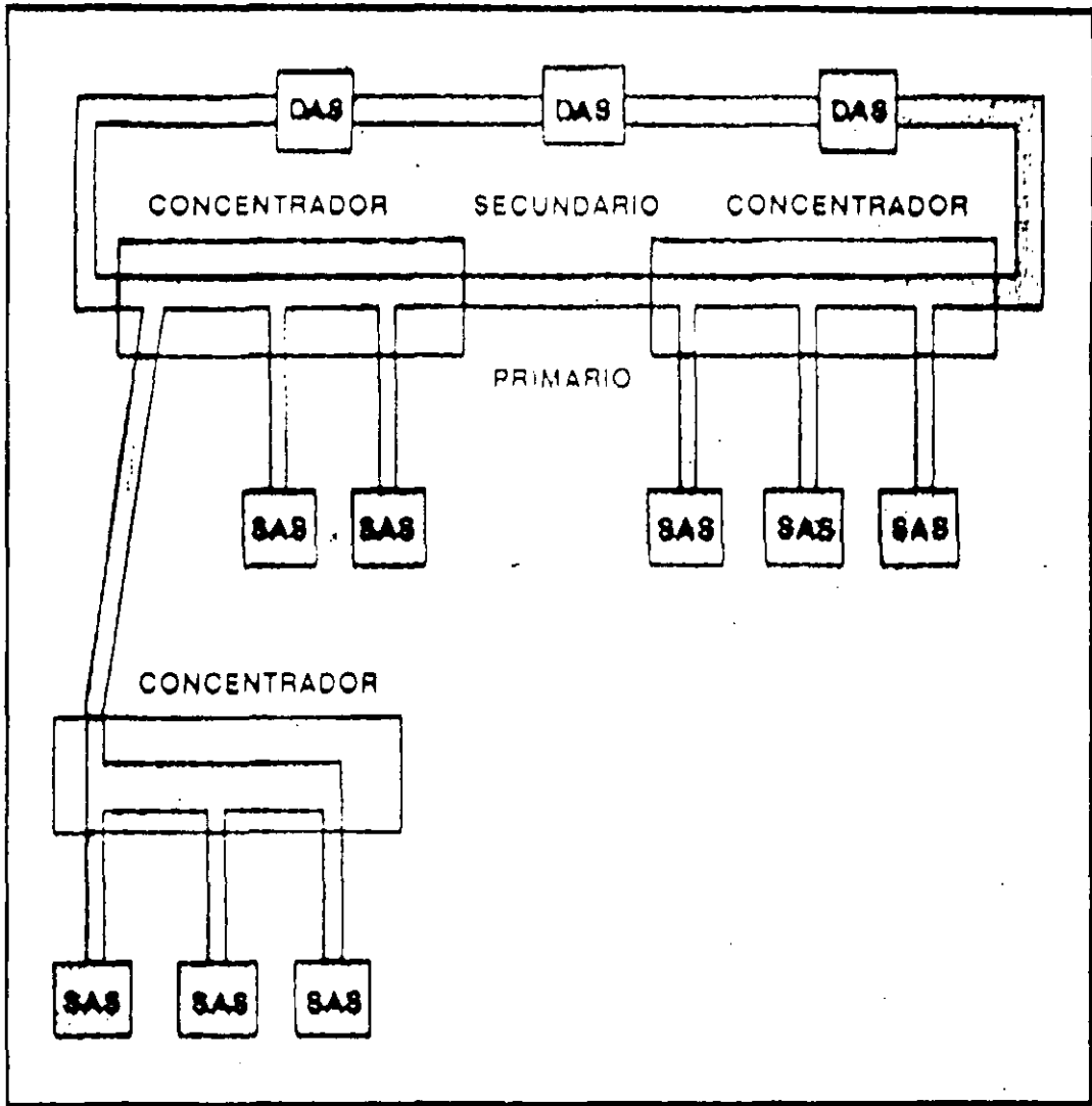
TOPOLOGIA FDDI
