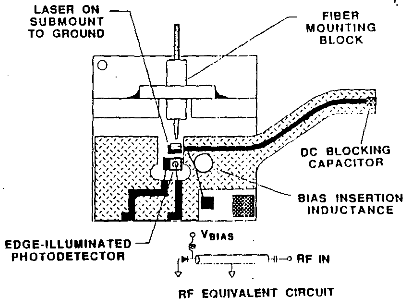
Figure 2. Detail view of unmatched wide-bandwidth diode laser package mount.
