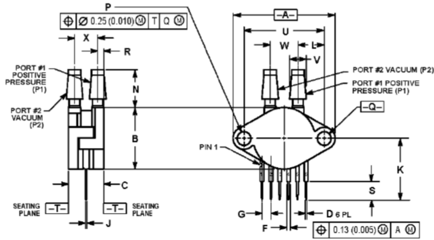
CASE 867C-05 ISSUE F UNIBODY PACKAGE
