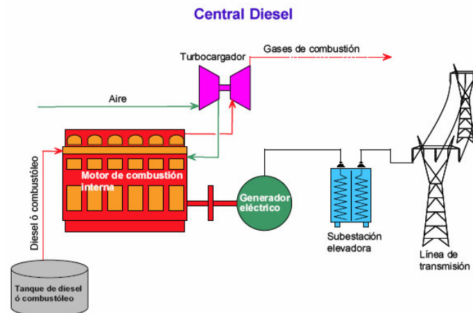
Figura 1.5.1. Central diesel
