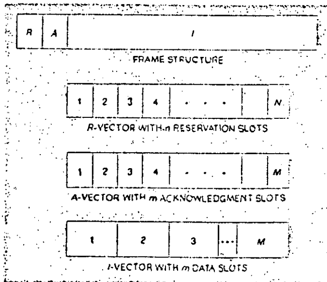
Fig. 3. Frame structure for CFMA channel.
