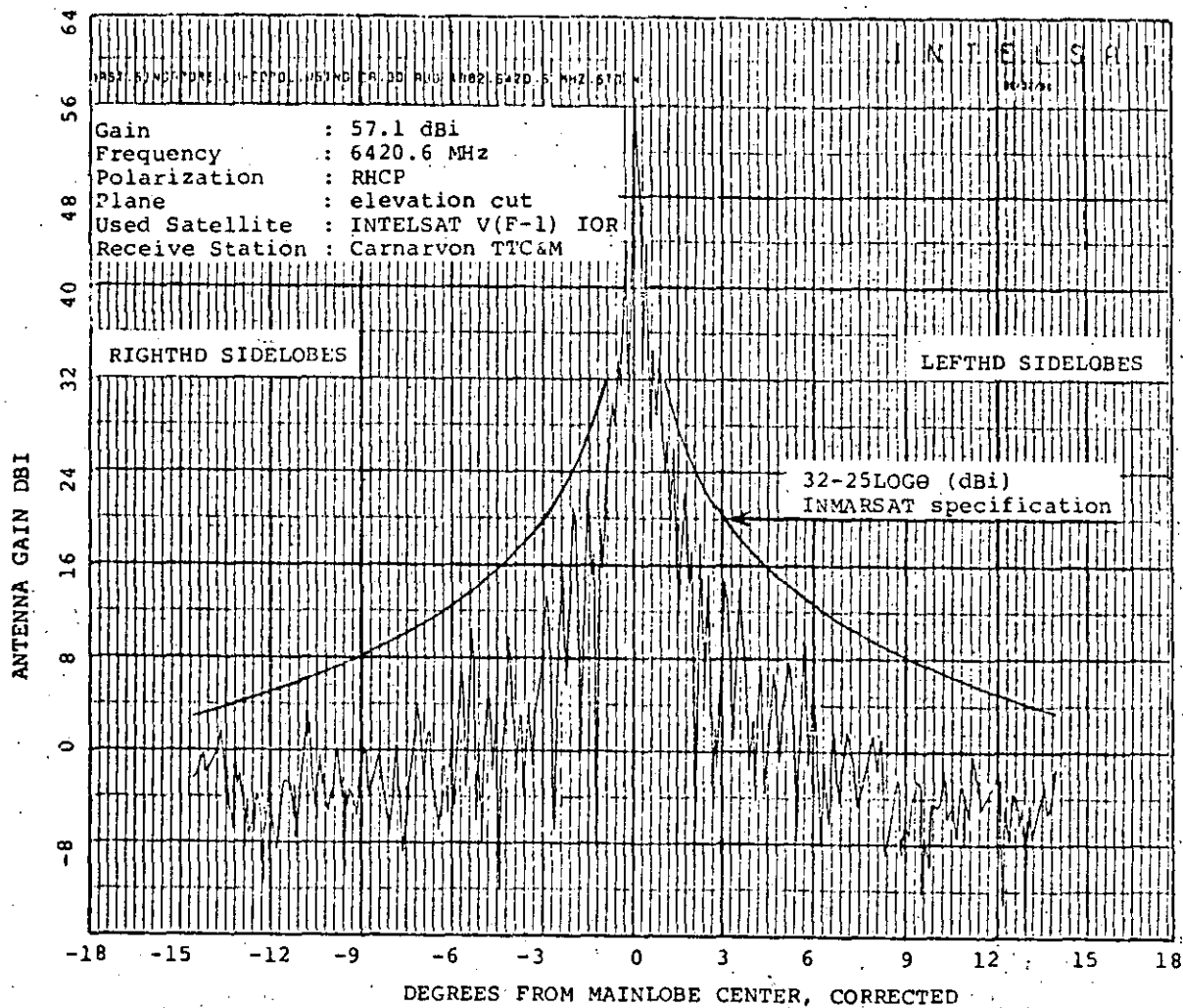
Fig. 8. C-band antenna transmit sidelobe pattern.
