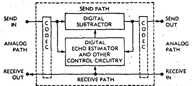
Figure 3d. Type D Echo Canceller
