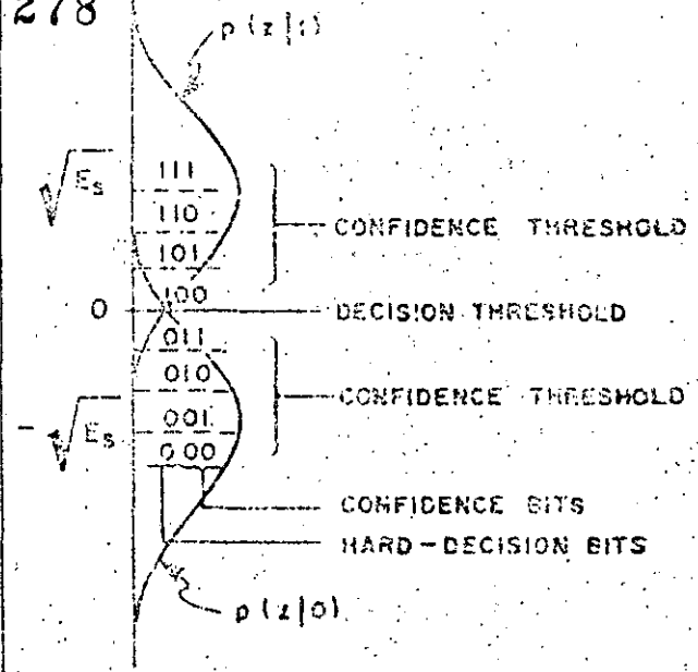
Fig. 4. Three-bit (8-level) soft-decision quantization. p(z|1) and p(z|0) are conditional probability density functions of the matched filter output for a coherent PSK system.
