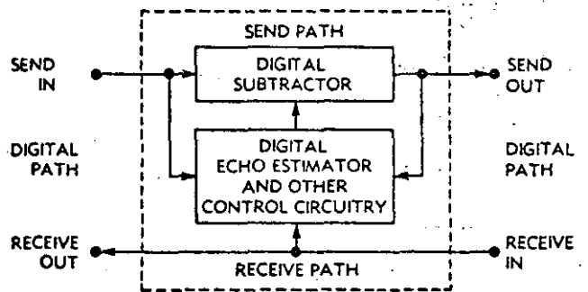
Figure 3c. Type C Echo Canceller
