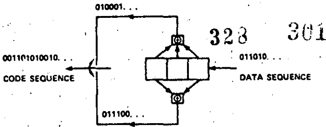
Fig. 1. Convolutional coder for K = 3, n = 2, b = 1 .
