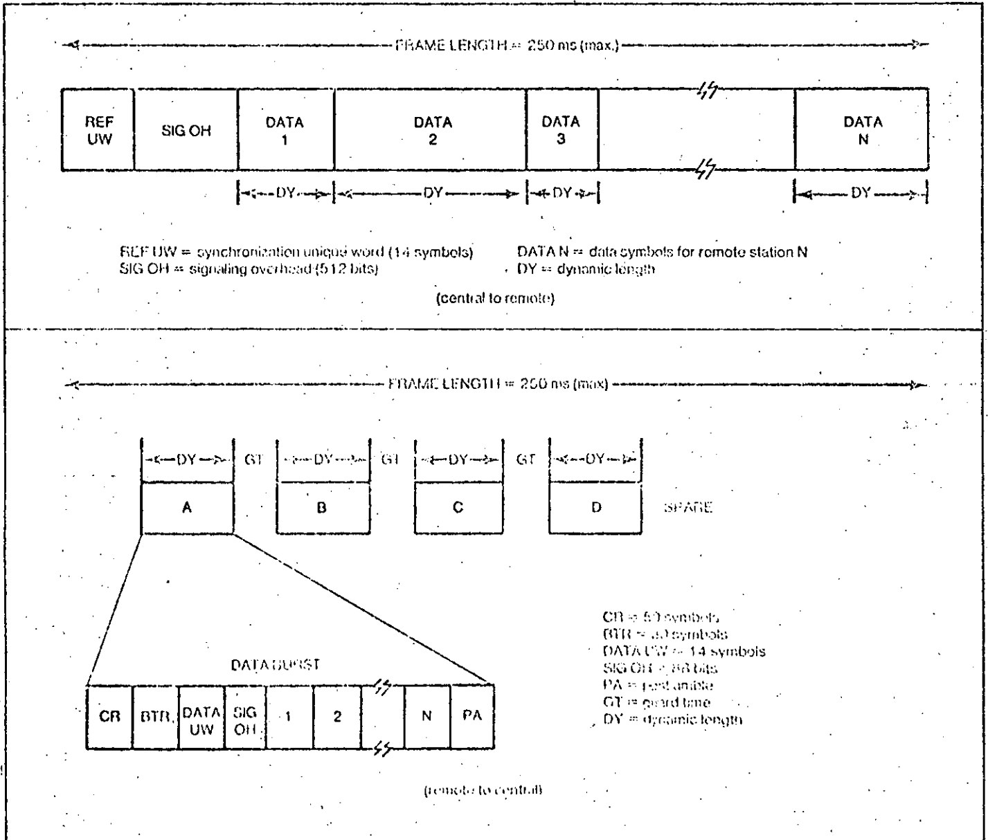
FIGURE 4 Frame Formats (Star Network)
