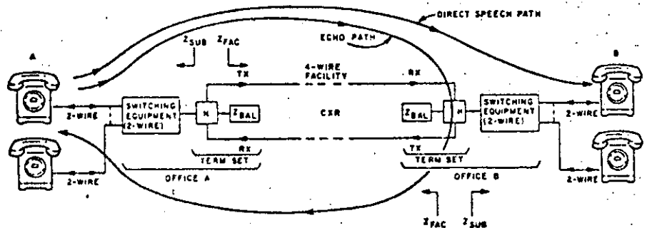
Fig. 2. Illustrating the use of "term sets" at each central office to provide 4-wire capability.
