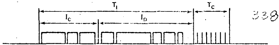
FIG. 4 Priority-oriented demand assignment (PODA).
