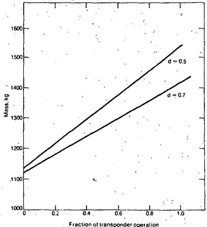
[7] As eclipse capability increases, so does the mass required for batteries and primary power to recharge them. A greater depth of discharge (d) reduces battery mass but not primary power requirements.
