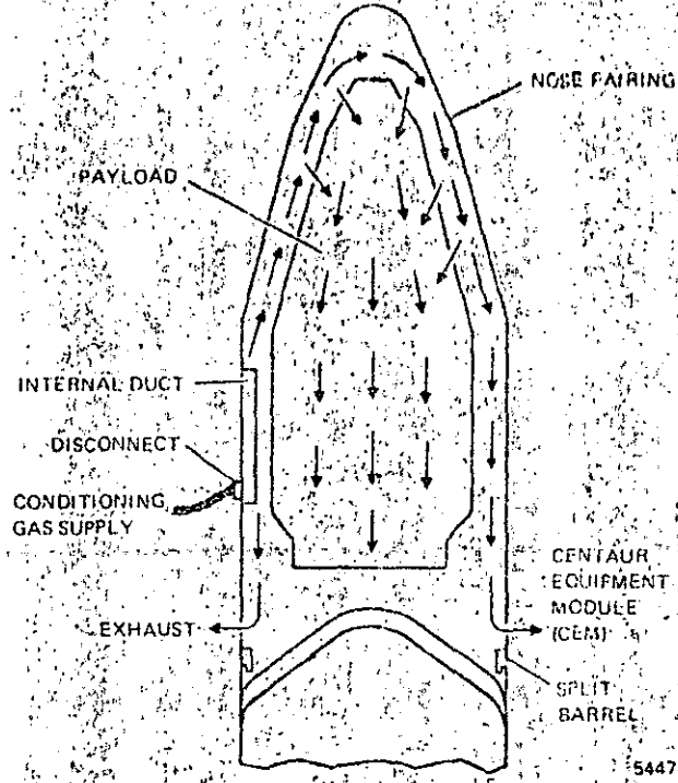
Figure 12. Payload gas conditioning system.
