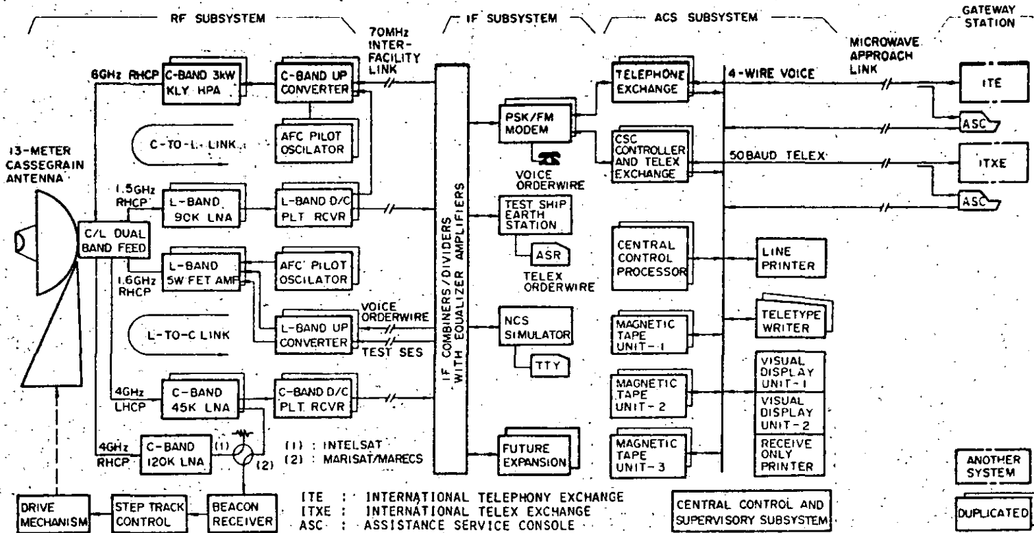
Fig. 2. Block diagram of Singapore coast earth station.
