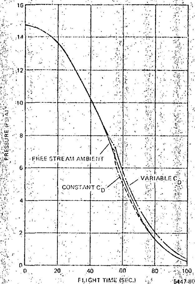
Figure 14. Typical firing pressures.
