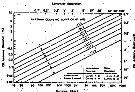
Fig. 2 ISL antenna diameter vs distance.
