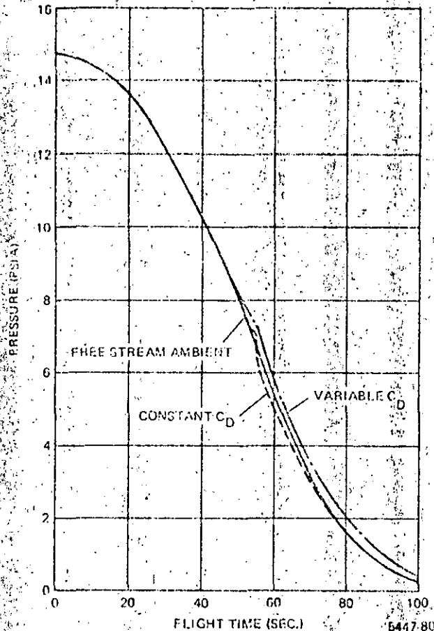
Figure 14. Typical fairing pressures.
