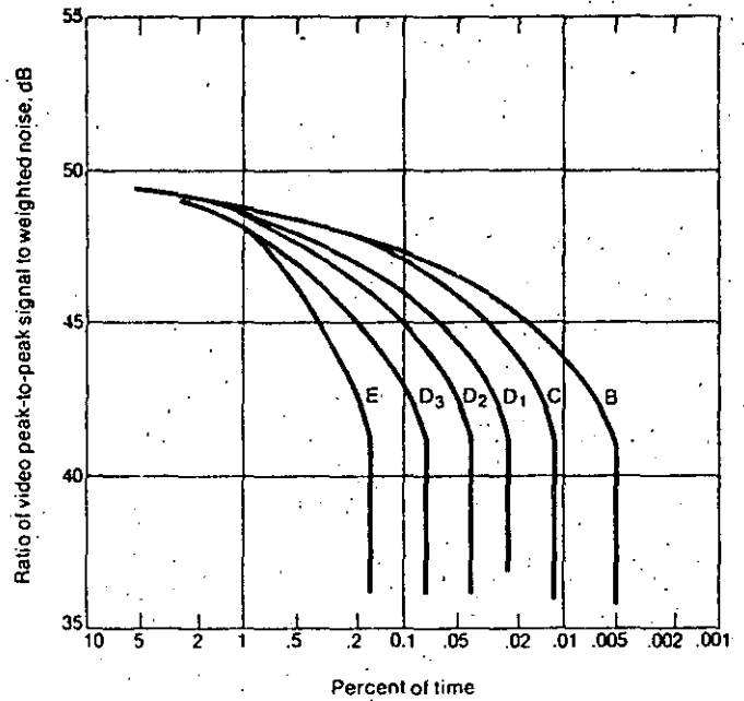
[4] In the 12-GHz band, video performance will degrade during rain. This example shows performance for a system designed to have a signal-to-noise ratio of 50 dB during clear weather. Climate types range from cold and dry areas such as Maine (B) to tropical areas such as Florida and Louisiana (E).
