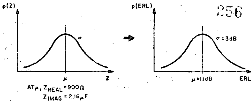
Fig. 3. Probability density functions of subscriber loop impedance and echo return loss.
