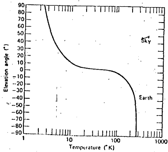
Approximate sky noise variation with antenna elevation angle (4 GHz).
