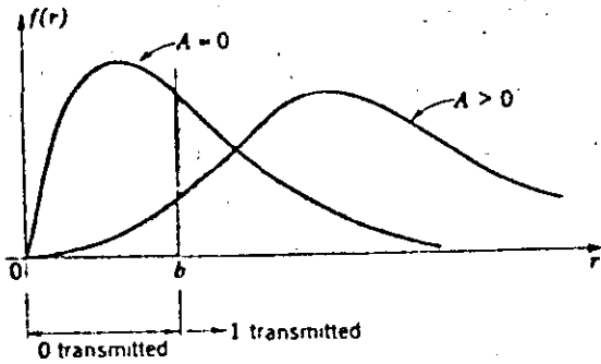
Figure 5-46 Decision regions with envelope-detected OOK signals.
