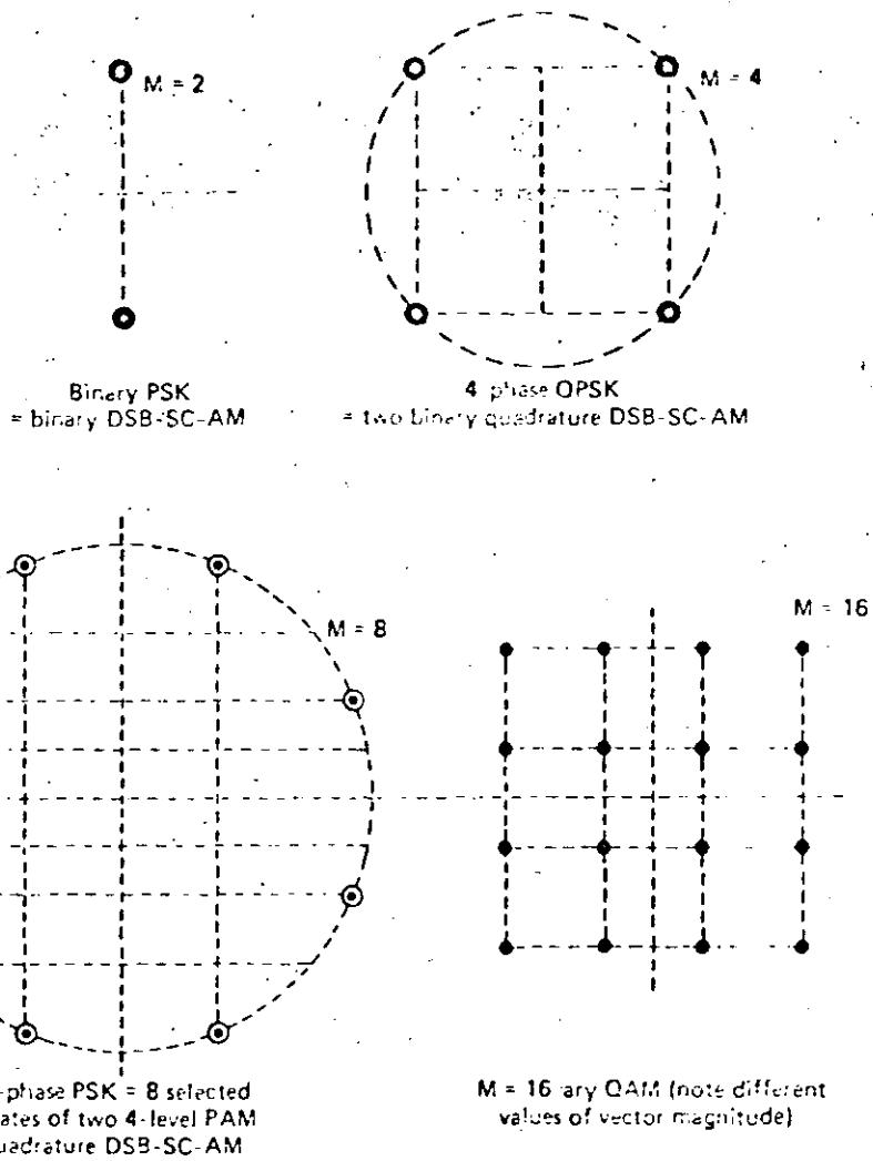
Fig. 6.8. Signal-state space diagrams of M -ary PSK and QAM signals.
