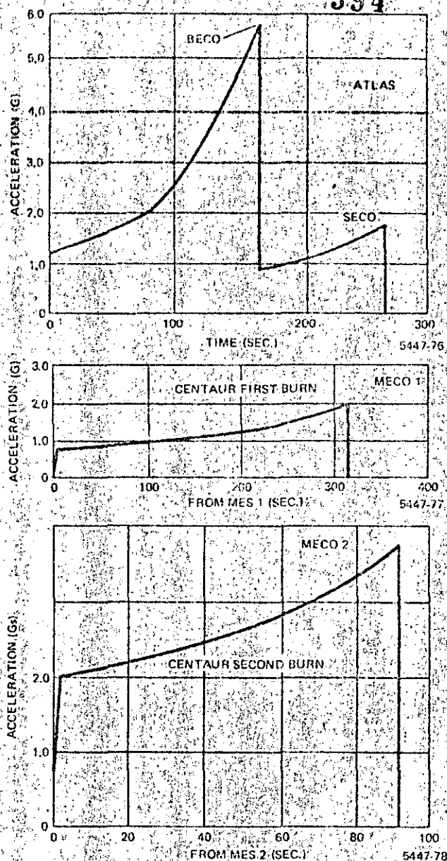
Figure 15. Axial load factors for Atlas/Centaur flight (5,200-lb payload).
