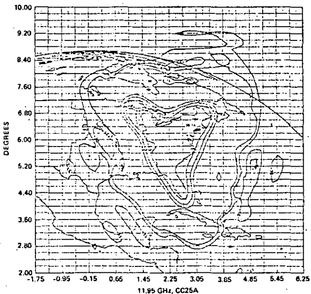
Figure 4. Beam Isolation Contours at 11.95 GHz
