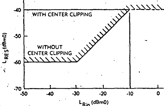
Figure 2. Echo Canceller Steady-State Performance Mask
