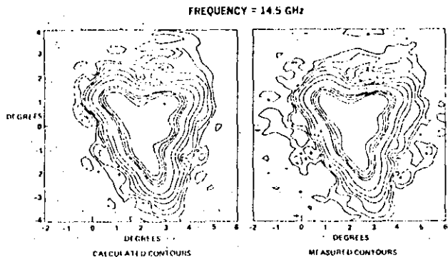
Figure 5. Comparison of Calculated and Measured Gain Contours
