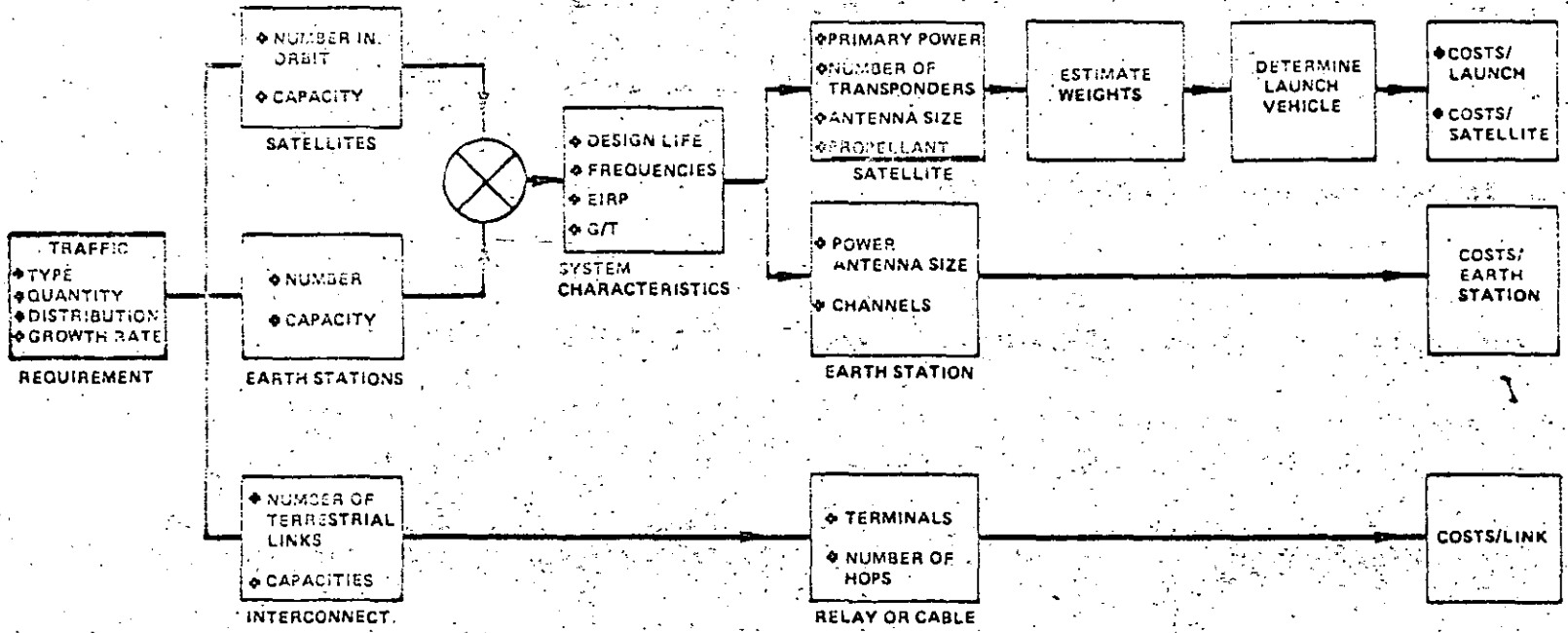
Fig. 1. Cost estimating flow diagram.
