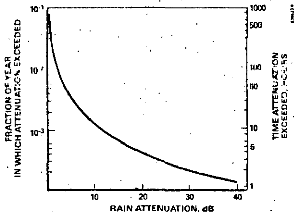
Figure 9. Ka Band Rain Attenuation Data Gathered by Bell Telephone Laboratories
