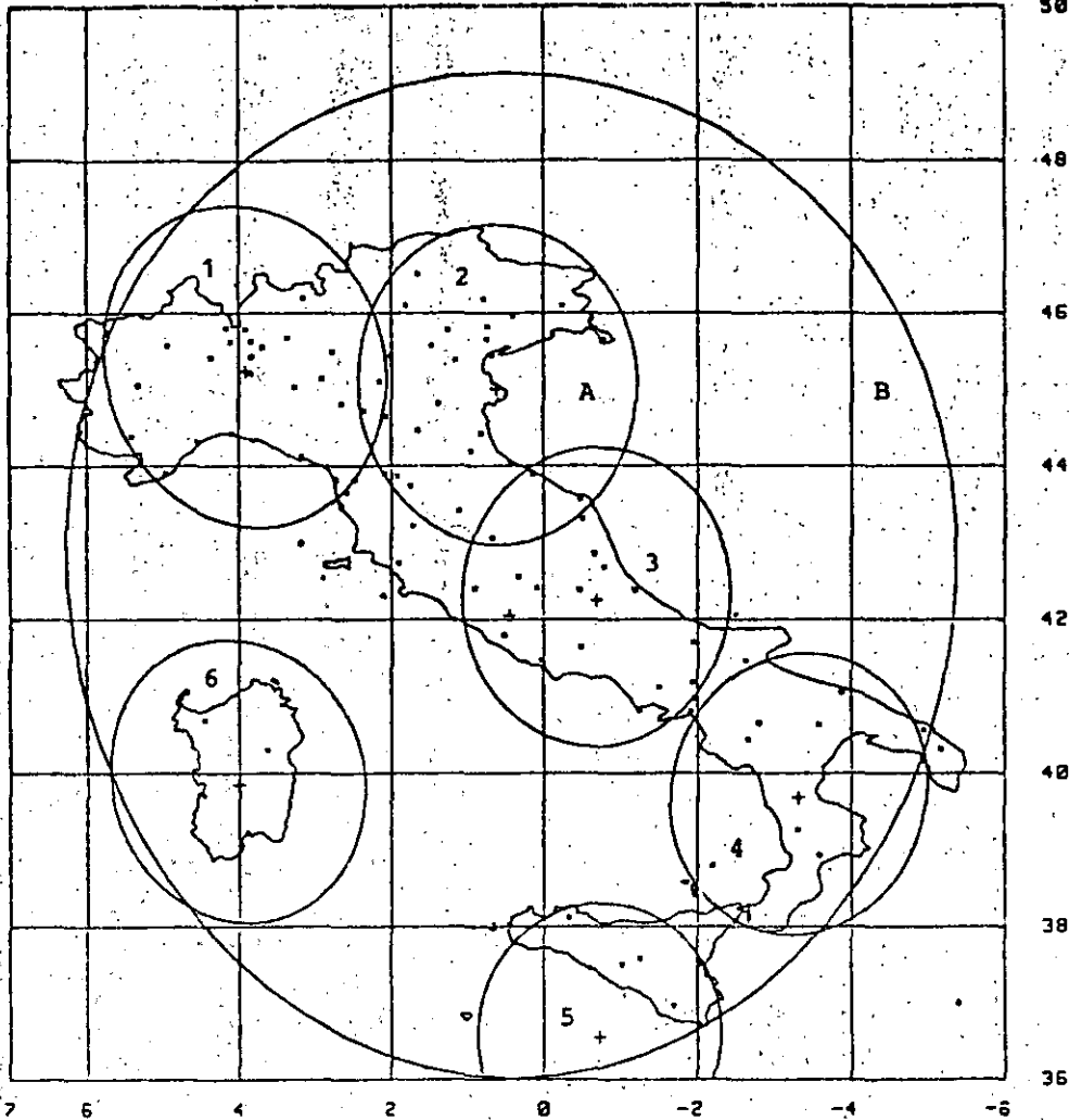
Fig. 1. A Multispot coverage; B. Global coverage.
