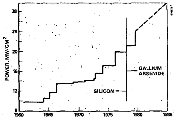
Figure 7. Solar Cell Efficiency Progression
