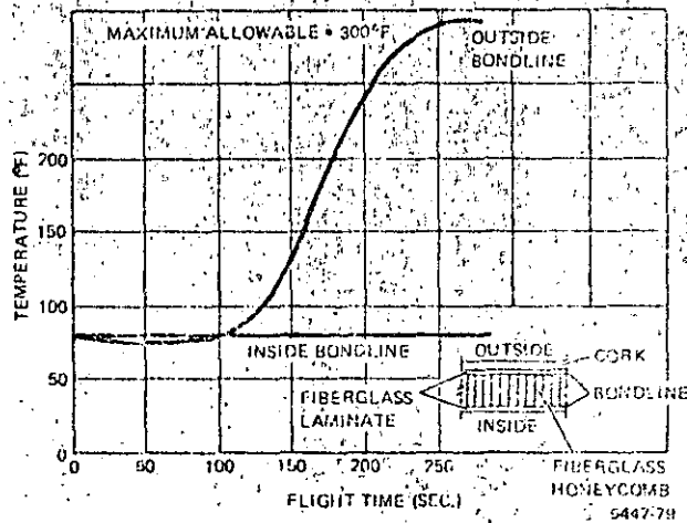
Figure 13. Fairing maximum bondline/temperature predictions (conical portion).
