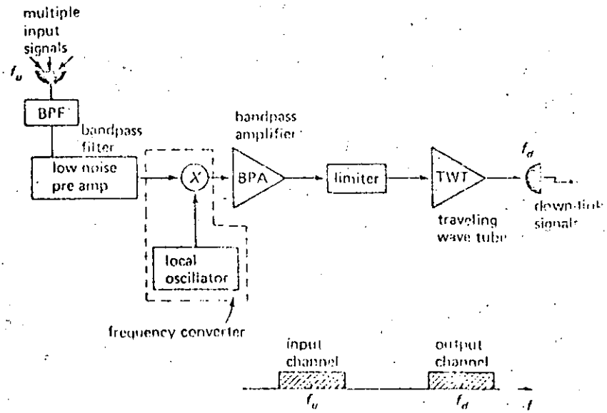
Simplified transponder block diagram showing a single channel transponder
