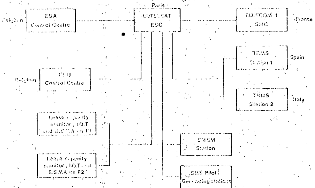
FIG. 4: MONITORING AND CONTROL NETWORK
