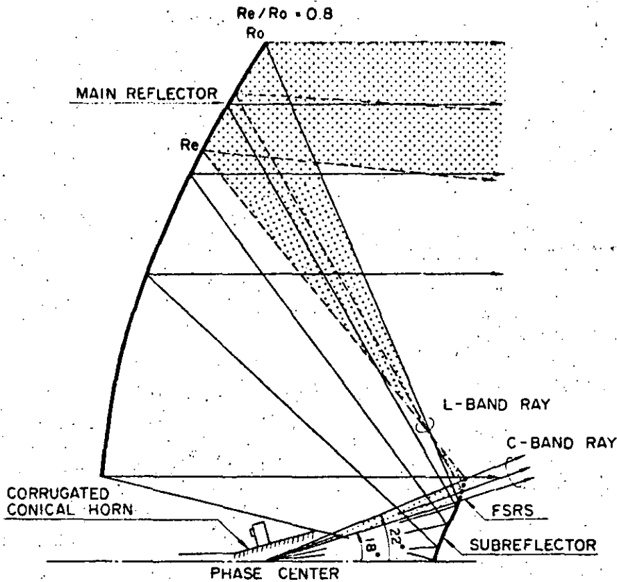
Fig. 4: Cassegrain geometry with RF optics (Main reflector diameter: 13 meter; Subreflector diameter: 1.95 meter; Primary horn diameter: 0.52 meter; Approximate F/D ratio: 0.35).
