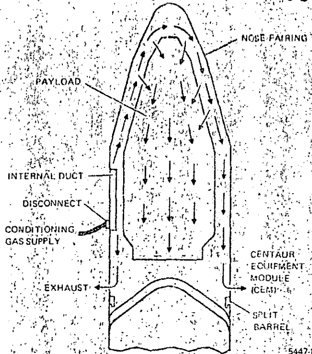
Figure 12. Payload gas conditioning system.
