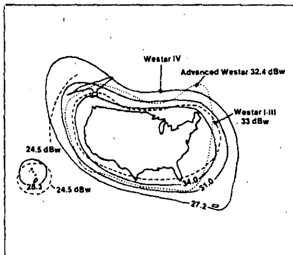
Figure 2. EIRP Coverage at 4 GHz
