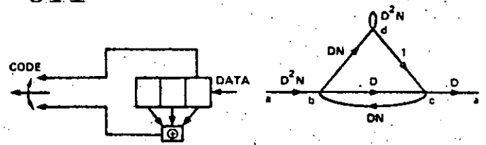
Fig. 13. Systematic convolutional coder for K = 3 and r = 1/2 .
