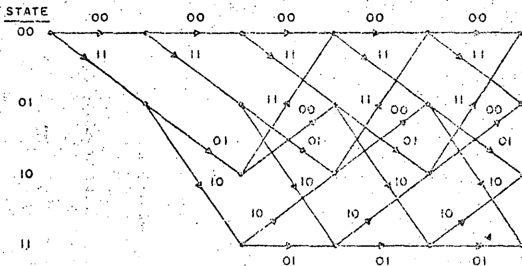
Fig. 10. Trellis for the convolutional encoder of Fig. 2.
