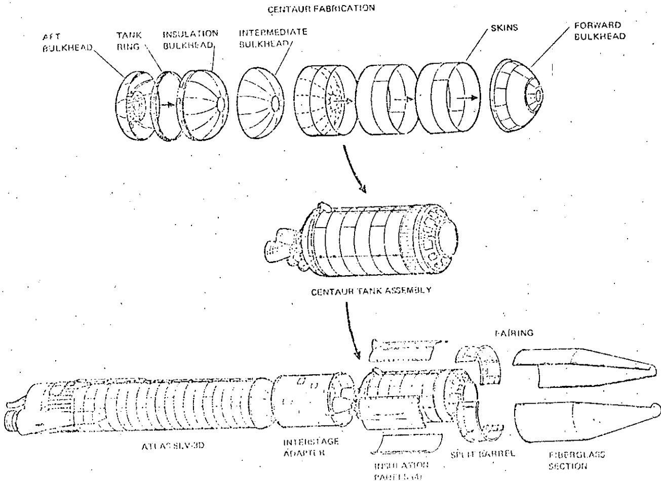
Figure 5. Fabrication sequence.
