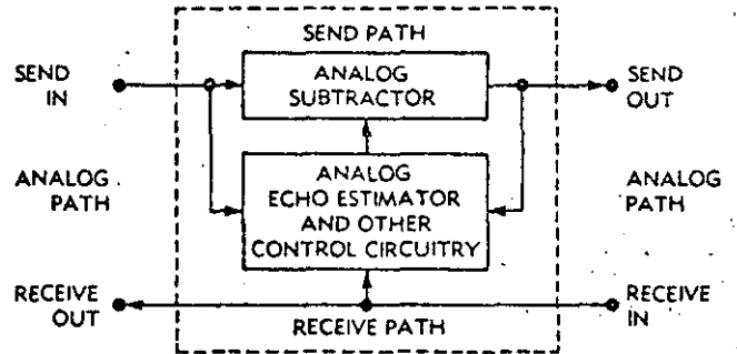
Figure 3b. Type B Echo Canceller
