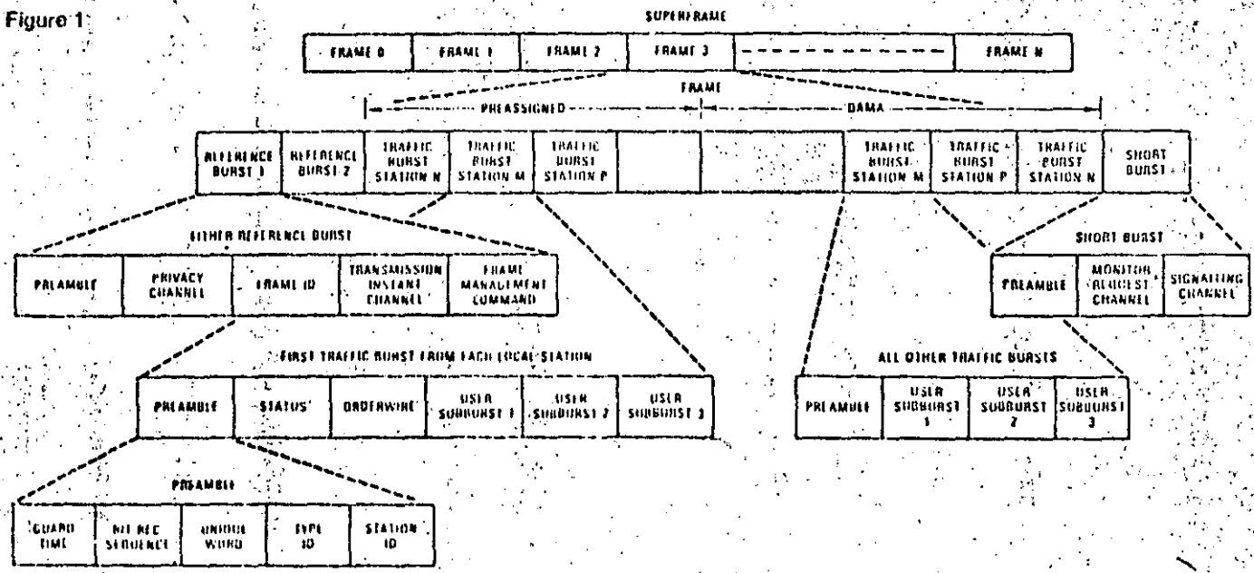
DST-1000 TDMA Frame Structure
