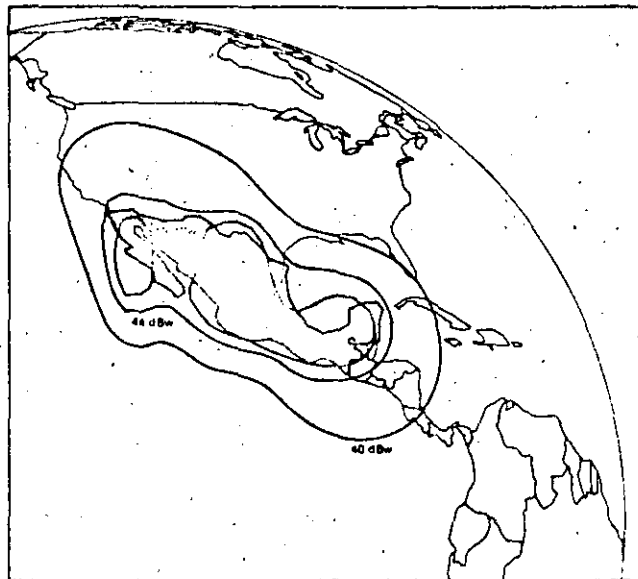
FIGURE 6. MORELOS K BAND COVERAGE (108 MHz, 20 W)
