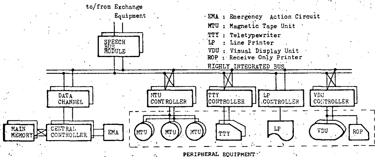
Fig. 13. Block diagram of central control processor.
