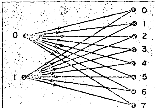
Fig. 5. Eight-level soft quantized DMC produced by a three-bit quantizer on a Gaussian channel.
