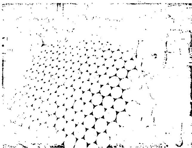
Figure 10. IntelSat VI Transmit Feed Array
