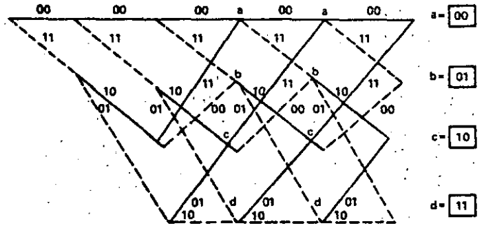
Fig. 3. Trellis-code representation for coder of Fig. 1.
