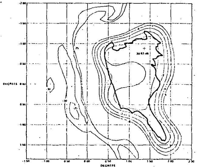
Figure 8. Antenna Directivity Contours Spacecraft at 115°W
