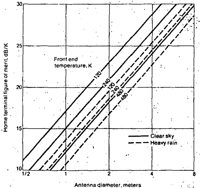
[5] Receiving station G/T is a function of antenna diameter, receiver temperature, and antenna temperature. In heavy rain, the antenna temperature increases from a clear weather value of perhaps 50 K to a maximum value of 290 K (ambient).
