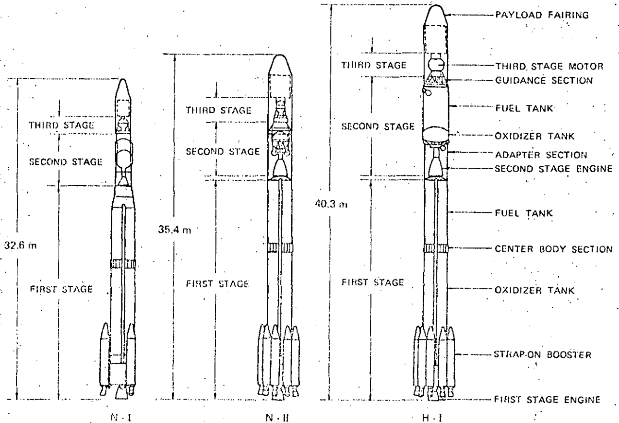
Fig. 2 OUTBOARD PROFILE COMPARISONS
