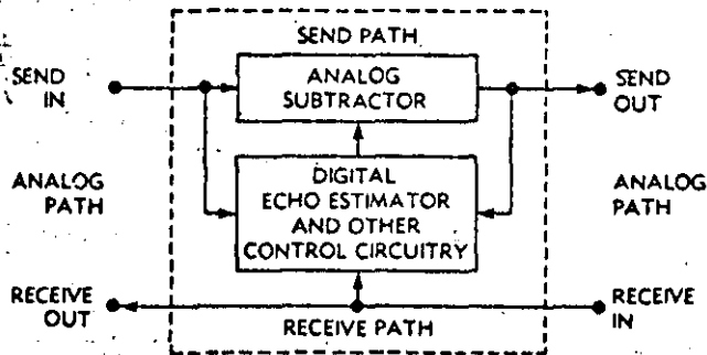
Figure 3a. Type A Echo Canceller
