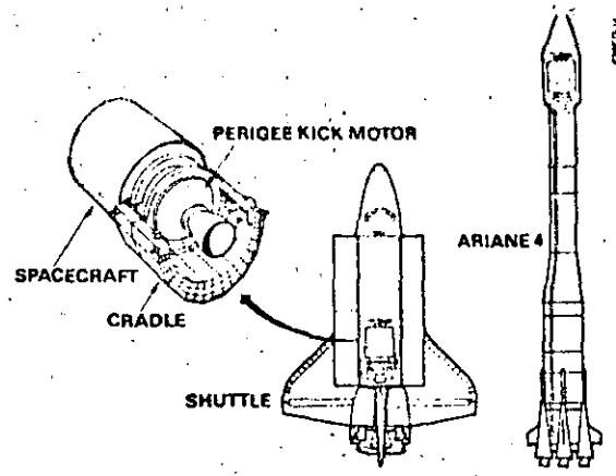
Figure 14. Intelsat VI Shuttle and Ariane 4 Launch Configurations
