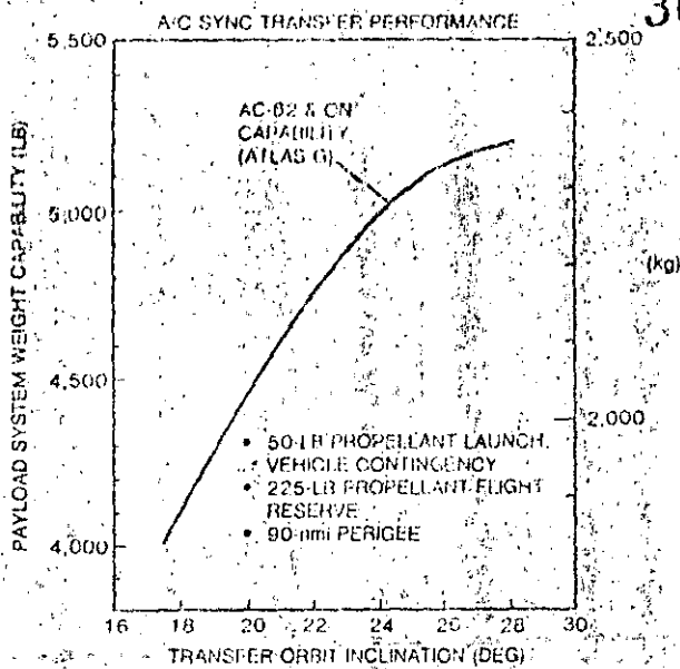
Figure 8. Synchronous transfer performance capability for Atlas/Centaur vehicles.
