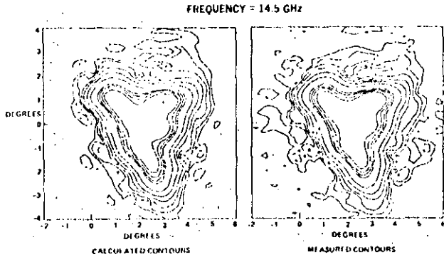
Figure 5. Comparison of Calculated and Measured Gain Contours
