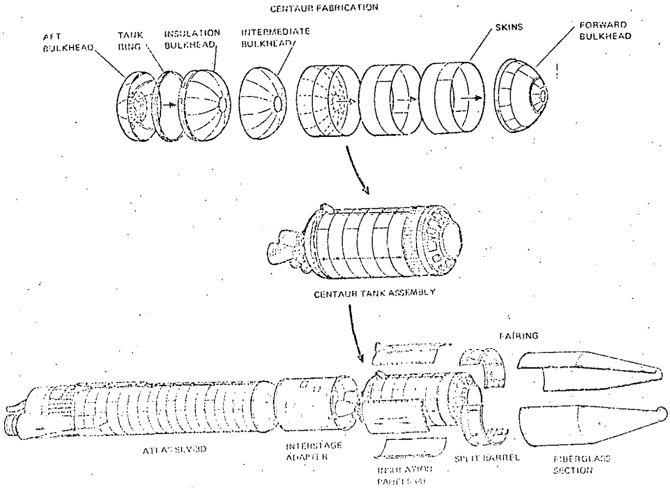
Figure 5. Fabrication sequence.
