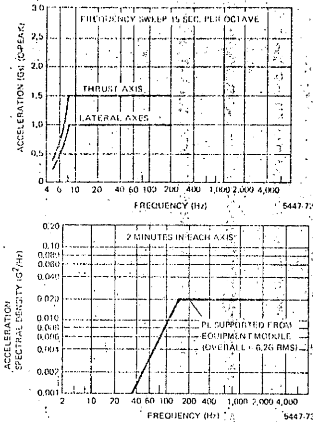
Figure 16. Recommended sinusoidal vibration environment and expected random vibration spectrum.
