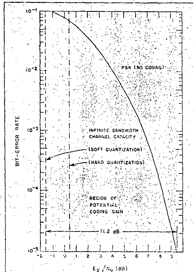
Fig. 6. Performance of uncoded PSK over white Gaussian channel.
