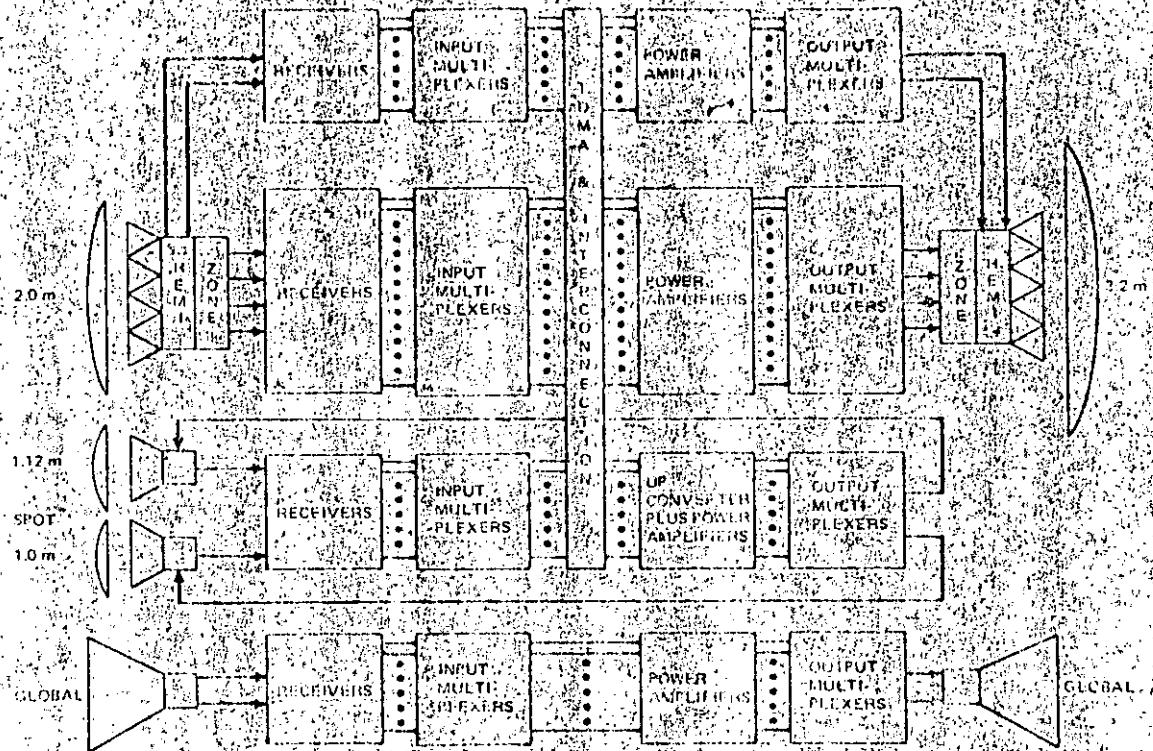
FIGURE 4: COMMUNICATIONS SUBSYSTEM SIMPLIFIED BLOCK DIAGRAM
