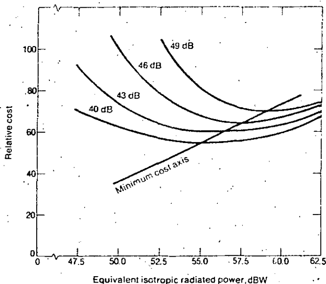
[8] Increasing EIRP raises satellite costs and lowers home receiver costs. The sum of satellite and receiver station costs reaches a minimum that varies with system performance requirements.
