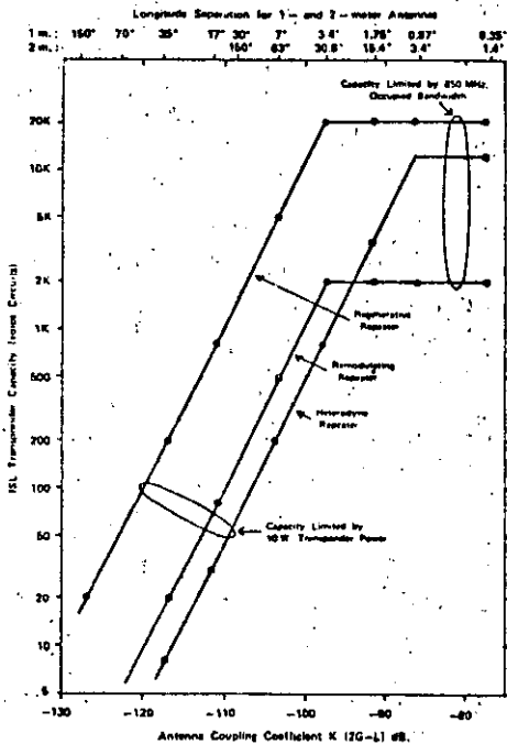
Fig. 1 ISL transponder capacity.
