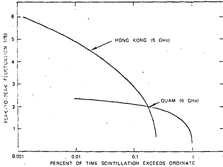
Figure 5. Cumulative Amplitude Distributions at Guam (6 GHz) and Hong Kong (6 GHz)
