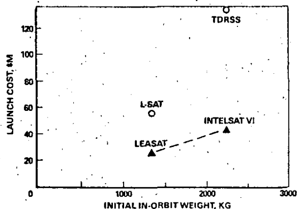
Figure 6. Launch Cost Versus Weight for Various Large New Spacecraft
