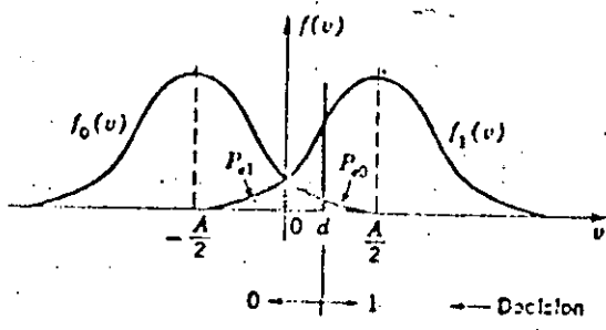
Choice of decision level in binary transmission.
