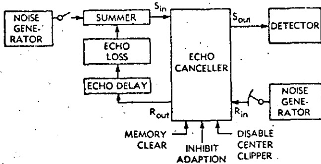
Figure 1. Steady-State Echo Canceller Test Configuration
