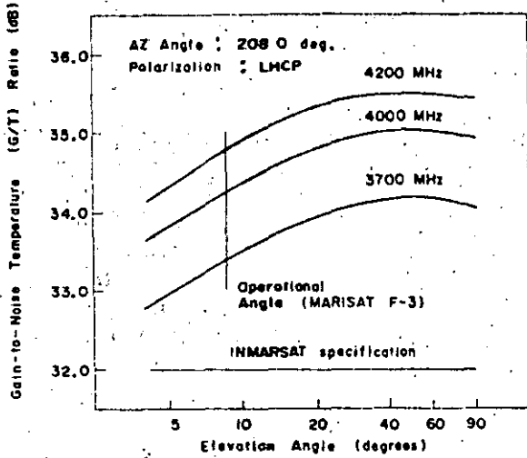
Fig. 10. C-band G/T ratio versus antenna EL angle.
