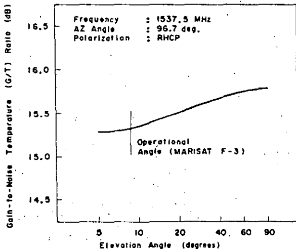
Fig. 11. L-band G/T ratio versus antenna EL angle.
