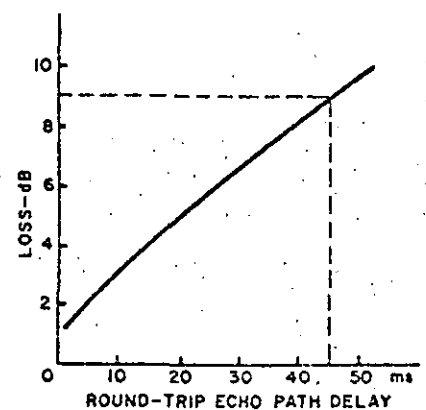
Fig. 4. The amount of loss required to reduce echo level increases with echo path delay.
