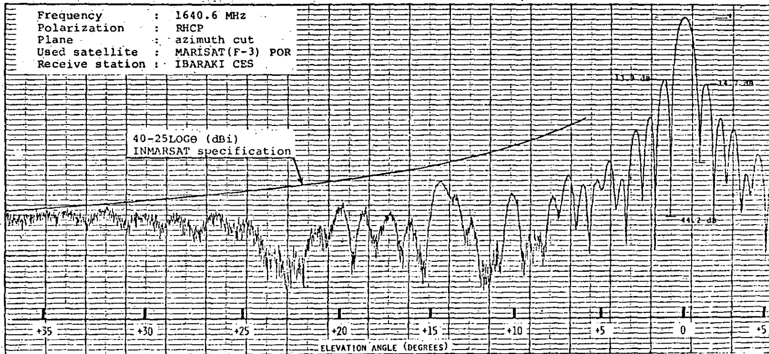
Fig. 9. L-band antenna transmit sidelobe pattern.
