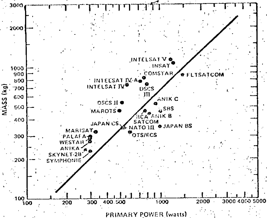
Fig. 2. Satellite on orbit mass vs primary power.
