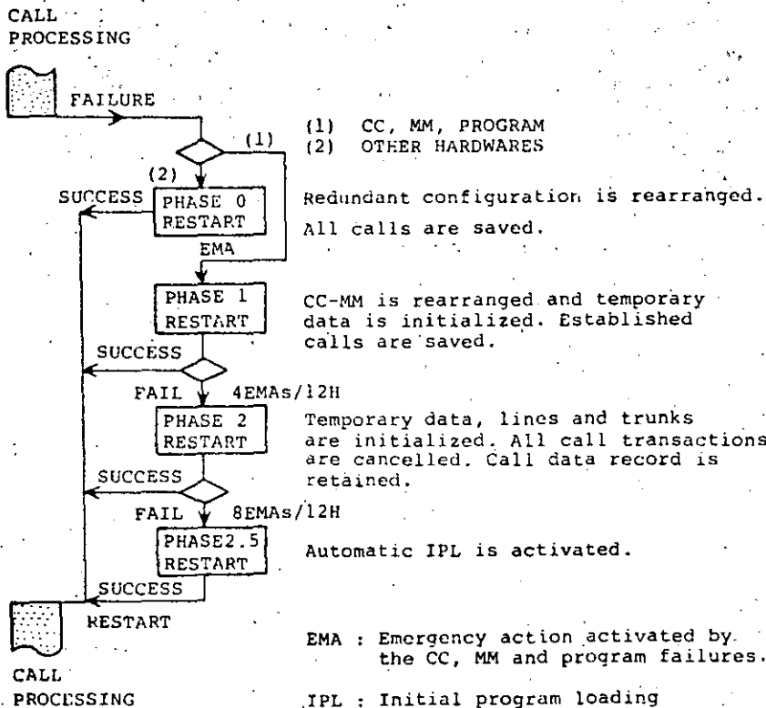
Fig. 15. ACS subsystem restart processes.
