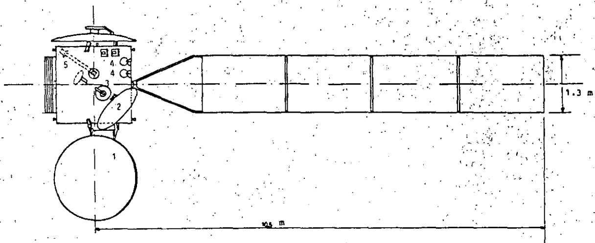
Fig. 2. ITALSAT configuration; 1. Multibeam antenna, 2. Global coverage antenna, 3. Global coverage subreflector, 4. Propagation experiment antennas, 5. TT & C antenna.
