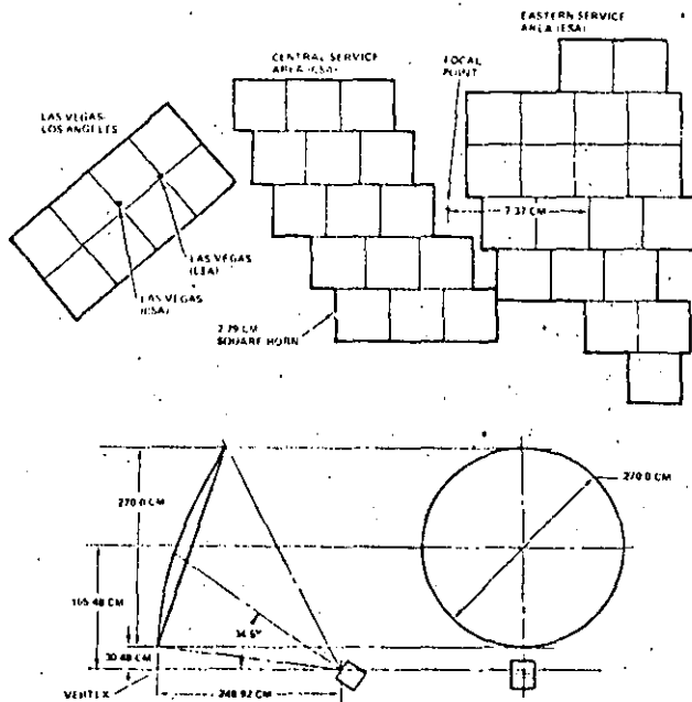
Figure 7. Eastern/Central Satellite Antenna Configuration
