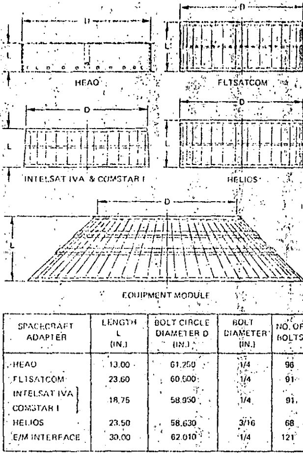
Figure 10. Equipment module interface.
