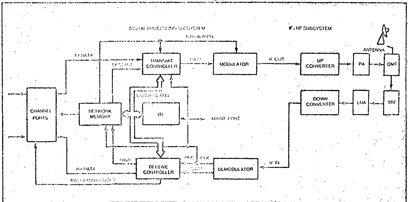
FIGURE 6 DYNACT™ Terminal Block Diagram (non-redundant)
