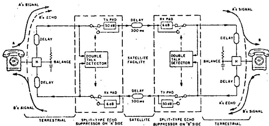
Fig. 5. A split echo suppressor connects the transmit speech path when one subscriber is talking but disconnects it when the other subscriber is talking (since this path is now the undesirable echo path)."
