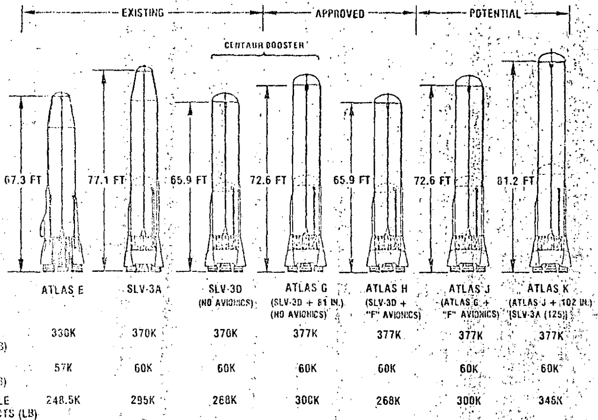
Figure 2. Atlas vehicle family.
