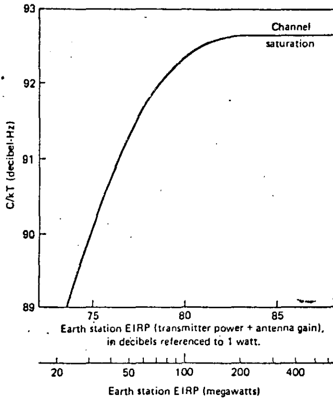
Figure 7.1 C/kT for a typical American domestic satellite.
