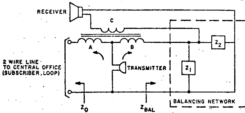
Fig. 1. The transformer in the typical telephone set permits the same pair of wires to carry both the transmitted and received signals.
