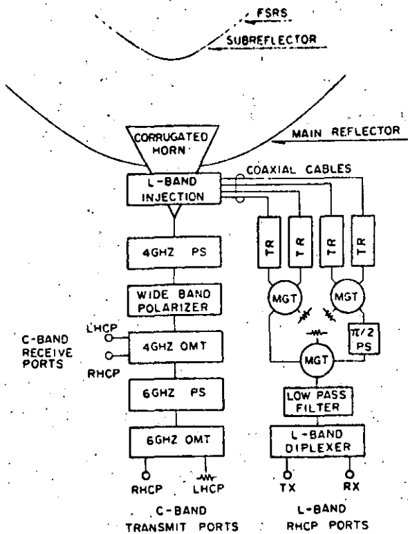
Fig. 5. Antenna feed configuration (PS: Phase shifter; OMT: Orthomode transducer; TR: Coaxial-to-waveguide transition; MGT: Magic T).
