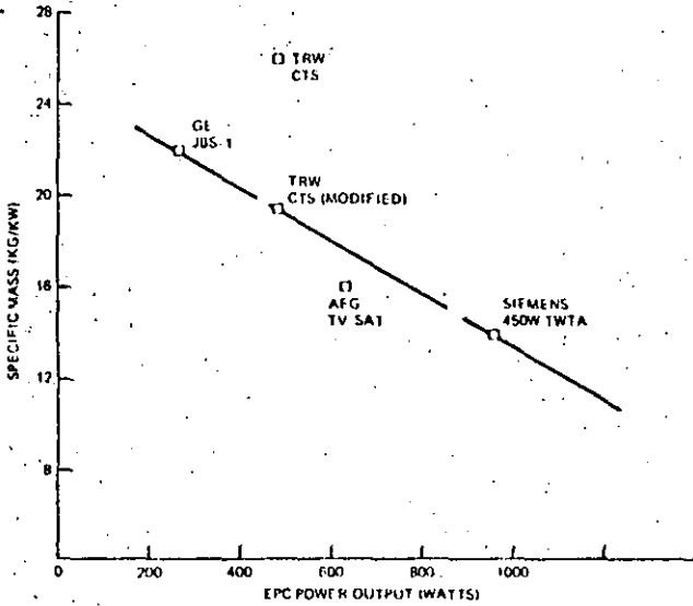
Figure 10. TWT Electronic Power Conditioner (EPC) Specific Mass
