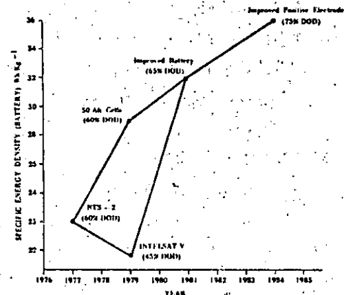
Fig. 10 Nickel-hydrogen battery design objectives.
