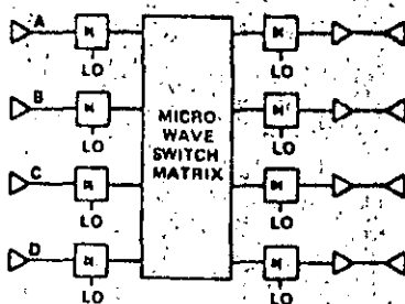
Fig. 5. SS-TDMA block schematic.
