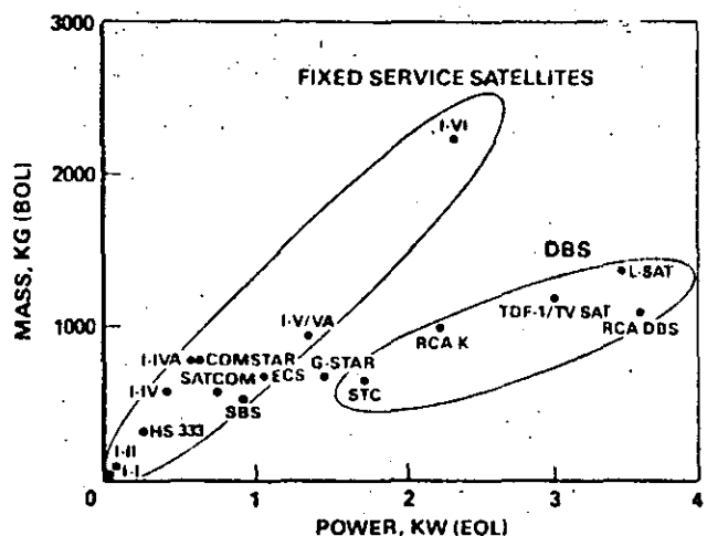
Figure 2. Weight and Power Relationship of Direct Broadcast and Fixed Service Satellites
