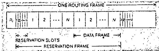
Fig. 2. R-TDMA channel.
