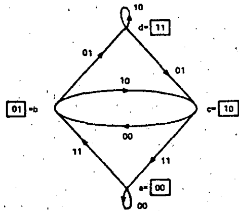
Fig. 4. State-diagram representation for coder of Fig. 1.
