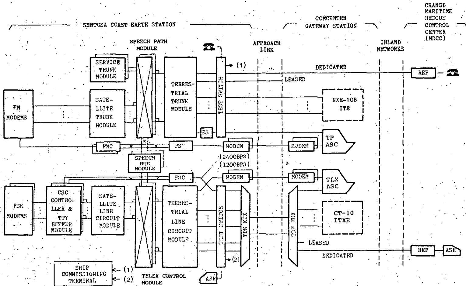
Fig. 14. Exchange equipment configuration.
