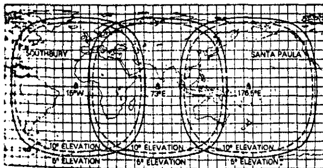
Figure 8. MARISAT Coverage (from COMSAT Technical Review, Vol. 7, No. 2, Fall 1977)
