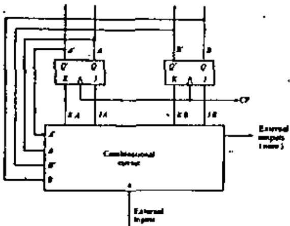
Figure 6-22 Block diagram of sequential circuit
