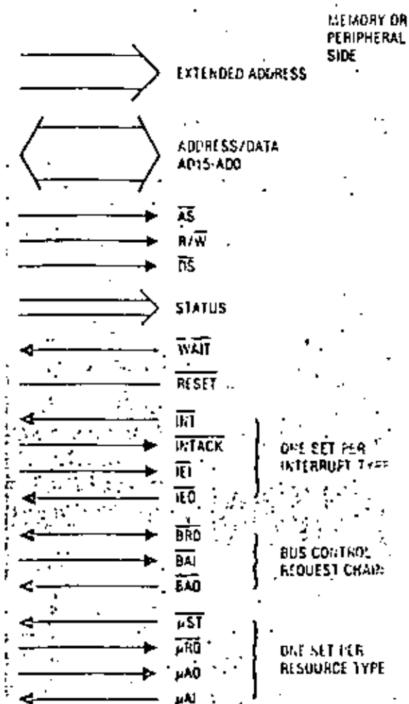
Figure 7. Z-bus signals.
