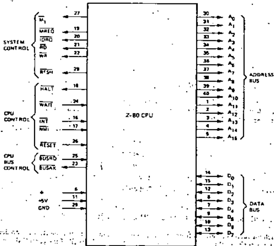
Z-80 PIN CONFIGURATION FIGURE 3.0-1
