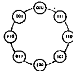
Figure 6-23 State diagram of a 3-bit binary counter
