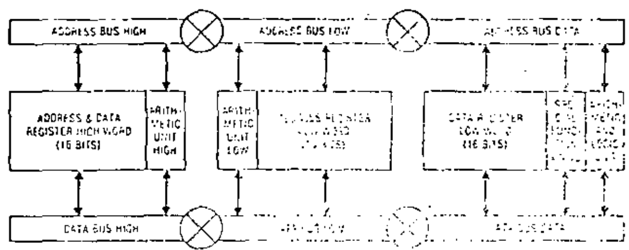
Figure 8 MC68000 execution unit configuration
