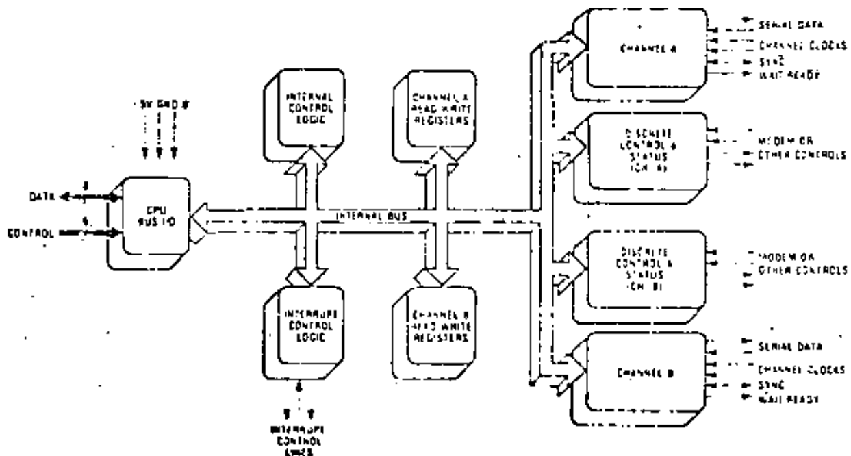
Z80-SIO BLOCK DIAGRAM
