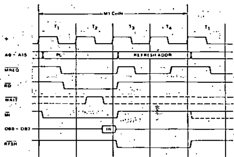
INSTRUCTION OF CODE FETCH FIGURE 4.0-1
