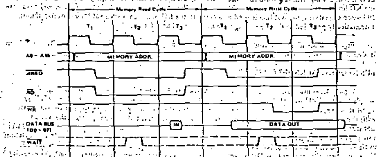
MEMORY READ OR WRITE CYCLES. FIGURE 4.0-2
