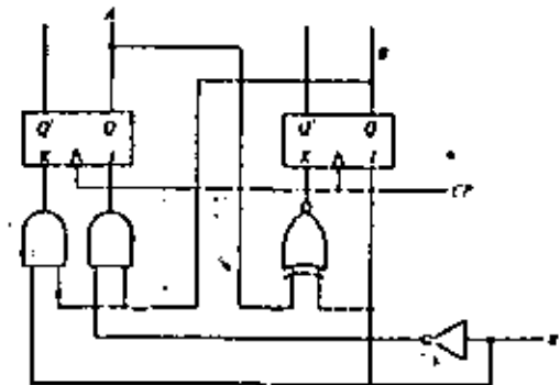
Figure 6-20 Logic diagram of sequential circuit
