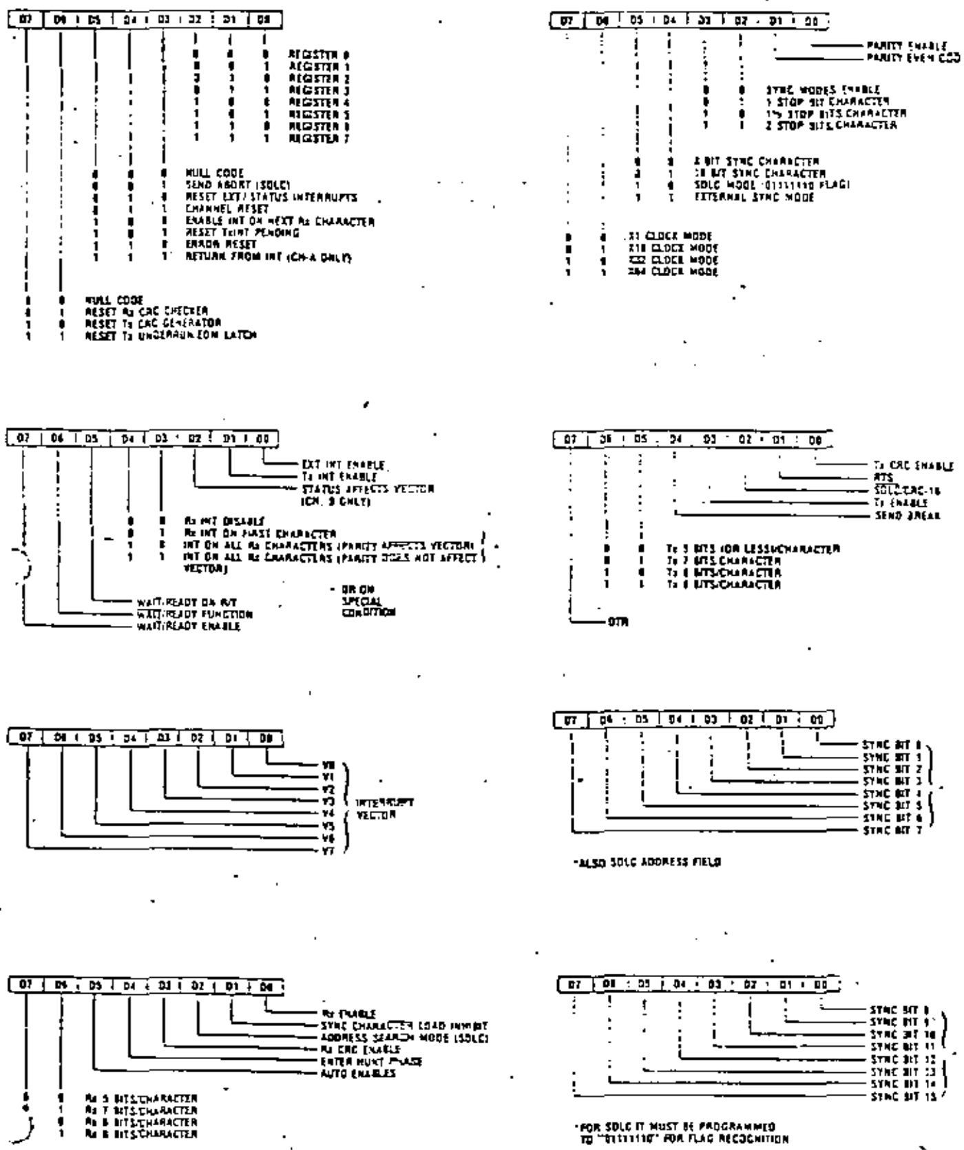
Figure 7. Write Register Bit Functions
