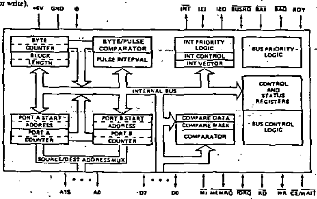
DMA Internal Block Diagram
