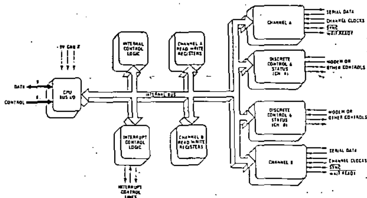
Figure 1. Z80-SIO Block Diagram
