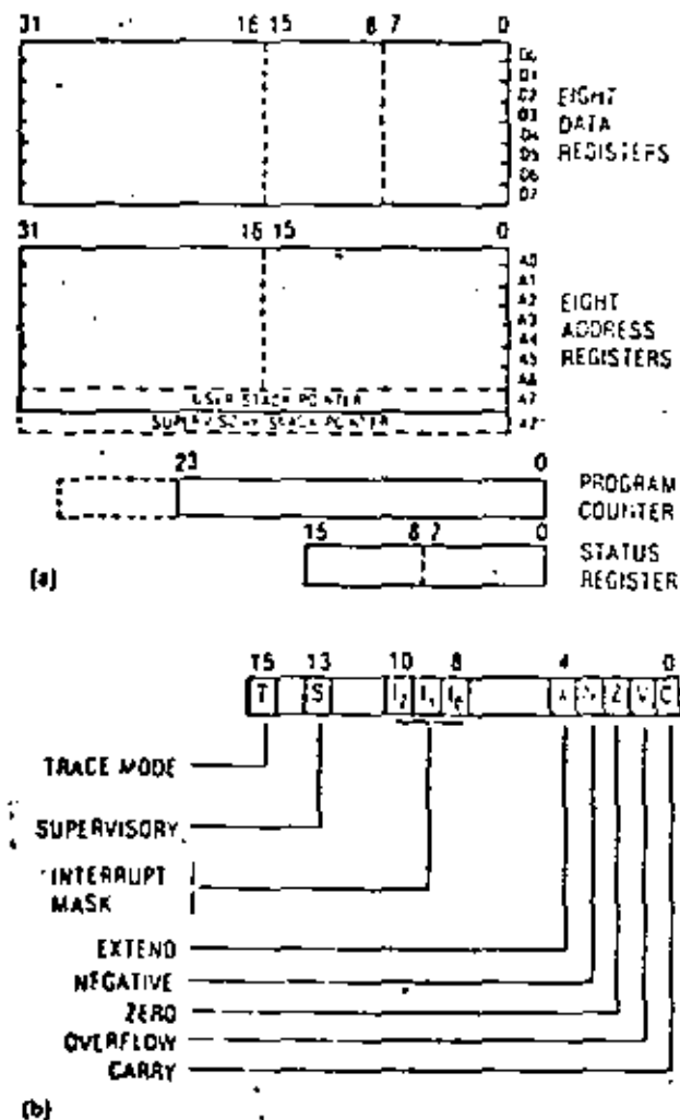
Figure 2. MC68000 programming model (a) and internal structure of status register (b).
