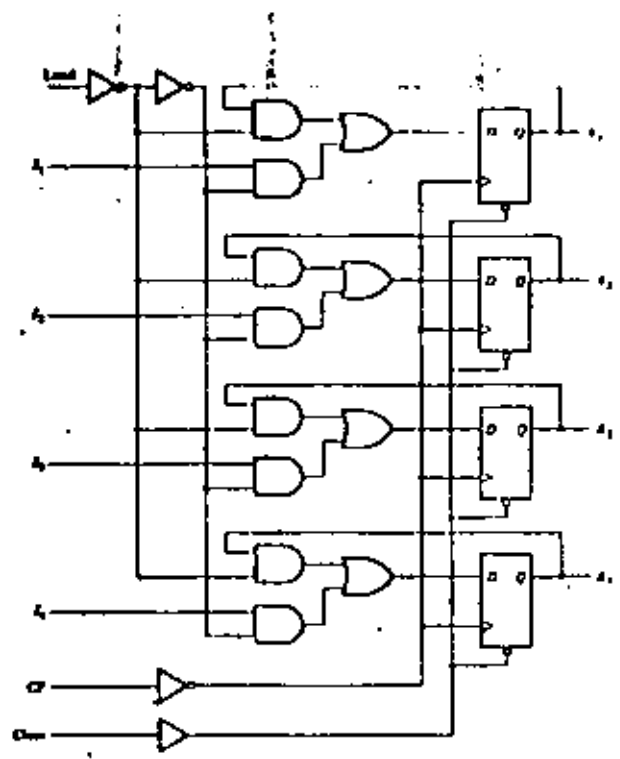
Figure 7-2 Register with parallel load using D flip-flops
