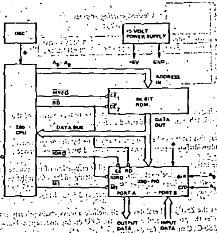
FIGURE 9.0-1 MINIMUM Z80 COMPUTER SYSTEM
