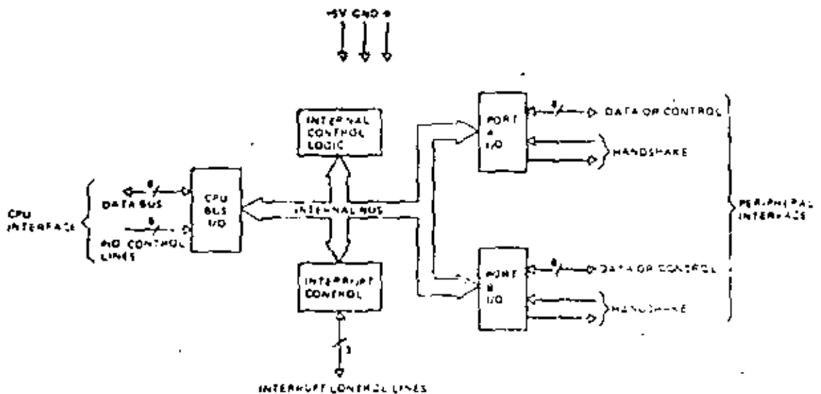
FIGURE 2.0-1 PIO BLOCK DIAGRAM
