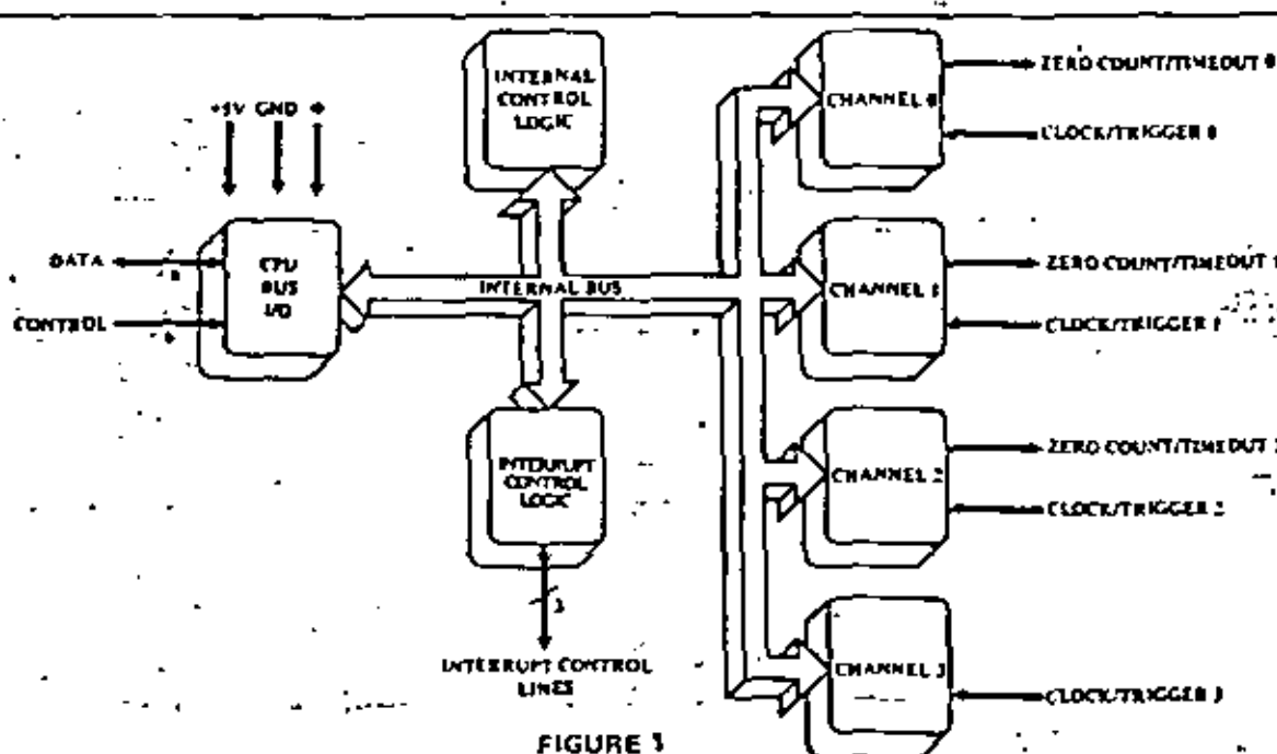
FIGURE 1 CTC BLOCK DIAGRAM
