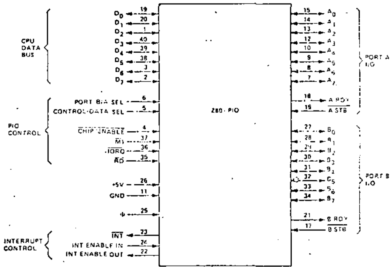
FIGURE 3 0 1 PIO PIN CONFIGURATION
