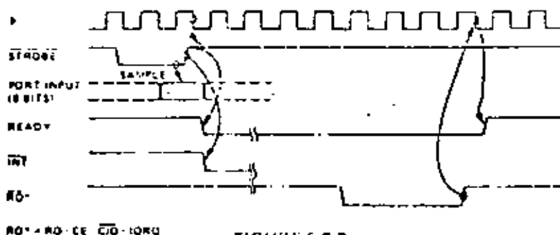
FIGURE 5.0-2 MODE 1 (INPUT) TIMING
