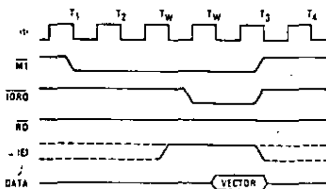
Figure 8c. Interrupt Acknowledge Cycle
