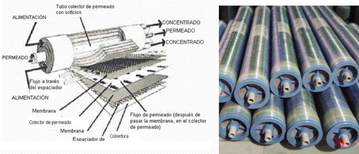
Figura 2-5 Membrana enrollada
