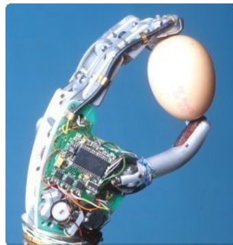
a) Cyberhand [5]
