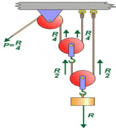
Figura 5.14 Polipasto factorial
