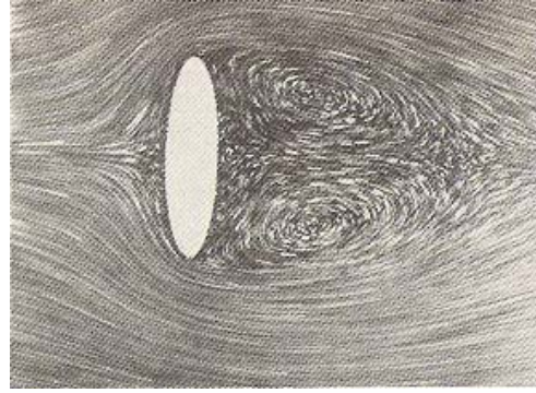
Fig. 3.69.- wb/v = 10.0
