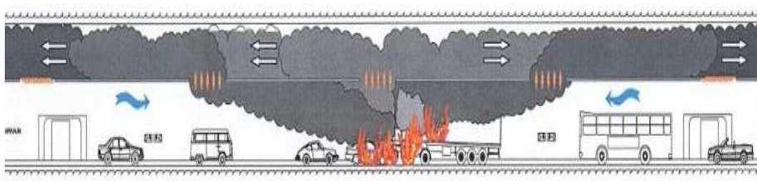
Figure 2.11 Scheme of the new ventilation system in the St. Gotthard tunnel (Lombardi engineering LTD.)
