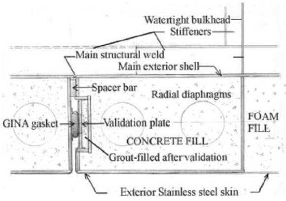
Figure 1.33 Rigid joint proposed by Grantz in 2003.
