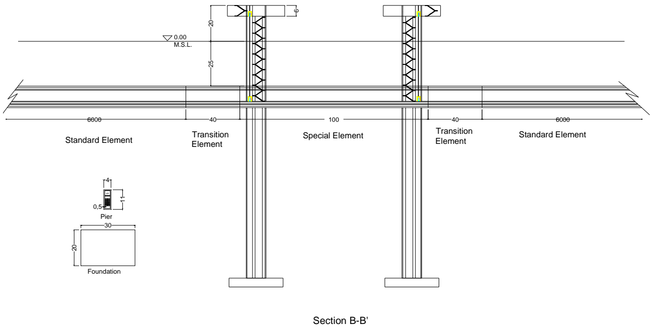
Figure 4.41 Longitudinal view of the towers and platforms (measures in meters)
