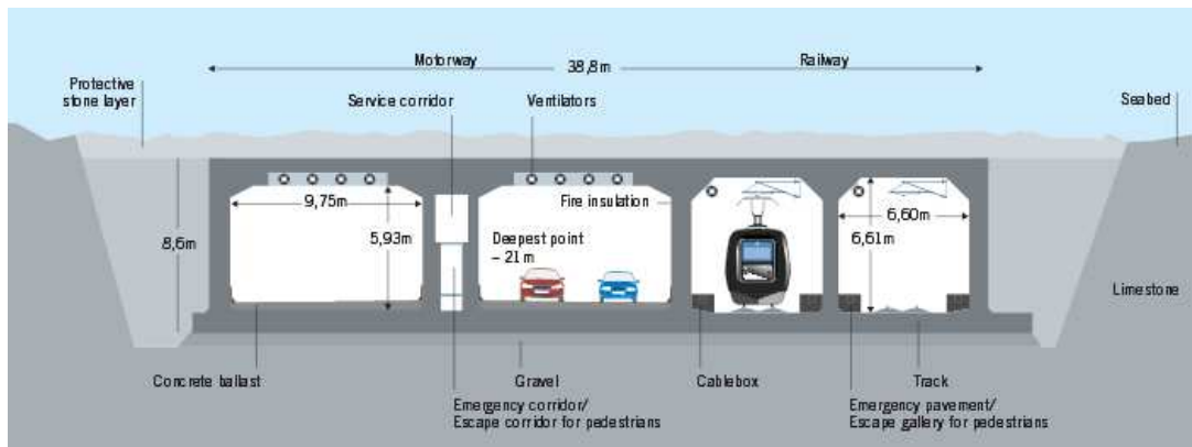
Figure 2.19 Cross section of Oresund Tunnel (Fermen, 2006)
