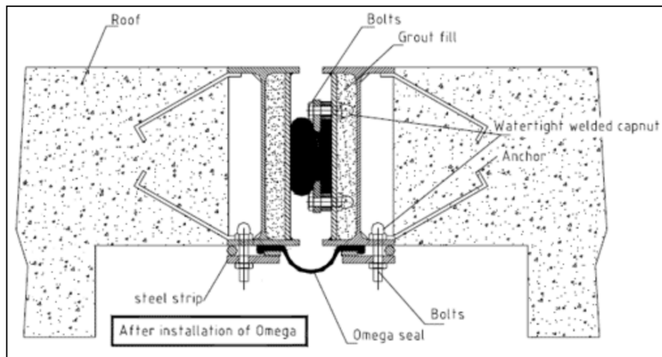
Figure 4.31 Details of the inter-modular joints (Bistoon Baspar LTD, continuation)
