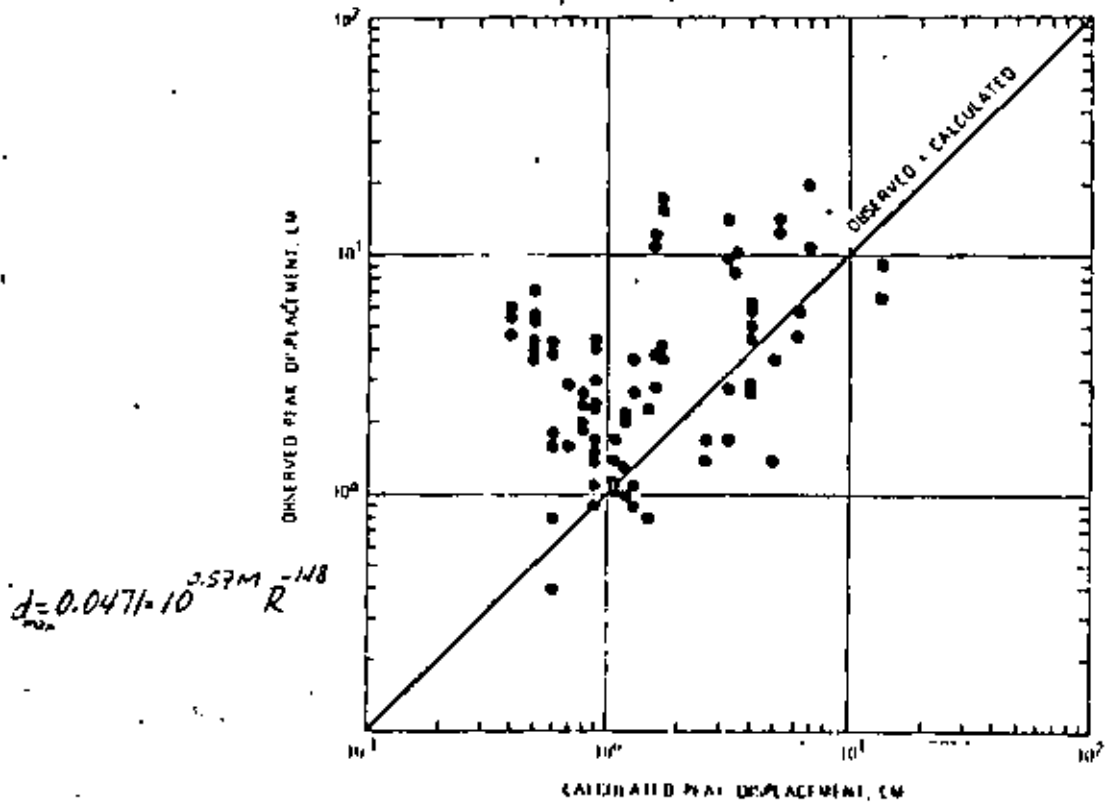
FIG. 9. Comparison between peak displacements derived from the CALTECH strong-motion accelerograms and corresponding calculations using equation (8).
