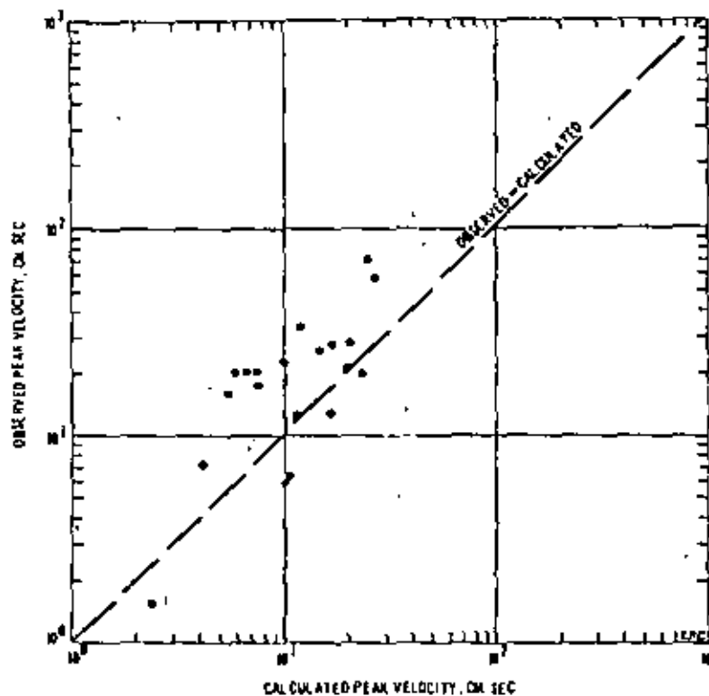
FIG. 7. Comparison between 20 recorded peak velocities (Ambrascys, 1969) and corresponding calculations using equation (7).
