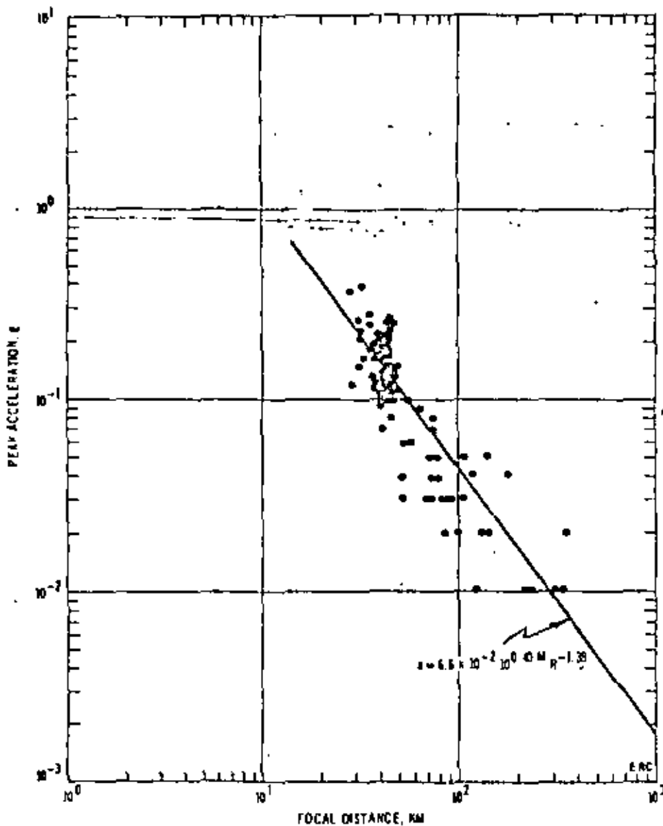
FIG. 1. Comparison between peak acceleration versus distance observed from San Fernando earthquake and calculated from equation (6).
