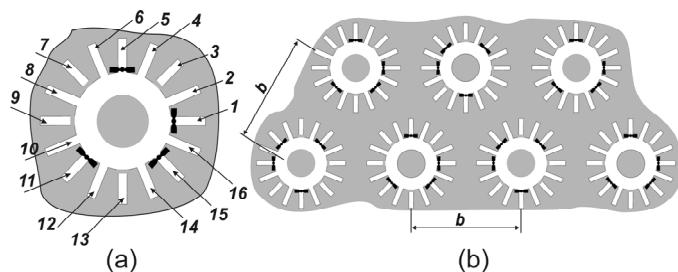
Fig. 4 (a) The third two-bit element with 16 stubs (b) Elements arranged at the nodes of triangular equilateral grid
