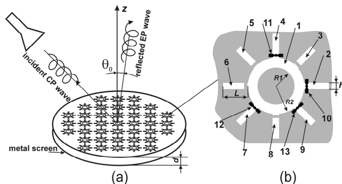
Fig.1 (a) Spiraphase-type reflectarray (b) Two-bit element of spiraphase-type reflectarray.
