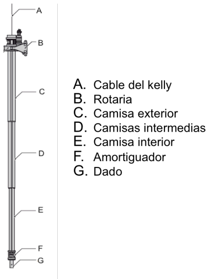
Fig.15. Partes de barretón o kelly (Hudelmaier and Küfner 2009)
