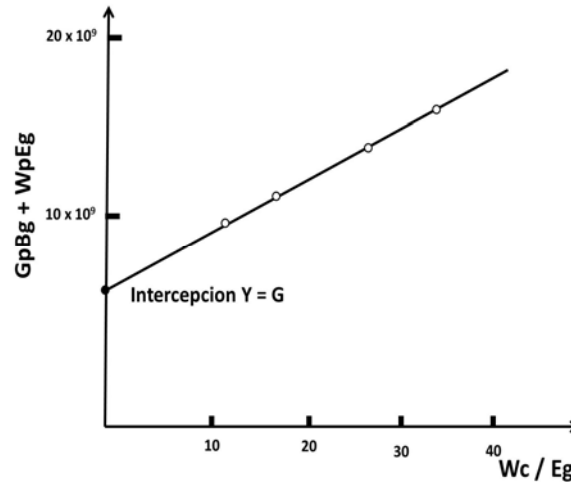
Fig. 3.8. G_p B_g + W_p / E_g Vs. W_c / E_g . 15
