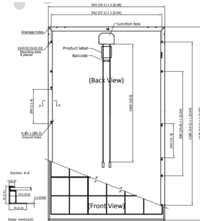
Figura 52. Paneles fotovoltaicos 250 polycrystalline solar module Recuperado de: http://dansolar.dk/wp-content/uploads/2012/09/Suntech-STP250-poly.pdf
