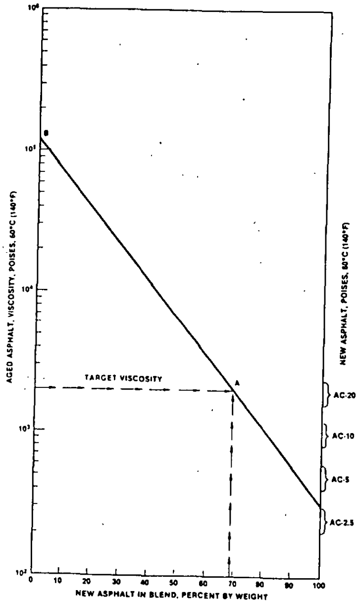
Figure III-2—Blending chart for reclaimed asphalt and new asphalt cements: Example 1.
