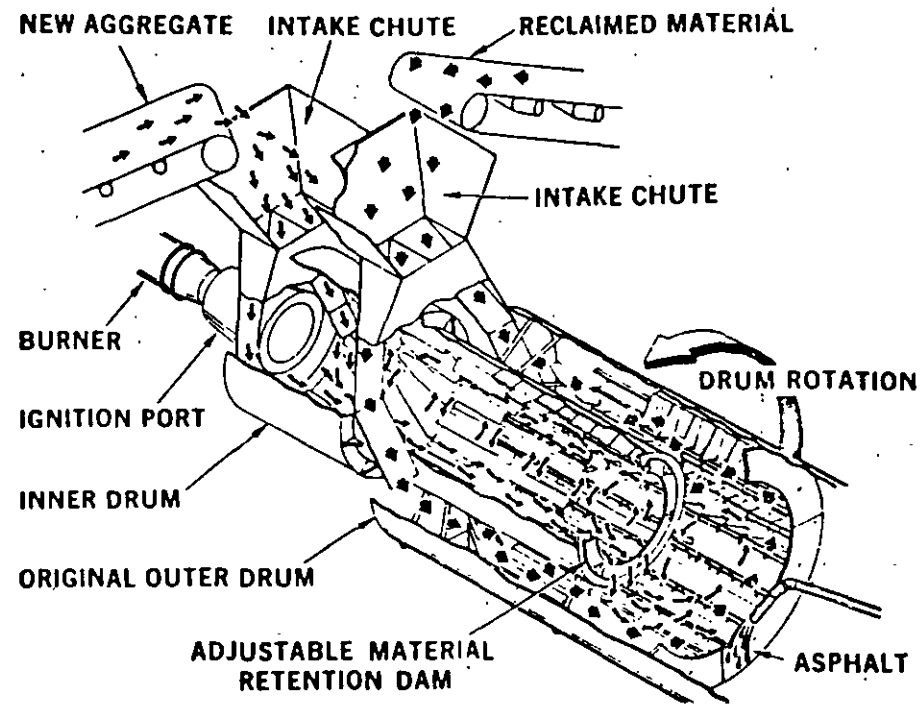
Figure VI-4—Drum plant, drum-in-a-drum (courtesy of Iowa Manufacturing Company).
