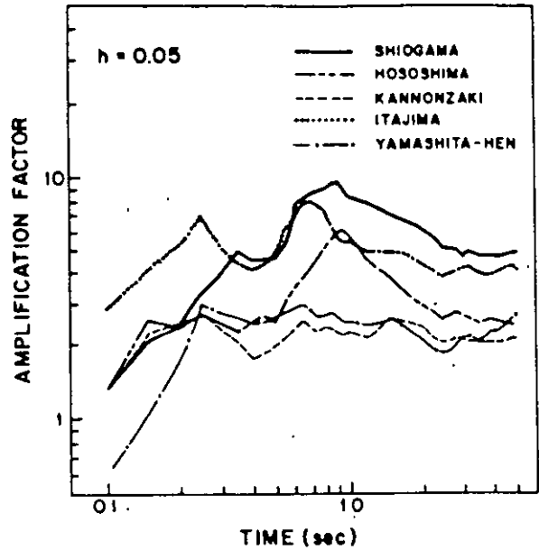
VELOCITY RESPONSE SPECTRA (HORIZONTAL)
