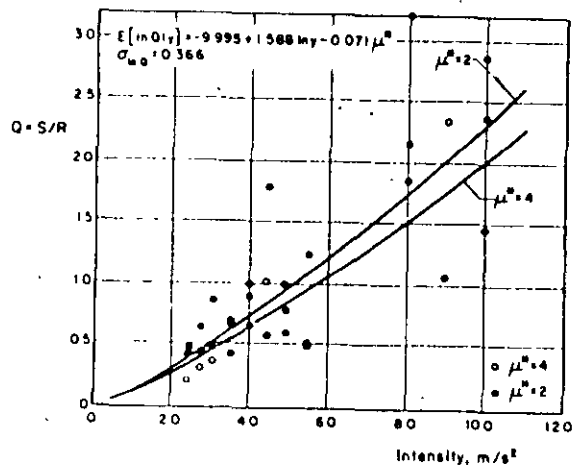
FIG. 10. Normalized Response of Three-Story Frames ( T = 0.85 s, \mu^* = 2 and V_\mu = 0.3 ) Low Spatial Correlation
