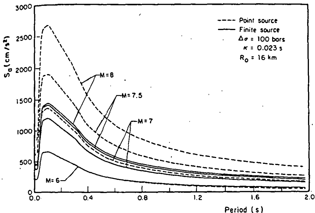
FIG. 10. Predicted response spectra, S_d ( \text{cm/sec}^2 ), 5 per cent damping, for M = 6, 7, 7.5 , and 8 at hard-rock sites in Acapulco ( \Delta\sigma = 100 bars, \kappa = 0.023 sec and R_0 = 16 km). Note that finite-source response spectra reaches a saturation for M \geq 7.5 .
