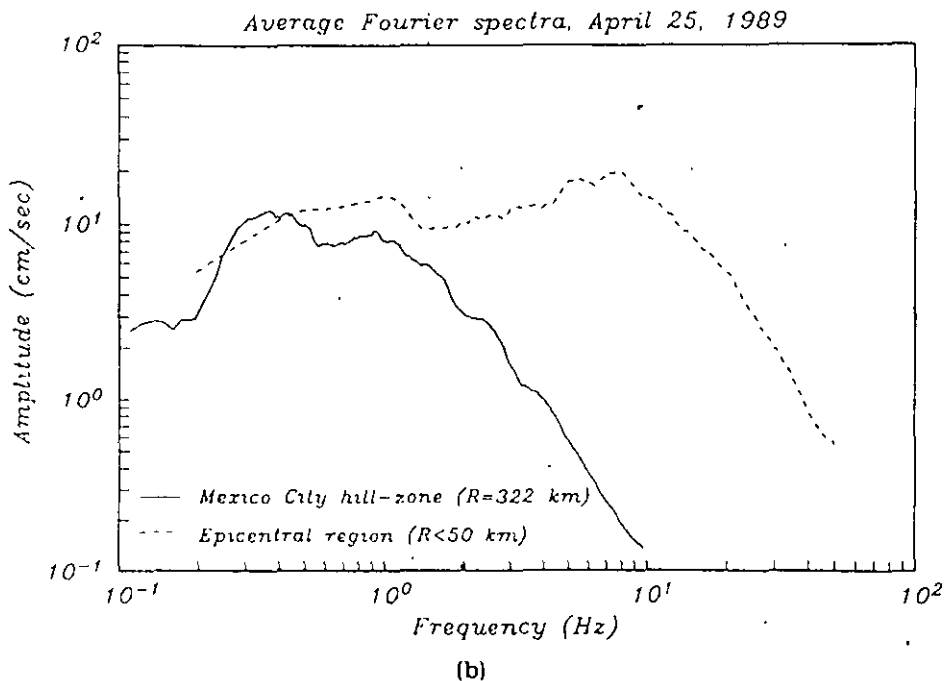
FIG. 2. Comparison of average Fourier amplitude spectra in the epicentral zone (dashed line) and in the hill zone of Mexico City. (a) 19 September 1985 ( M_s = 8.1 ) earthquake. Epicentral recordings from Caleta de Campos, Villita, and La Unión (Fig. 3); hill-zone recordings from CUI and TAC (Fig. 1). (b) 25 April 1989 ( M_s = 6.9 ) earthquake. Epicentral recordings from San Marcos, Cerro de Piedra, Las Vigas, and Las Mesas; hill-zone recordings from CUI, TAC, BS34, and BS74. Note that the epicentral and hill-zone spectral levels are nearly equal between 0.2 and 1 Hz.
