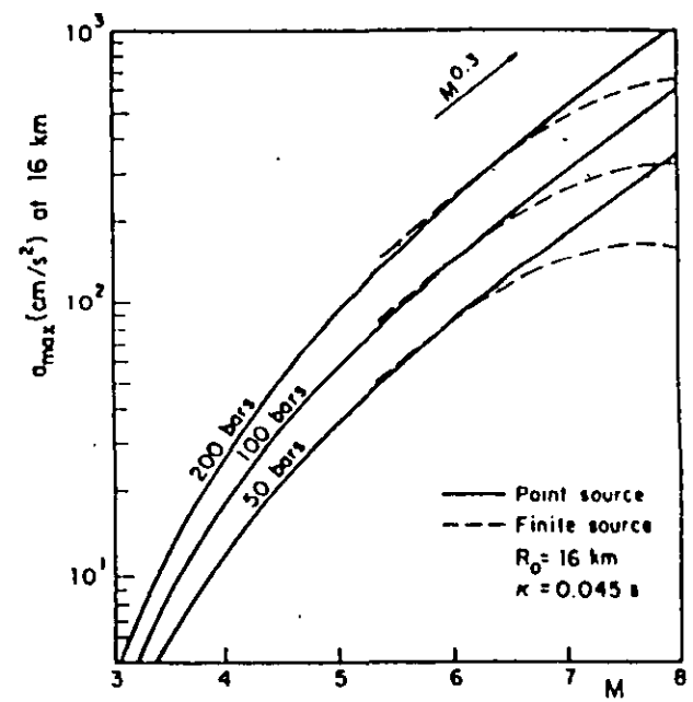
FIG. 5. Expected a_{max} curves as a function of M for a site at 16 km with \Delta\sigma values of 50, 100, and 200 bars and \kappa = 0.023 sec and 0.045 sec. Note that beyond M \approx 6 the point source model overestimates a_{max} with respect to the finite-source model (which predicts almost no dependence of a_{max} on M for M \geq 7.5 ).
