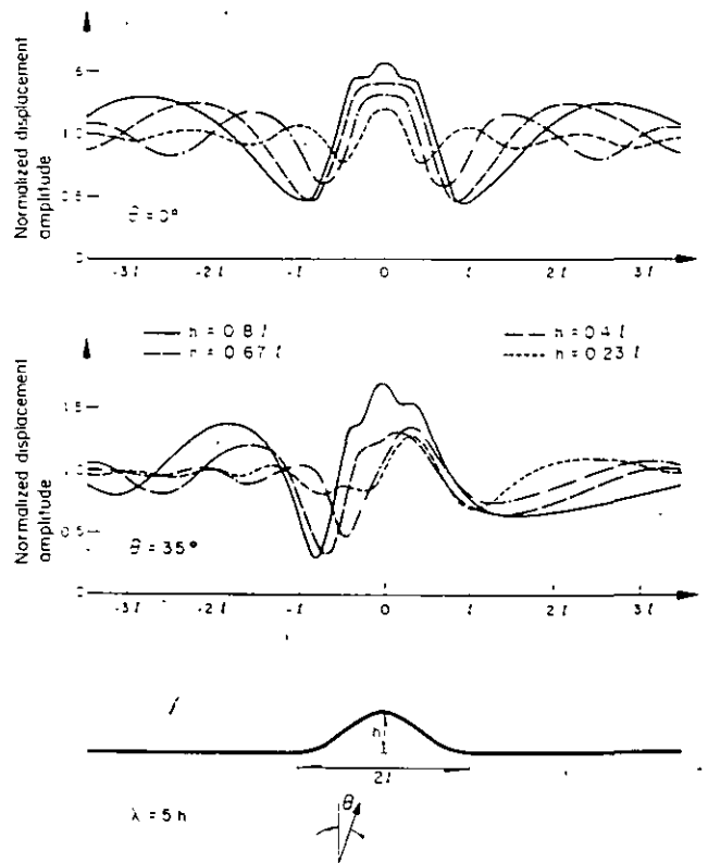
Fig. 6. Normalized displacement amplitudes in surface of a ridge under incident SH waves. (After Bouchon, 1973)
