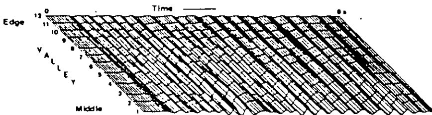
Fig. 35. Two-dimensional anti-plane shear resonance across Chusal Valley. (Top) Observed space-time response of Chusal Valley. The 12 NS component seismograms were recorded during a very small local event on October 12, 1977, located 3 km south of Chusal at a depth of 6 km. These records have been band-passed between 1.5 and 4.5 Hz in order to
