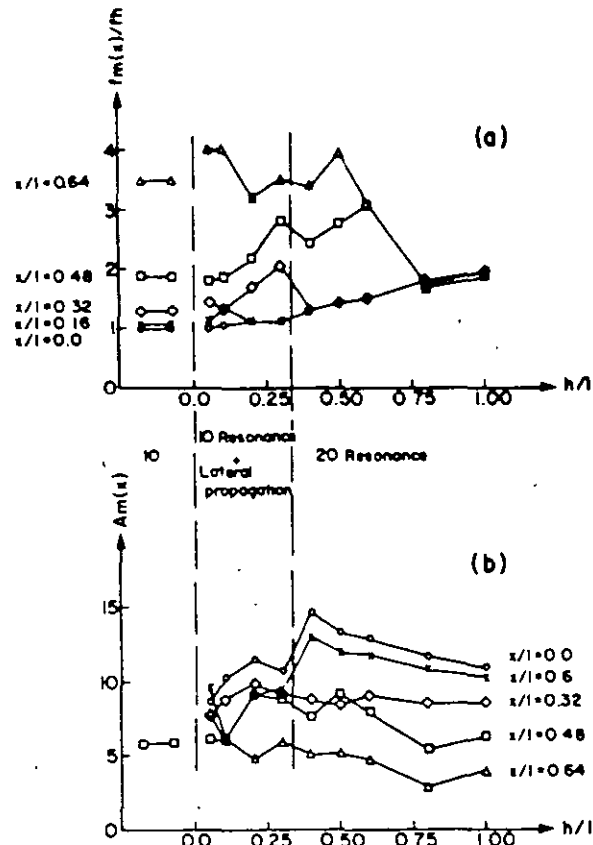
Fig. 30. Peak frequency and the corresponding amplification factor at several horizontal locations x within the sediment as a function of the shape ratio. ( h/l ). (Reproduced from Bard and Bouchon (1985).)
