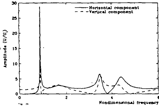
Fig. 24. The amplification factor due to a surface layer for SV waves incident at 45°. The solid line for horizontal and the broken line for vertical component. (Recalculated using parameters in Burridge et al. (1980).)
