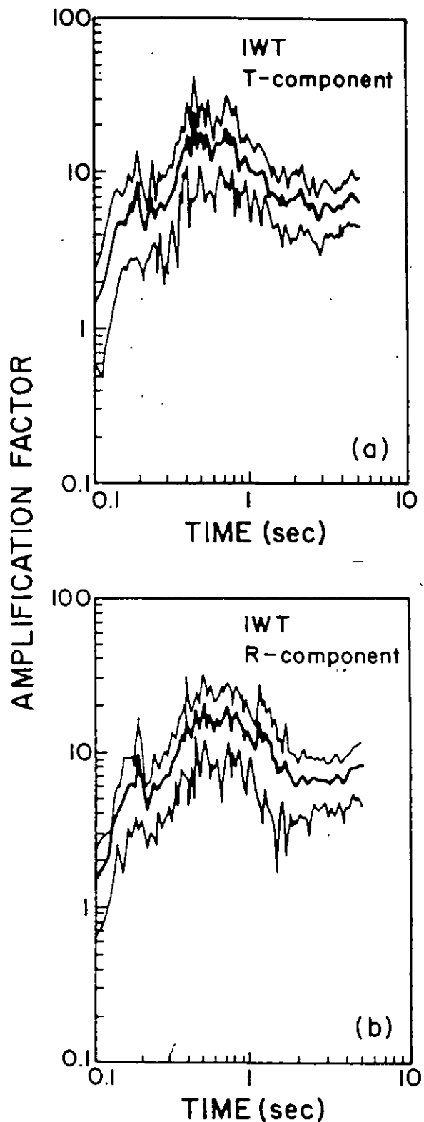
Fig. 5. Amplification factor for the surface site relative to the borehole bottom in the basement rock with the range of one standard error for station IWT. (a) transverse component; (b) radial component. (Reproduced from Kinoshita et al. (1986).)
