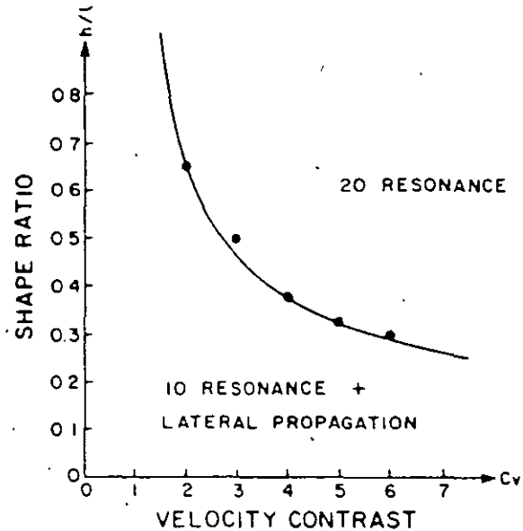
Fig. 29. The critical shape ratio for the 2-D resonance as a function of the velocity contrast between the sediment and basement for incident SH waves. (Reproduced from Bard and Bouchon (1985).)
