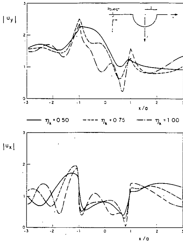
Fig. 11. Amplitudes of vertical and horizontal displacements at the free-surface Semicircular canyon Incidence of Rayleigh waves with normalized frequencies \eta_k=0.5, 0.75, 1.0 (Poisson ratio 0.33)
