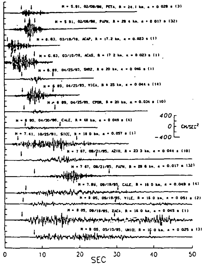
FIG. 2. Near-source, NS component accelerograms of all M \geq 5.9 events recorded above the Mexican subduction zone. R = closest distance to the rupture area. The number in brackets following a value refers to number of events used in its estimation. Arrows indicate rupture duration, T_r . CALE recording of 19 September 1985 is of the first subevent. Arrows at VILE and ZACA correspond to T_r of the first subevent. Note that the records show no dependence of a_{max} on M .
