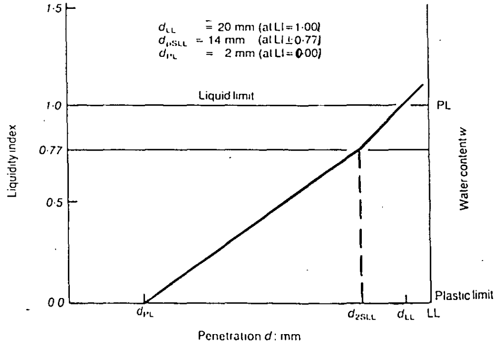
Fig. 3. Relationship between liquidity index, water content and penetration
