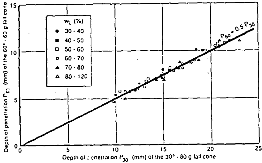
Fig. 1. Relationship between the depths of penetration of the 60° - 60 g and 30° - 80 g fall cones.
