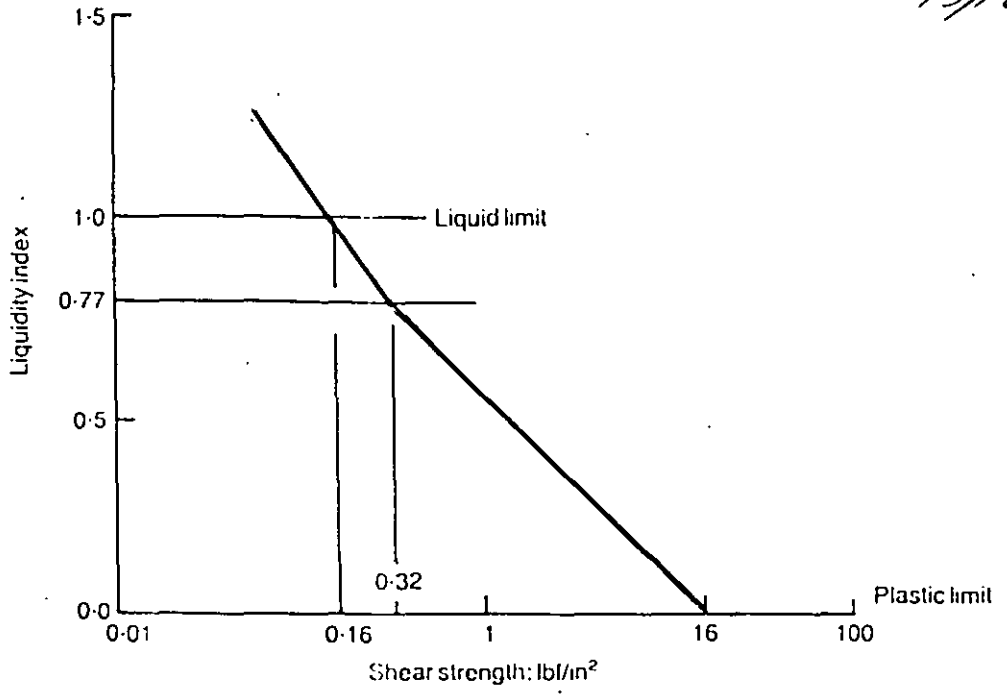
Fig. 2. Idealization of relationship between liquidity index and shear strength
