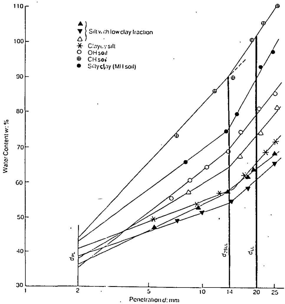
Fig. 4. Experimental results of the relationship between water content and penetration
