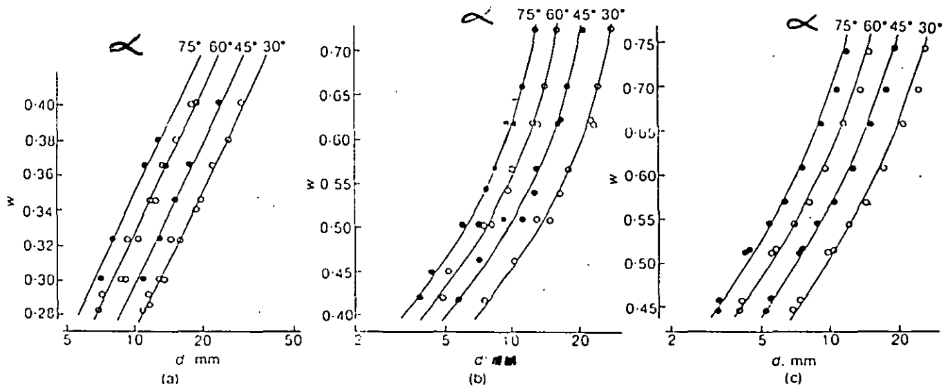
Fig. 2. Variation in penetration d with water content w for cones of weight 100 gf with angles 30°, 45°, 60° and 75°: (a) Drammen Clay; (b) speswhite kaolin; (c) Cambridge Gault Clay
