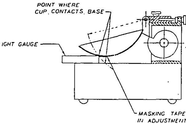
FIG. 4 Calibration for Height of Drop
