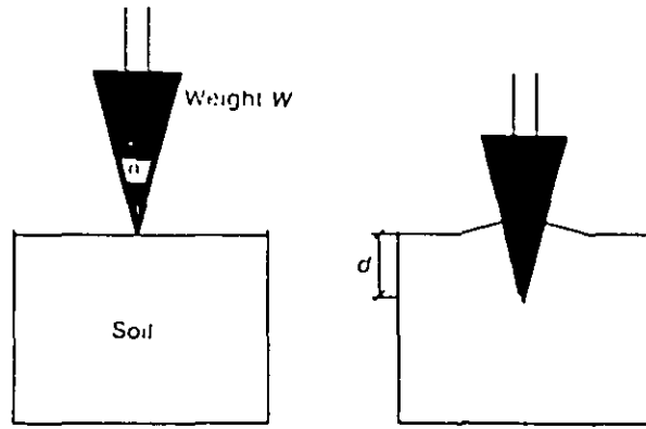
Fig. 1. Diagram of fall-cone test
