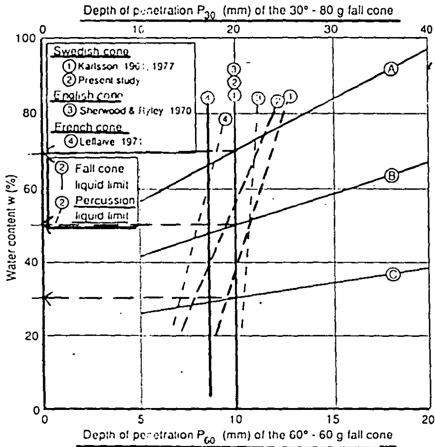
Fig. 5. Liquid limits determined by different fall cone and percussion methods
