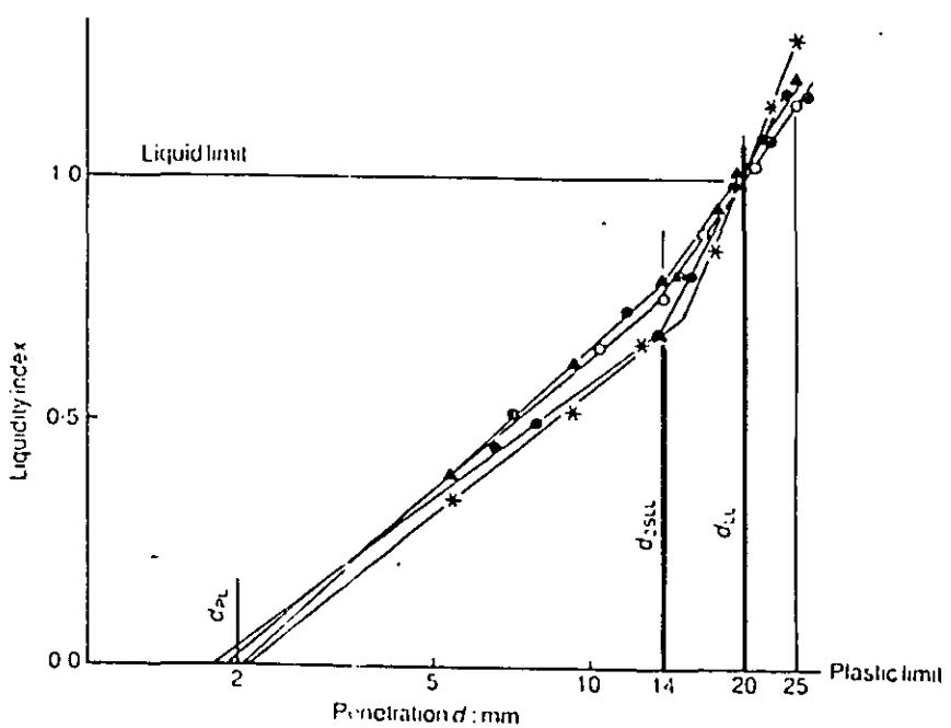
Fig. 5. Experimental results of the relationship between liquidity index and penetration
