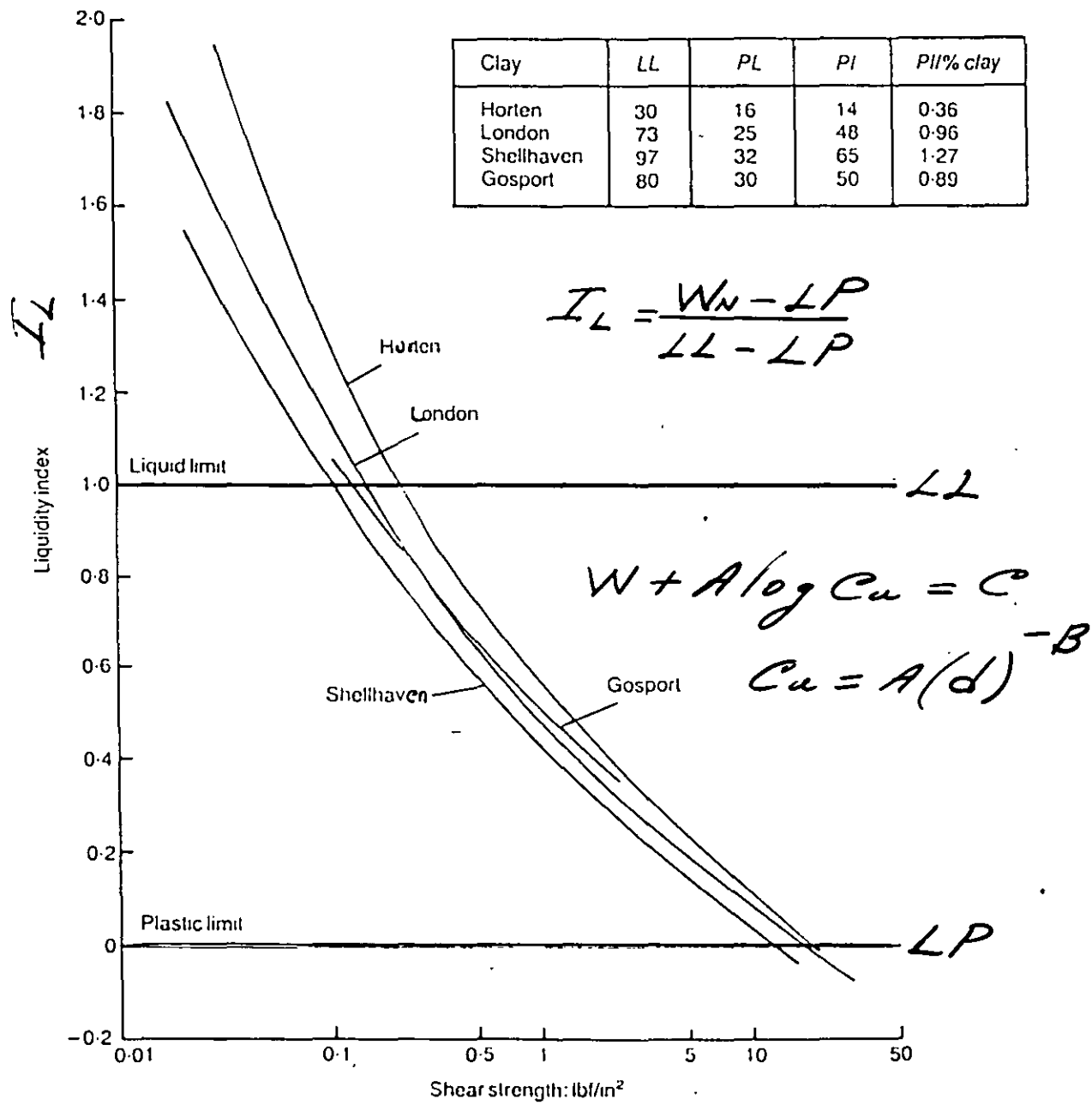
Fig. 1. Relationship between shear strength and liquidity index of remoulded clays (after Skempton & Northey, 1953)
