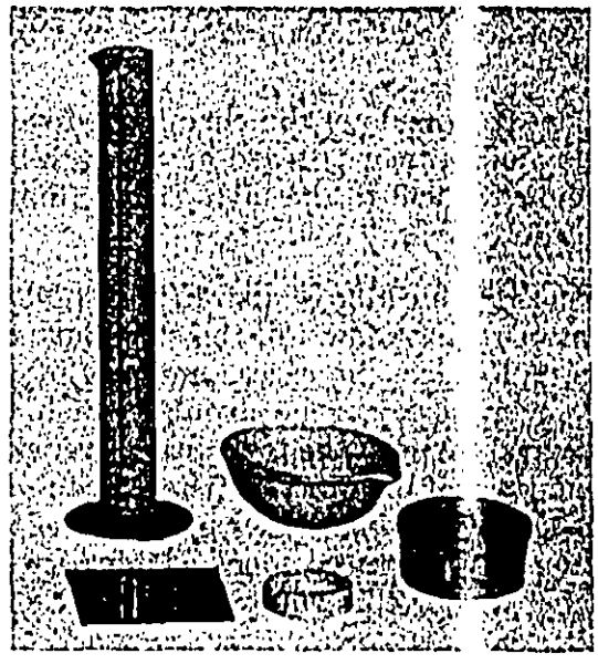
FIGURE 8-2 Apparatus for Determining Shrinkage Limit (Courtesy of Soiltest, Inc.)
