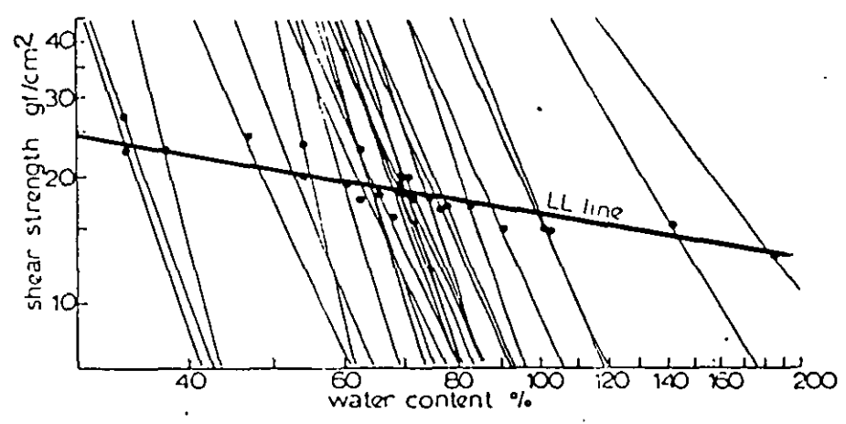
FIG. 2. Relation between water content and shear strength. Each line represents a different soil. The solid points indicate the shear strengths at the liquid limit (after Youssef et al. 1965).
