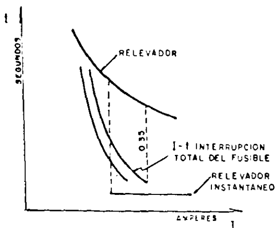
Fig.17 COORDINACION INTERRUPTOR-FUSIBLE
