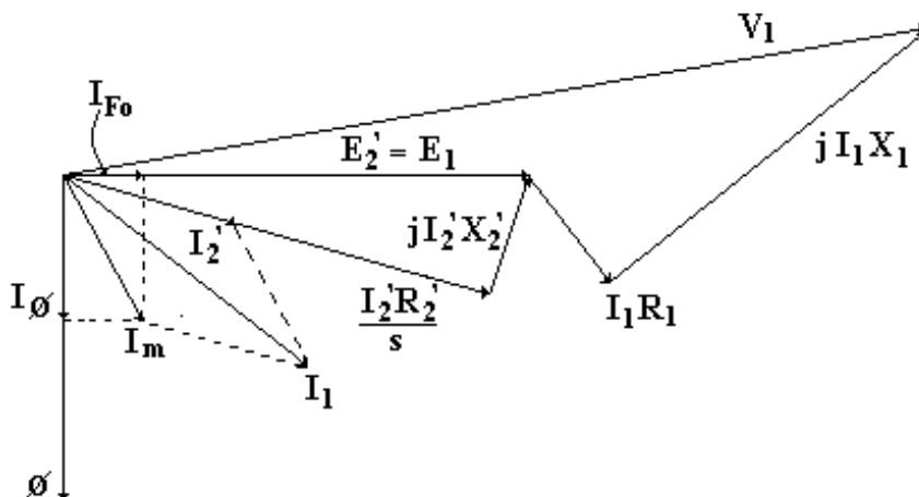
Figura 3.7 Diagrama fasorial
