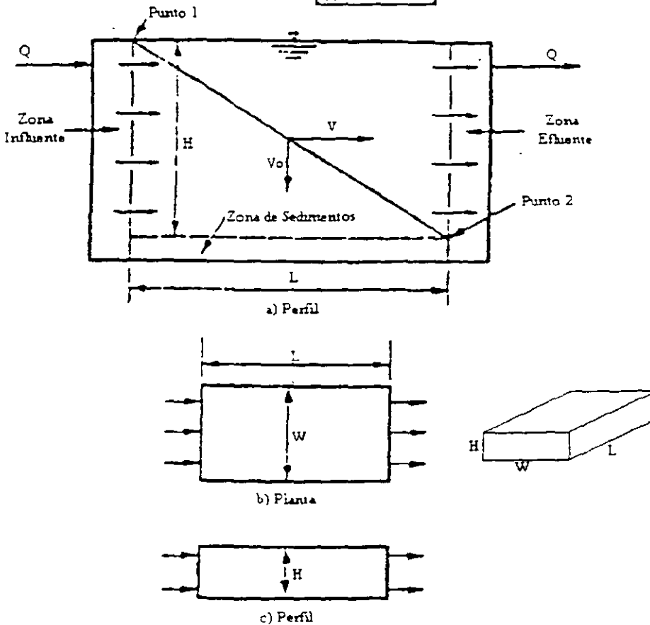
Figura 7.4 Tanque rectangular ideal
