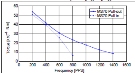
PM20S-020 UNI-CONST. V (at 12[V],50[Ω])
