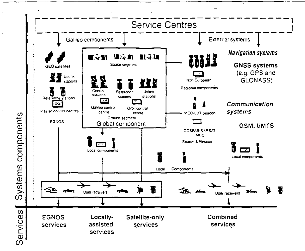
The Galileo system components mapped to services
