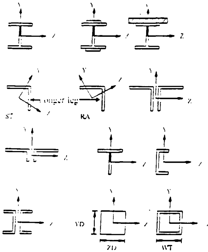
Local axes for different cross-sections
