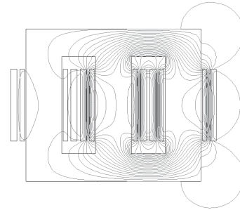
Fig. 6. Distribution of magnetic flux ( \omega t = 0 ) for the short-circuit condition.
