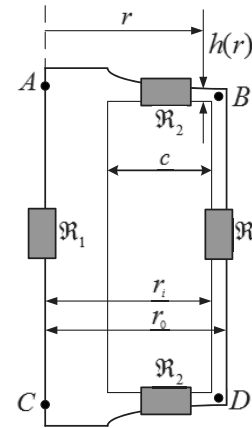
Fig. 3. Reluctance-network of the axisymmetric model.
