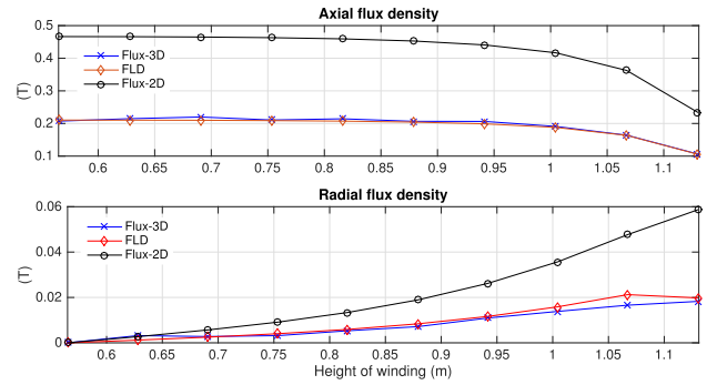
Fig. 7. Flux density components versus height: short-circuit condition.
