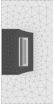
Fig. 5. Geometry and mesh of the 5 kVA axisymmetric transformer.
