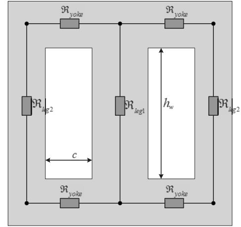
Fig. 2. Reluctance-network of the shell-type core transformer.
