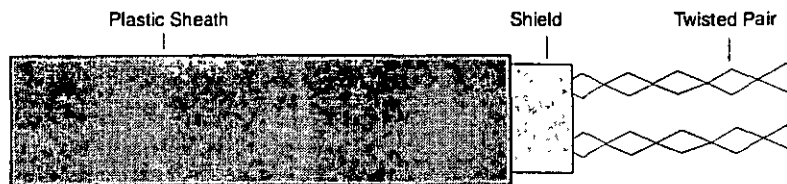
Figure 4-2. Shielded Twisted Pair Cable
