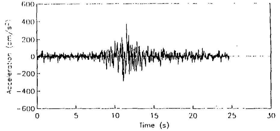
Simulated accelerogram 3
